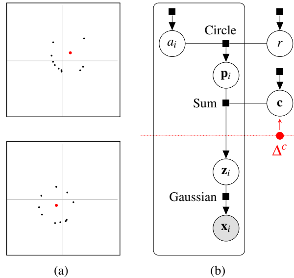
Figure 4.2: The circle problem. (a) Given a sample of points on a circle (black), we wish to infer the circle’s center (red) and its radius. Two sets of samples are shown. (b) The graphical model for this problem.
