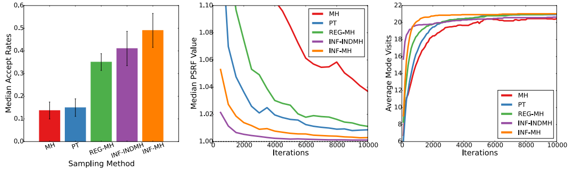
Figure 3.3: Results of the ‘Estimating Camera Extrinsic’ experiment. Acceptance Rates (left), PSRFs (middle), and average number of modes visited (right) for different sampling methods. We plot the median/average statistics over 30 test examples.
