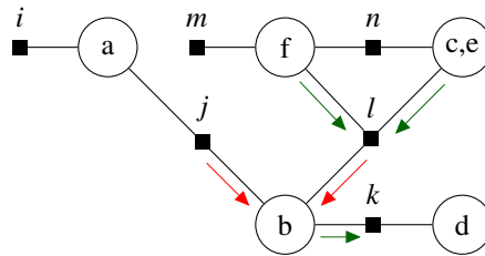
Figure 2.3: An example factor graph. Variable nodes (circles) and factor nodes (squares) representing the factorized function P(a, b, c, d, e, f) = \psi_i(a)\psi_j(a, b)\psi_k(b, d)\psi_l(b, c, e, f)\psi_m(f)\psi_n(c, e, f) . Also shown are sample variable-to-factor messages (green arrows) and, factor-to-variable messages (red arrows).
