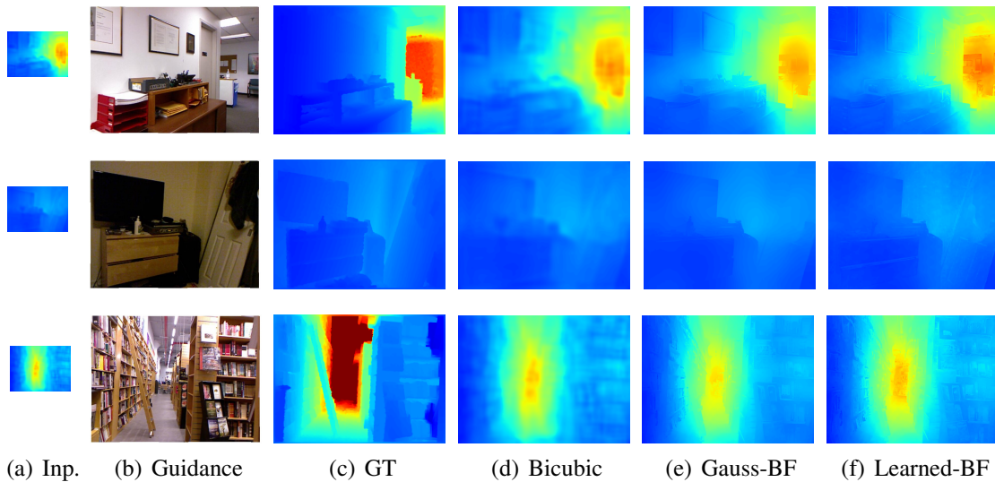
Figure A.12: Depth Upsampling. Depth 8\times upsampling results using different upsampling strategies, from left to right, (a) Low-resolution input depth image (Inp.), (b) High-resolution guidance image, (c) Ground-truth depth; Upsampled depth images with (d) Bicubic interpolation, (e) Gauss bilateral upsampling and, (f) Learned bilateral updowngling (best viewed on screen).
