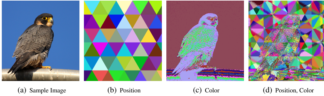
Figure 5.2: Visualization of the permutohedral lattice. (a) Input image; Lattice visualizations for different feature spaces: (b) 2D position features: 0.01(x,y) , (c) color features: 0.01(r,g,b) and (d) position and color features: 0.01(x,y,r,g,b) . All pixels falling in the same simplex cell are shown with the same color.
