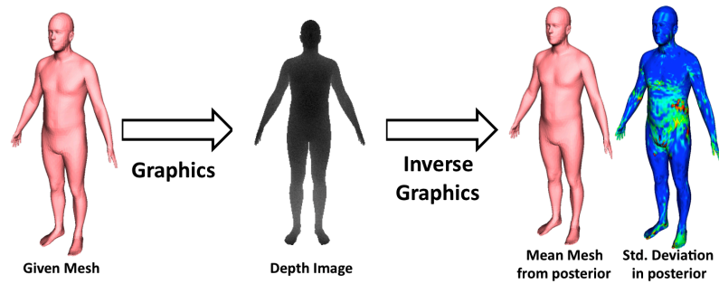
Figure 3.1: An example ‘inverse graphics’ problem. A graphics engine renders a 3D body mesh and a depth image using an artificial camera. By ‘Inverse Graphics’, we refer to the process of estimating the posterior probability over possible bodies given the depth image.
