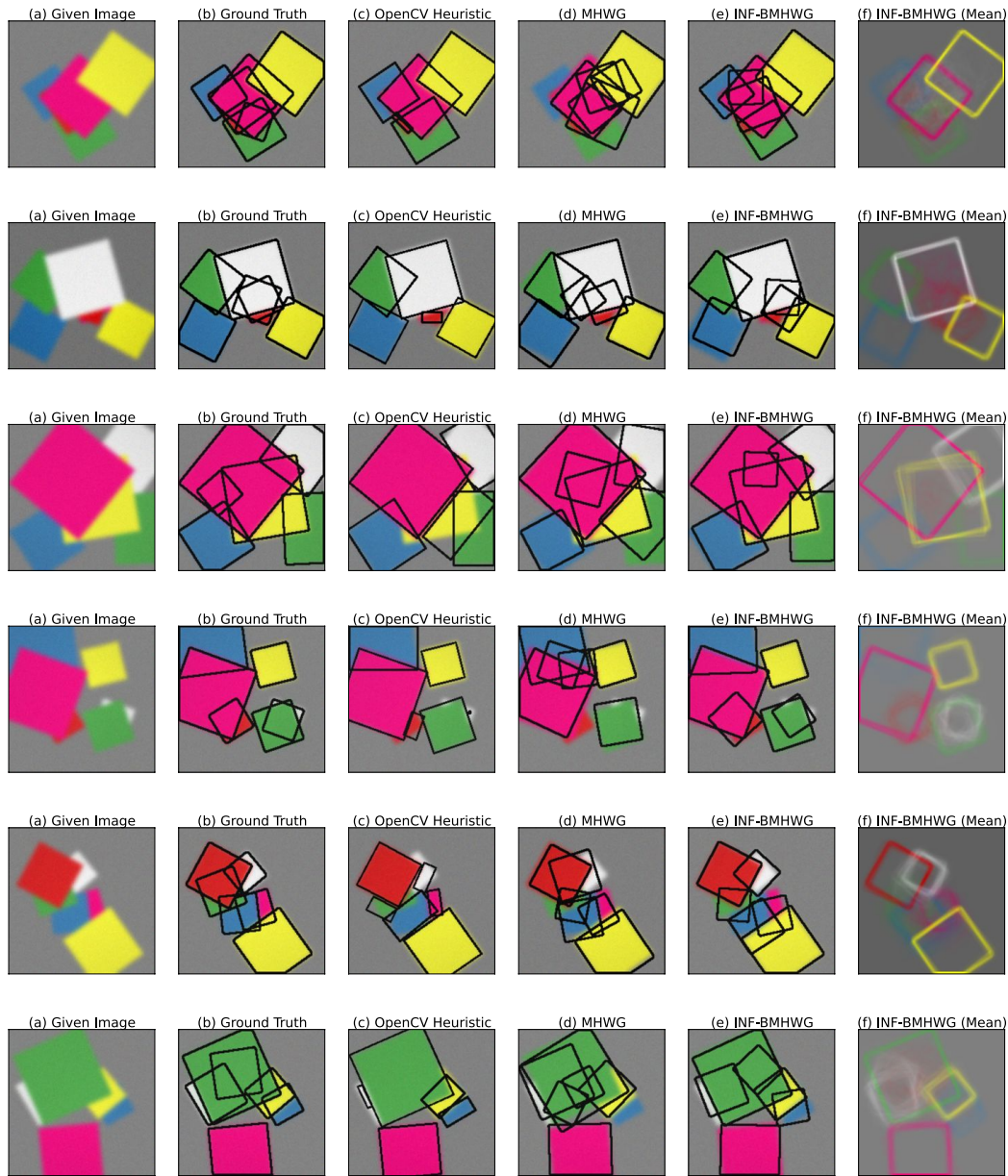
Figure A.5: Additional qualitative results of the occluding tiles experiment. From left to right: (a) Given image, (b) Ground truth tiles, (c) OpenCV heuristic and most probable estimates from 5000 samples obtained by (d) MHWG sampler (best baseline) and (e) our INF-BMHWG sampler. (f) Posterior expectation of the tiles boundaries obtained by INF-BMHWG sampling (First 2000 samples are discarded as burn-in).
