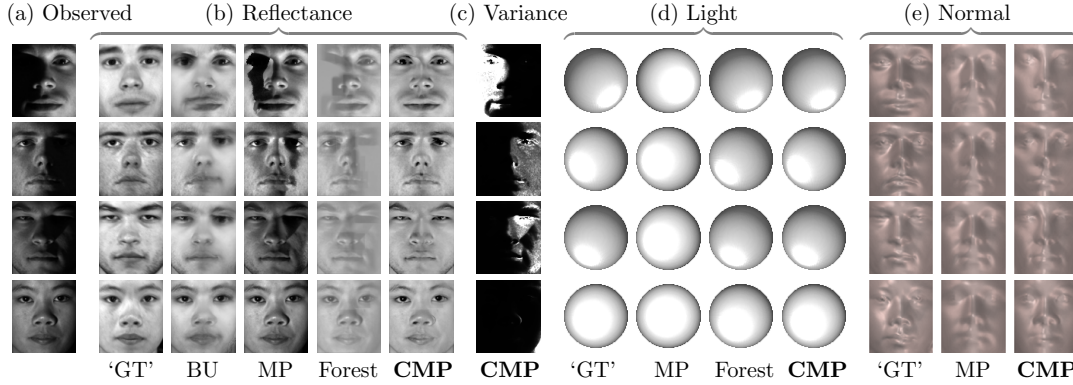
Figure 4.7: A visual comparison of inference results for the face problem. For 4 randomly chosen test images, we show inference results obtained by competing methods. (a) Observed images. (b) Inferred reflectance maps. GT is the stereo estimate which we use as a proxy for ground-truth, BU is the bottom-up reflectance estimate of Biswas et al. (2009), MP refers to standard variational message passing, Forest is the consensus prediction and CMP is the proposed consensus message passing technique. (c) The variance of the inferred reflectance estimate produced by CMP (normalized across rows). High variance regions correlate strongly with cast shadows. (d) Visualization of inferred light. (e) Inferred normal maps.
