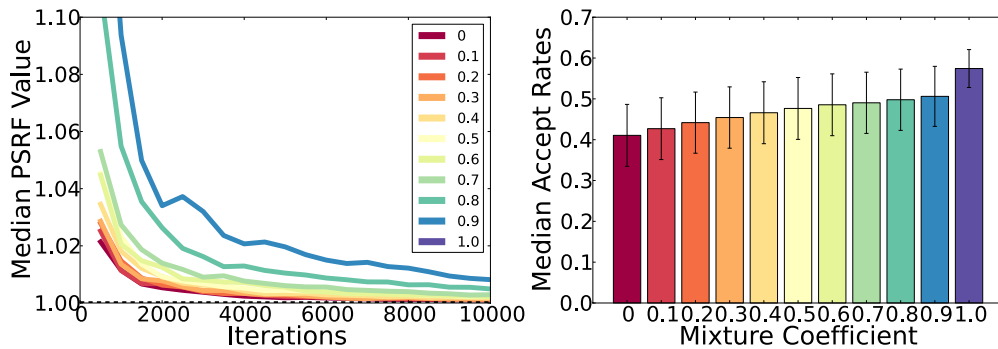
Figure 3.4: Role of mixture coefficient. PRSFs and Acceptance rates corresponding to various mixture coefficients ( \alpha ) of INF-MH sampling in ‘Estimating Camera Extrinsic’ experiment.
