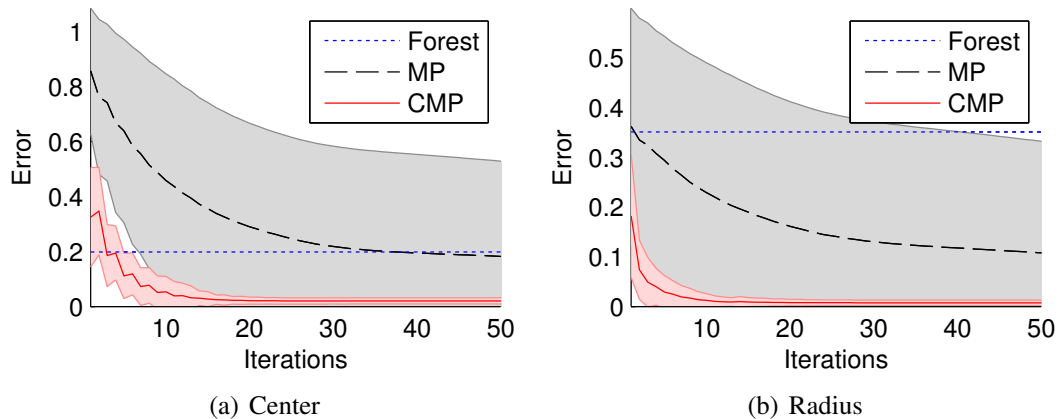
Figure 4.3: Accelerated inference using CMP for the circle problem. (a) Distance of the mean of the marginal posterior of center c from its true value as a function of number of inference iterations (Forest: direct prediction, MP: standard VMP, CMP: VMP with consensus). Consensus message passing significantly accelerates convergence. (b) Similar plot for radius r .
