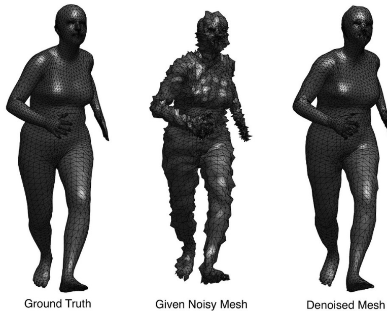
Figure 5.6: Sample denoising result. Ground truth mesh (left), corresponding given noisy mesh (middle) and the denoised result (right) using the learned bilateral filter.
