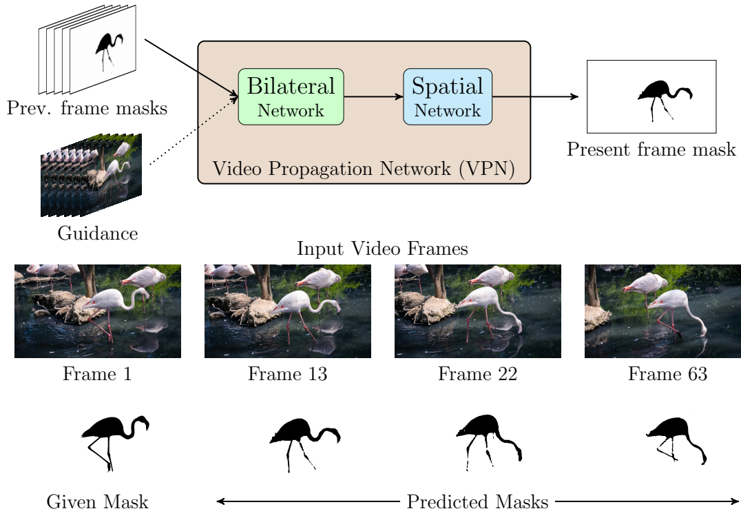
Figure 6.1: Video Propagation with VPNs. The end-to-end trained VPN network is composed of a bilateral network followed by a standard spatial network and can be used for propagating information across frames. Shown here is an example result of foreground mask from the 1 st frame to other video frames.
