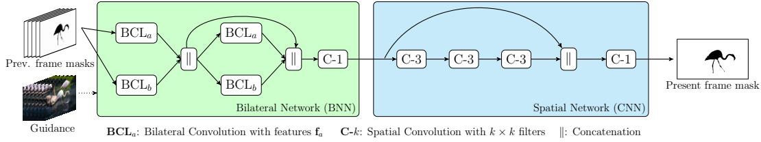
Figure 6.2: Computation Flow of Video Propagation Network. Bilateral networks (BNN) consist of a series of bilateral filterings interleaved with ReLU non-linearities. The filtered information from BNN is then passed into a spatial network (CNN) which refines the features with convolution layers interleaved with ReLU non-linearities, resulting in the prediction for the current frame.
