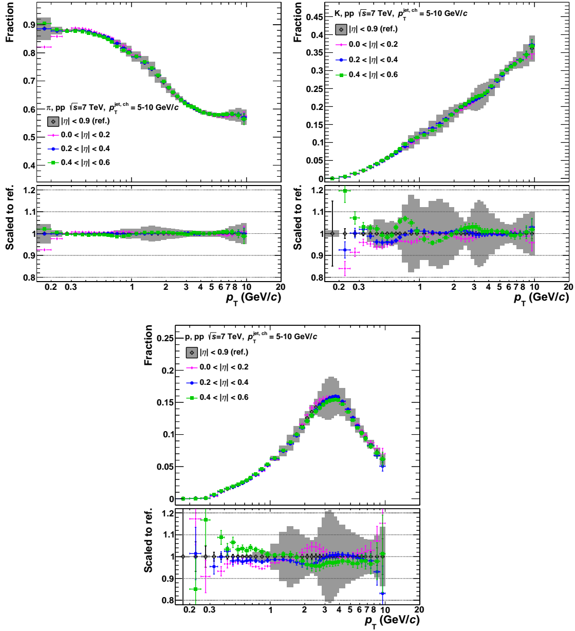
Figure G.2.: Comparison of the uncorrected particle fractions in \eta slices (coloured symbols) and in the full \eta range (black open crosses) versus p_T^{\text{track}} for p_T^{\text{jet}} = 5 - 10 GeV/c in data. The results are shown for (from upper left to lower right) \pi , K and p. The grey area indicates the systematic uncertainties for the full \eta range.
