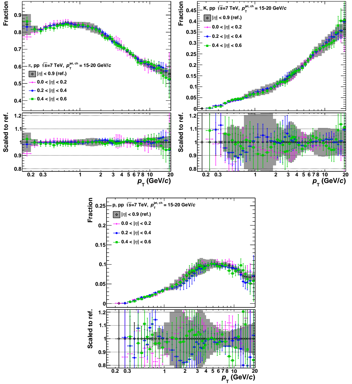
Figure G.3.: Comparison of the uncorrected particle fractions in \eta slices (coloured symbols) and in the full \eta range (black open crosses) versus p_T^{\text{track}} for p_T^{\text{jet}} = 15 - 20 \text{ GeV}/c in data. The results are shown for (from upper left to lower right) \pi , K and p. The grey area indicates the systematic uncertainties for the full \eta range.
