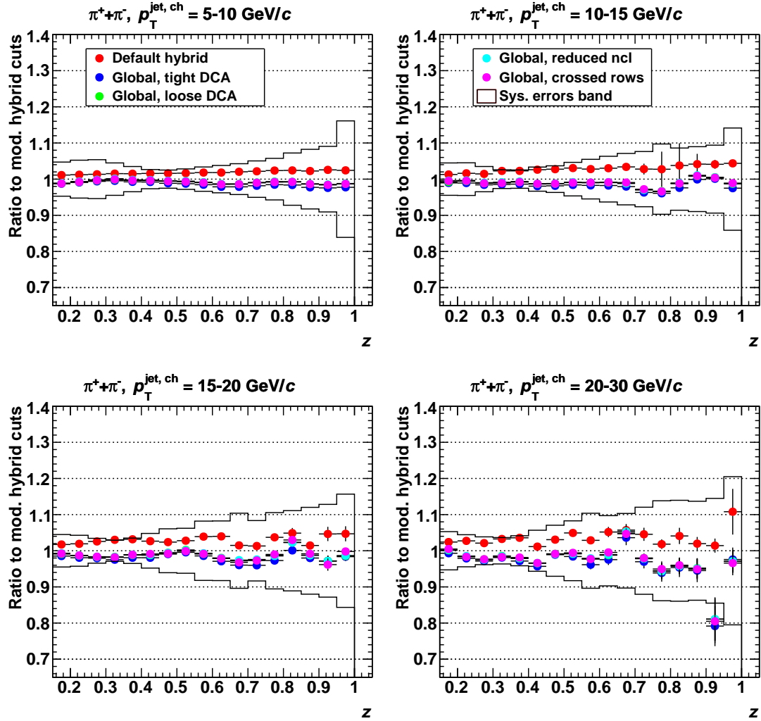
Figure I.4.: Cut variations for pions in jets as a function of z . The ratio to the modified hybrid track cuts is shown. Each set of cuts is corrected with its own MC correction factors. The systematic error band shows the total uncertainty from fit and MC corrections.
