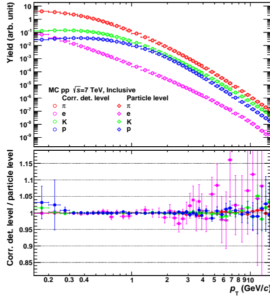
(a) Inclusive
