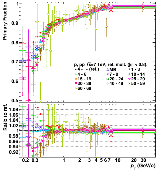
(c) Protons
