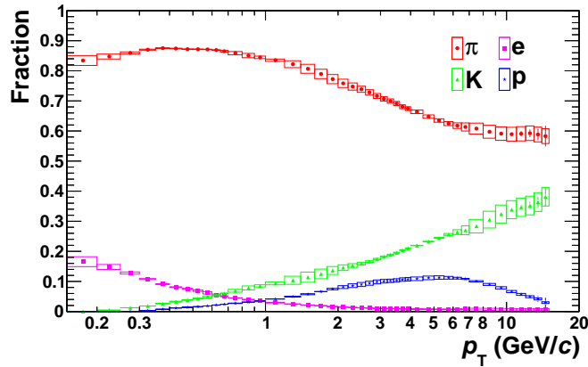
Figure 6.7.: The uncorrected particle fractions are shown for particles in jets with p_T^{\text{jet}} = 10 - 15 \text{ GeV}/c in data. The boxes show the systematic error due to the spline uncertainties.
