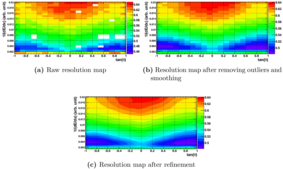
Figure 3.16.: Resolution map obtained from protons. a) shows the raw result from the fits and b) shows the same map after removing outliers and smoothing. In c) , the refined map using interpolation is presented. The colour code shows the relative resolution per cluster, where bins in which the fit failed are shown in white.
