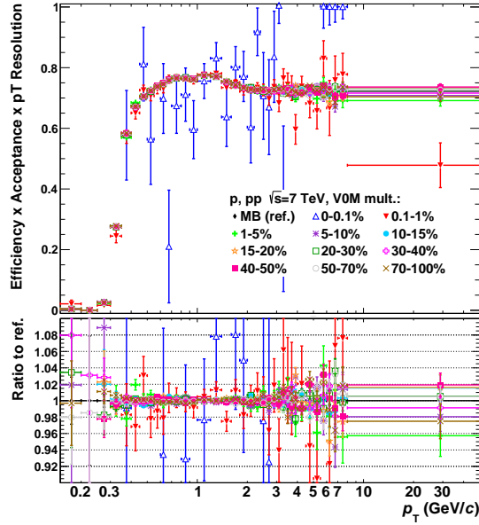
(c) Protons
