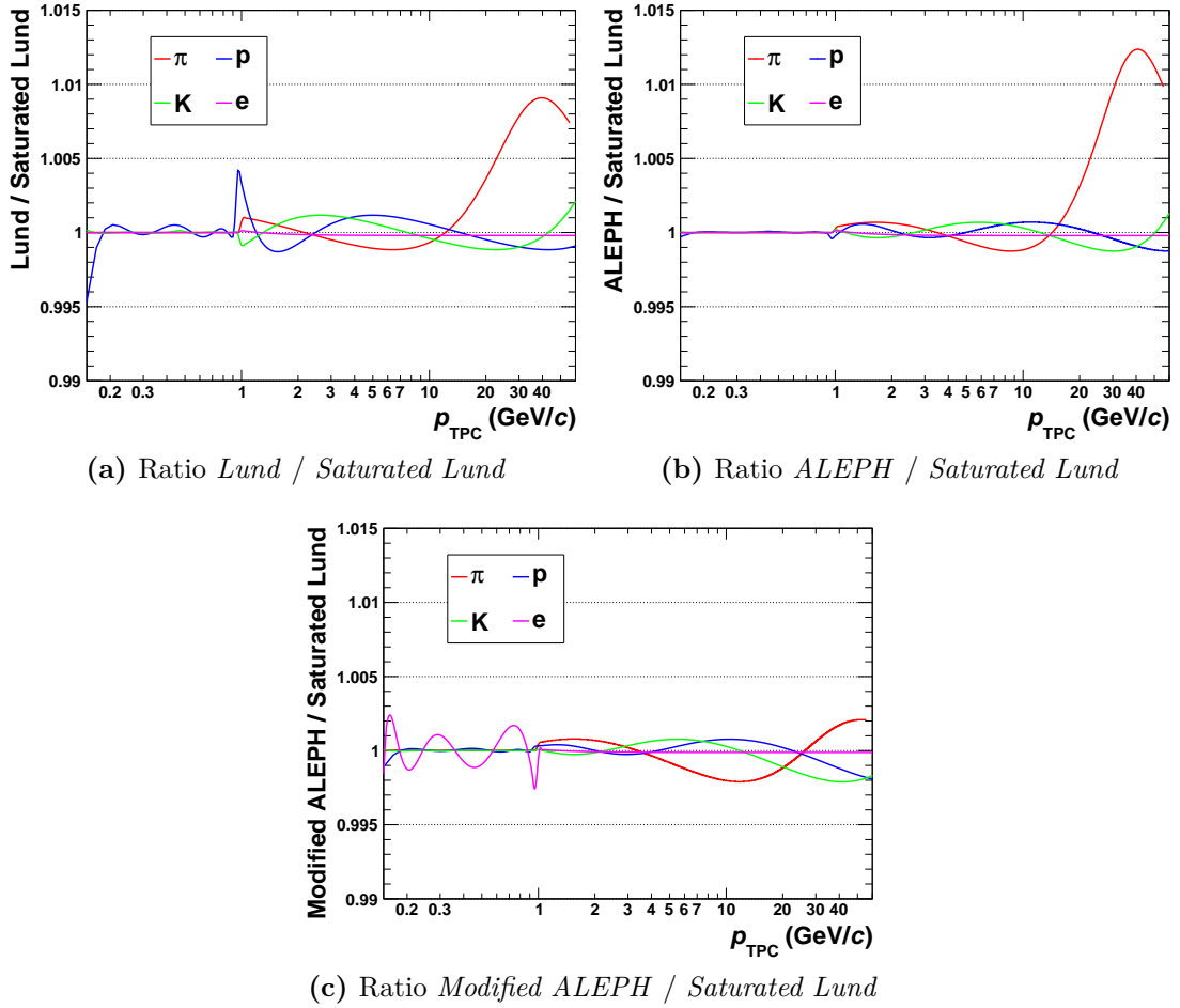
Figure 3.9.: Comparison of a) Lund , b) ALEPH and c) Modified ALEPH Bethe-Bloch parametrisations to the Saturated Lund model. Note that the low-momentum corrections are already included for all parametrisations.
