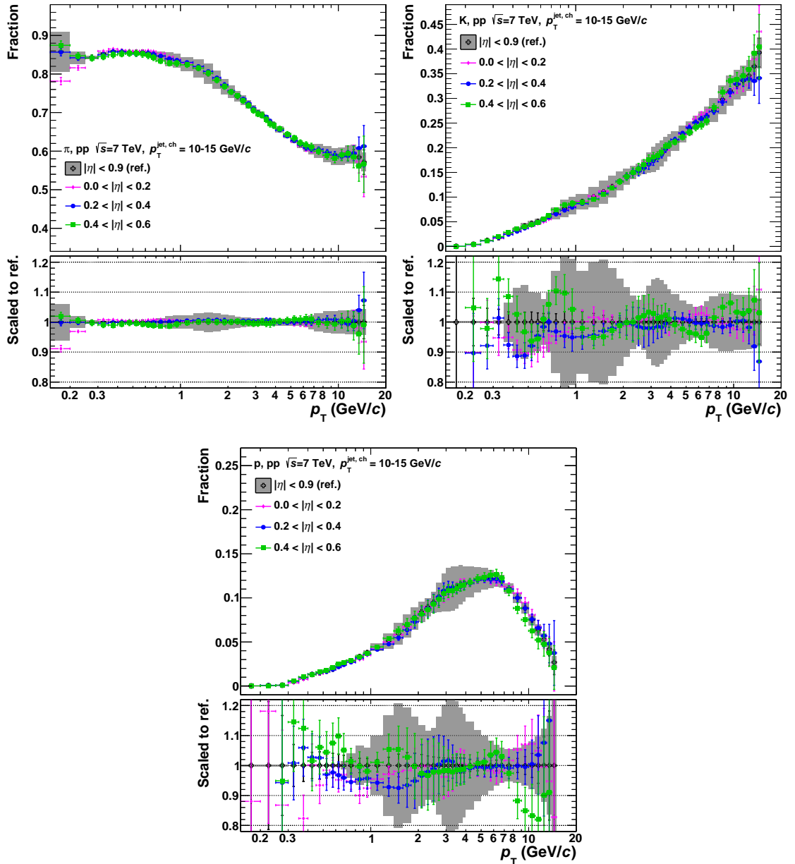
Figure 6.14.: Comparison of the uncorrected particle fractions in \eta slices (coloured symbols) and in the full \eta range (black open crosses) versus p_T^{\text{track}} for p_T^{\text{jet}} = 10 - 15 \text{ GeV}/c in data. The results are shown for (from upper left to lower right) \pi , K and p. The grey area indicates the systematic uncertainties for the full \eta range.
