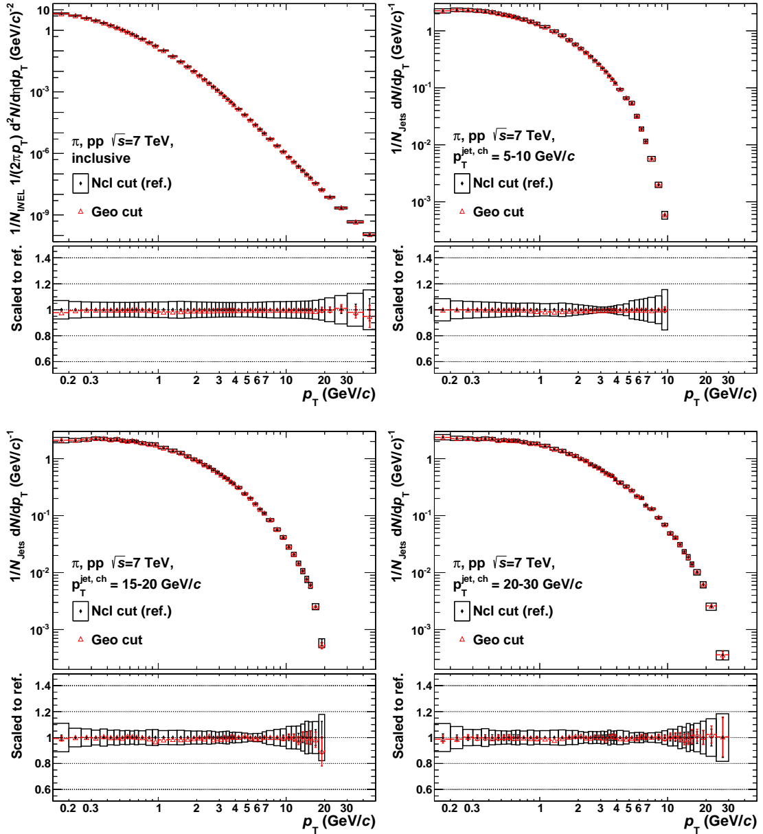
Figure I.1.: Comparison of the corrected pion yields for the TPC geometrical cut (red open triangles) and the ncl cut (black diamonds) versus p_T^{\text{track}} in data. Each set of cuts is corrected with its own MC correction factors. The boxes correspond to the systematic errors for the ncl cut, including the uncertainties of the corresponding MC correction factors.
