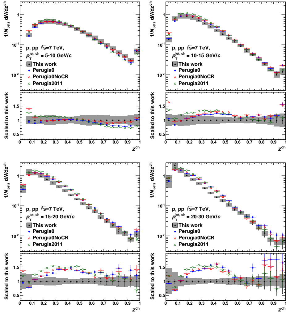
Figure K.9.: Comparison of corrected proton yields in jets to different MC predictions as a function of z . The p_T^{\text{jet}} increases from the upper left to the lower right panel.
