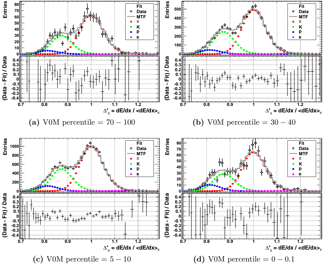
Figure F.5.: Template fits to data for different V0M percentile bins for p_T = 8 - 10 GeV/ c . The V0M percentile decreases from the upper left to the lower right plot.
