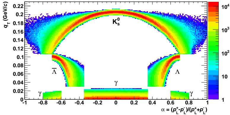
Figure 3.4.: Armenteros-Podolanski plot of V0 mothers of particles used to extract the TPC PID response. The cuts have already been applied (see text). The contributions from K_S^0 , \Lambda , \bar{\Lambda} and \gamma are indicated.
