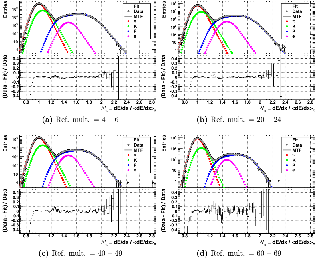
Figure F.1.: Template fits to data for different reference multiplicity bins for p_T = 0.8 - 0.9 \text{ GeV}/c . The multiplicity increases from the upper left to the lower right plot.
