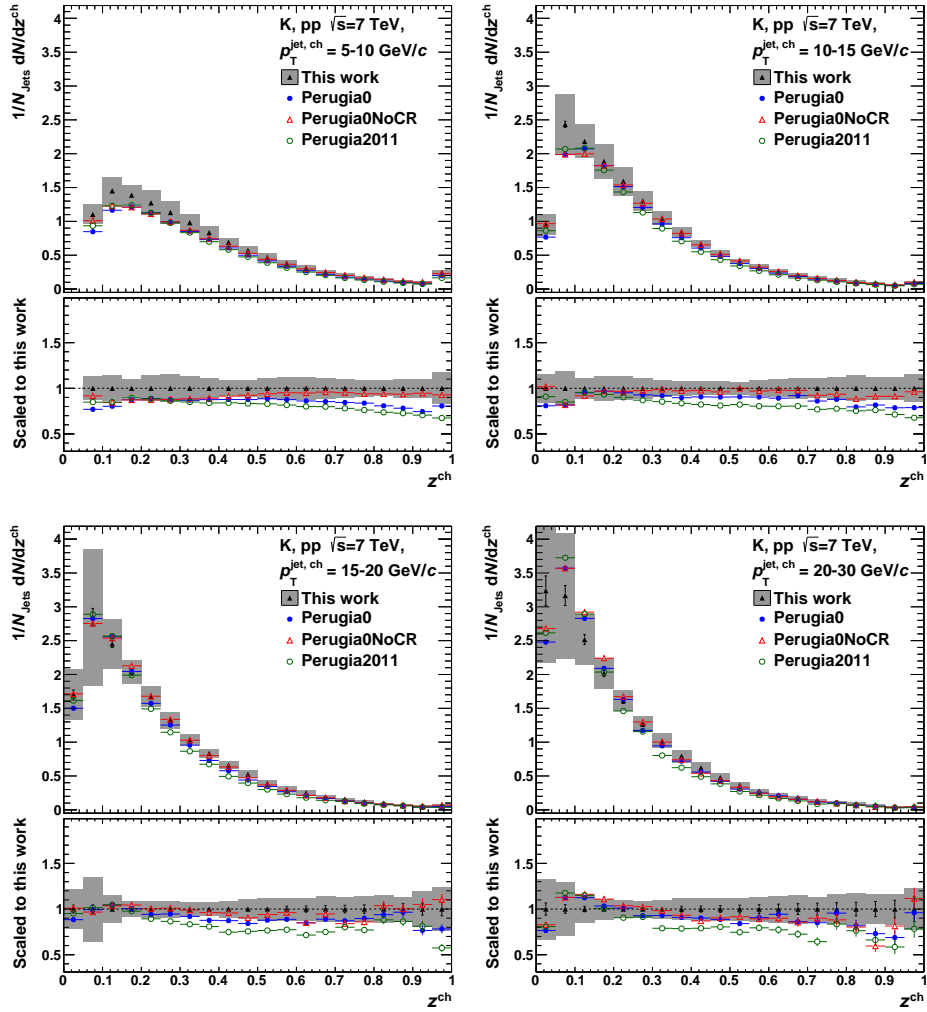
Figure K.2.: Comparison of corrected kaon yields in jets to different MC predictions as a function of z . The p_T^{\text{jet}} increases from the upper left to the lower right panel.
