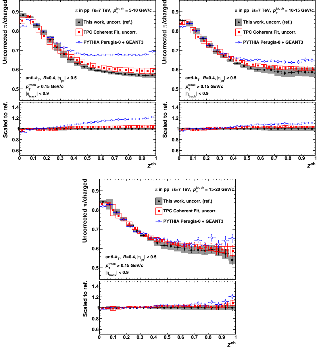
Figure H.1.: Comparison of uncorrected pion fractions as a function of z to the TPC Coherent Fit. In addition, the MC prediction from PYTHIA Perugia-0 is overlaid.
