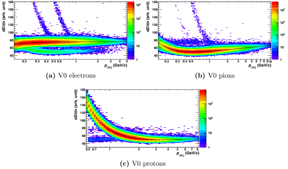
Figure 3.6.: The V0 purity is demonstrated via the dE/dx distributions of the V0 daughters. The black data points indicate the mean of Gauss fits around the peaks.
