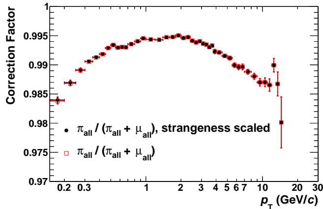
Figure 5.4.: Correction factors for the muon contamination of the pions in jets with p_T^{\text{jet}} = 10 - 15 \text{ GeV}/c . The difference between the correction factors with (black dots) and without (red open boxes) strangeness scaling is negligible.
