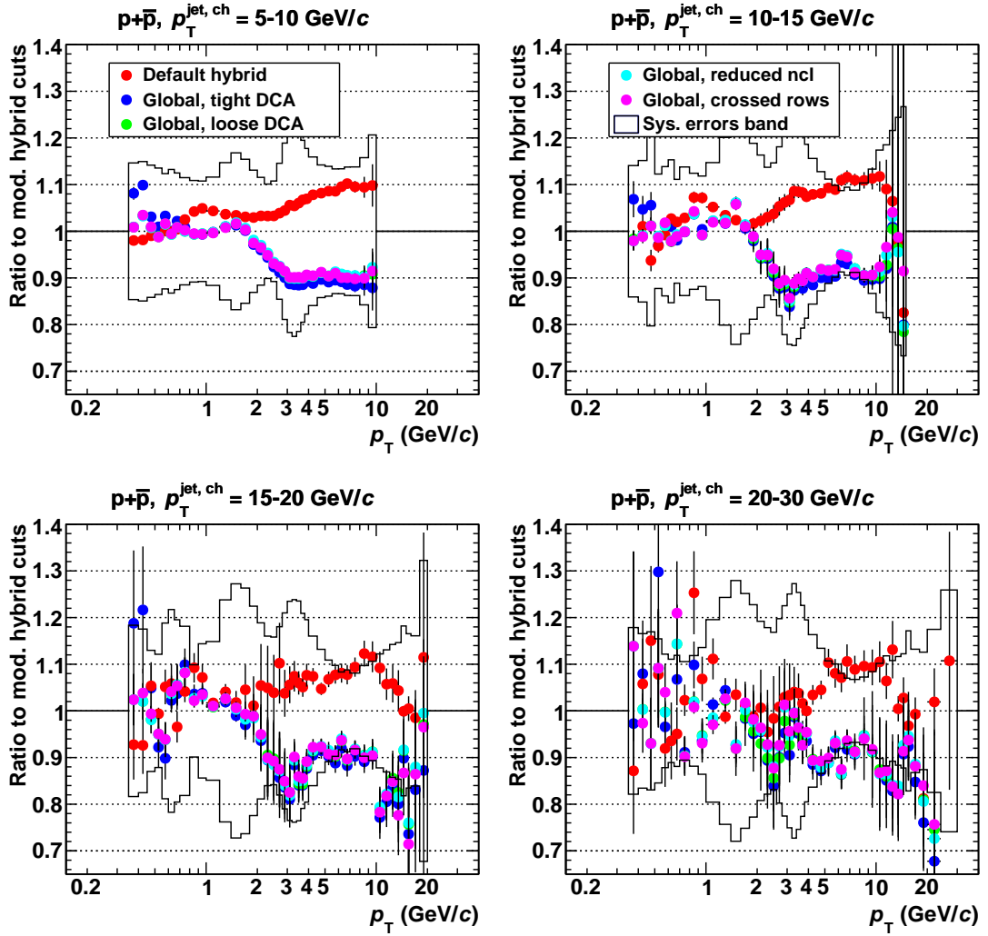
Figure 6.20.: Cut variations for protons in jets. The ratio to the modified hybrid track cuts is shown. Each set of cuts is corrected with its own MC correction factors. The systematic error band shows the total uncertainty from fit and MC corrections.
