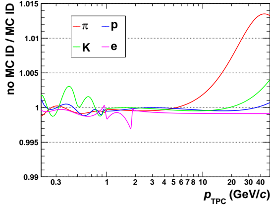
Figure 4.12.: The splines extracted with ( MC ID ) and without ( no MC ID ) MC information are compared. Their ratio is shown as a function of momentum for the individual species. no MC ID indicates that the splines were extracted as in data from V0’s and other clean detector samples (TPC, TPC+TOF). For MC ID , primary particles which are “identified” via the particle level truth have been used.
