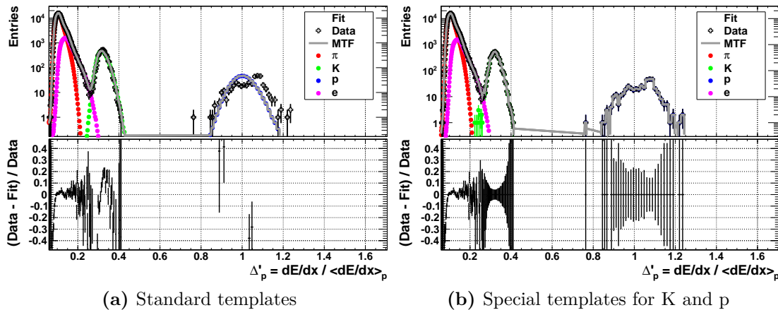
Figure 4.5.: Demonstration of special dE/dx templates: in a) , the default templates for all species have been used, whereas in b) , special templates are used for kaons and protons. The plots are for data and show tracks with p_T^{\text{track}} = 0.25 - 0.30 \text{ GeV}/c in jets with p_T^{\text{jet}} = 5 - 10 \text{ GeV}/c .
