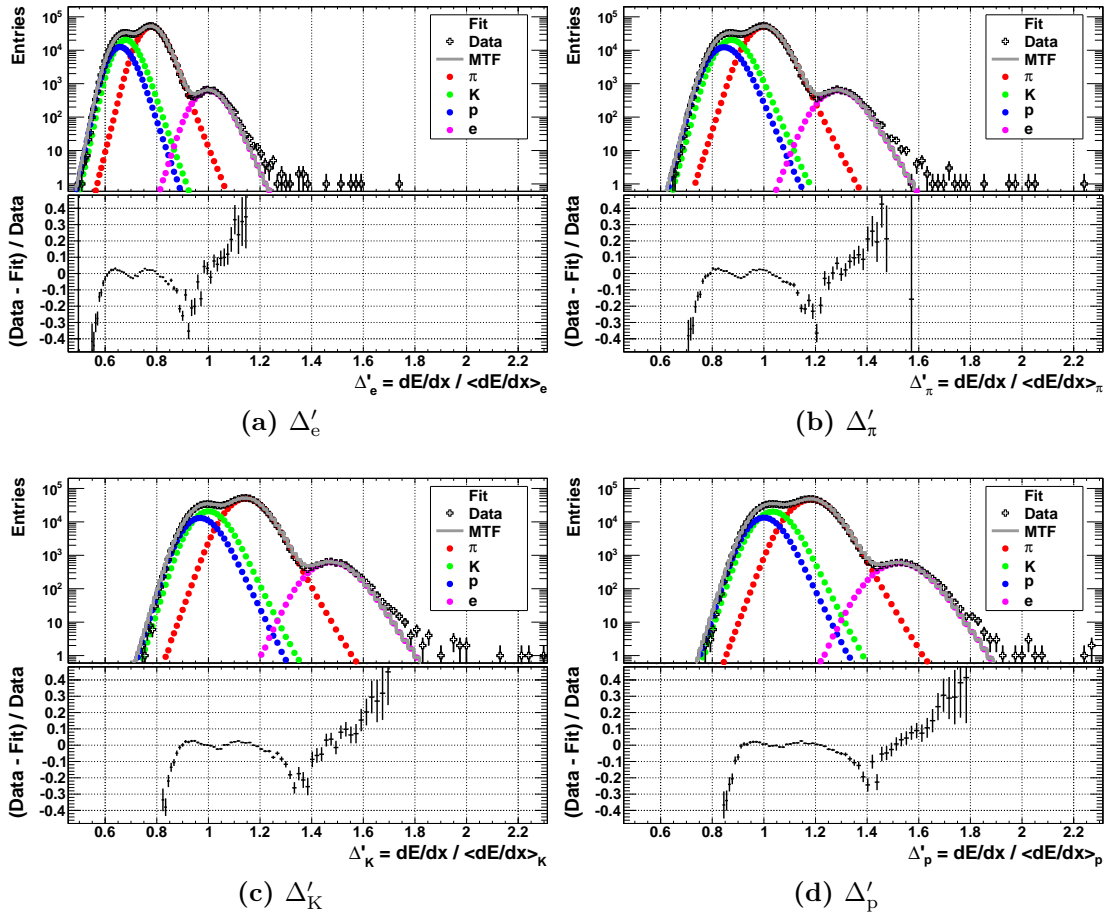
Figure 4.7.: Comparison of template fits to data for different \Delta'_{\text{species}} for the horizontal axis. In the upper panel of each plot, the dE/dx distribution for p_T = 3.0 - 3.2 \text{ GeV}/c is shown in black together with the templates (full points) and the fit (grey line). The lower panels show the relative deviation of the fit from data.
