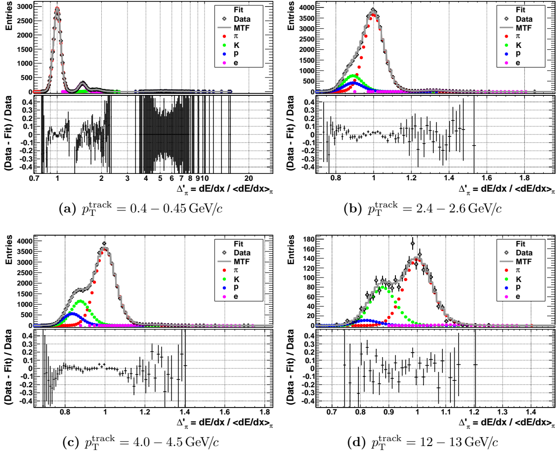
Figure F.6.: Template fits to data in different p_T^{\text{track}} intervals for p_T^{\text{jet}} = 10 - 15 \text{ GeV}/c . The panels a) – d) show the following p_T^{\text{track}} ranges in \text{GeV}/c : 0.4 – 0.45, 2.4 – 2.6, 4.0 – 4.5 and 12 – 13. Note the different ranges of the abscissa and its logarithmic scale in a).
