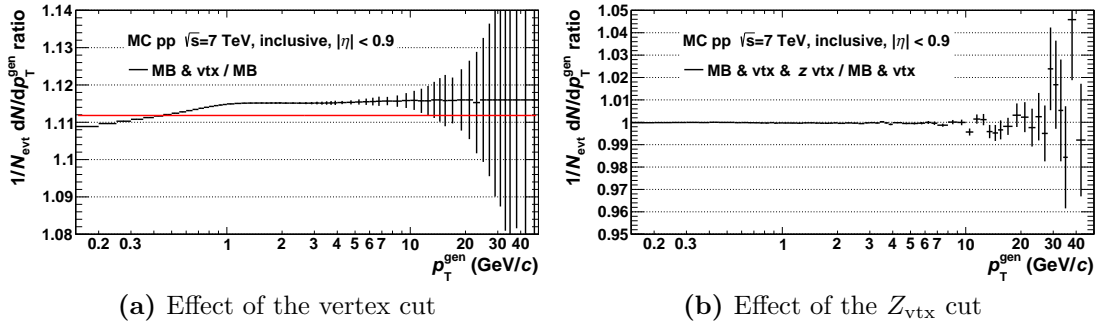
Figure 6.21.: Impact of vertex cuts on the inclusive charged primary p_T spectra in MC. The 1/N_{\text{evt}} \cdot dN/dp_T spectra at the particle level are compared for a) MB trigger selection (“MB”) before and after an additional vertex cut (“vtx”) and b) for MB selection with vertex cut before and after an additional Z_{\text{vtx}} cut (“z vtx”). The solid red line in a) is the fit of a constant to the ratio.
