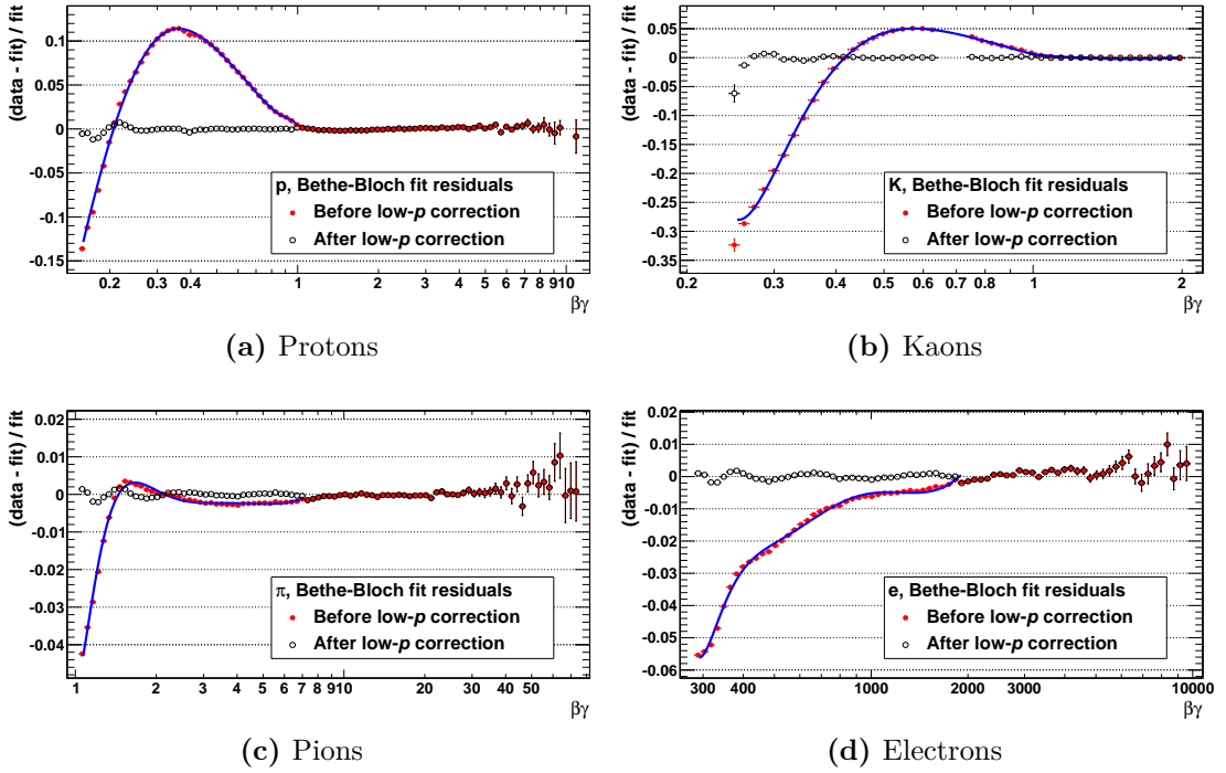
Figure 3.7.: The residuals of the Bethe-Bloch fit for data are shown as red full points. The blue lines are parametrisations of the residuals used to correct for low-momentum effects. The black open points are the difference of the blue lines and the red points.
