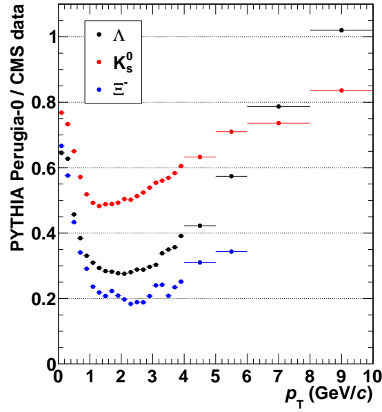
Figure 5.2.: Yield ratio between MC and CMS measurement for different strange particles: \Lambda , K_S^0 and \Xi^- . The MC yields are for PYTHIA tune Perugia-0, which is the same tune that was used to extract the MC corrections in this work. The inverse of the corresponding ratio is used as a strangeness scale factor for the secondary correction.
