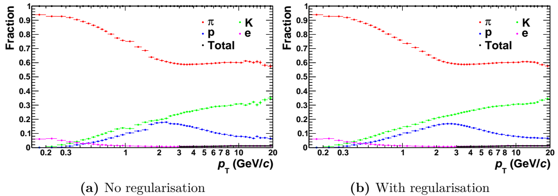
Figure 4.11.: Comparison of raw fractions with and without regularisation as in Fig. 4.9, but for data.
