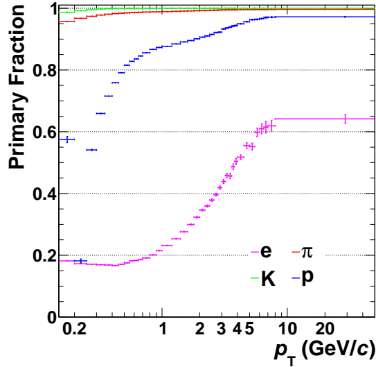
Figure 5.8.: The primary fractions for inclusive spectra are shown for both charges and including strangeness scaling.
