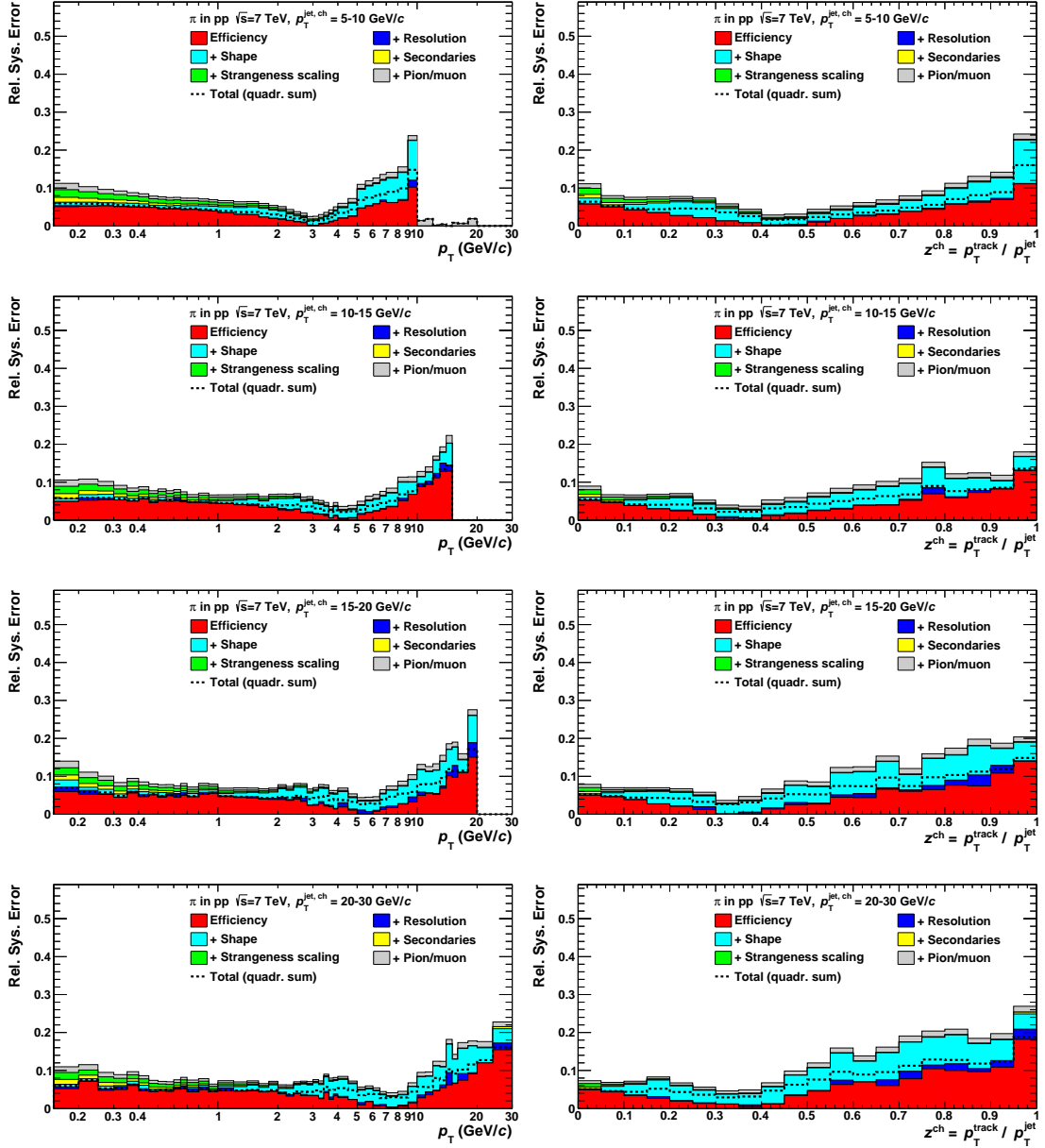
Figure E.6.: Relative systematic uncertainties of the MC correction factors for the pion yields. The rows show (from top to bottom) p_T^{\text{jet}} = 5 - 10, 10 - 15, 15 - 20 and 20 - 30 \text{ GeV}/c , respectively, as a function of p_T^{\text{track}} (left column) and z (right column).
