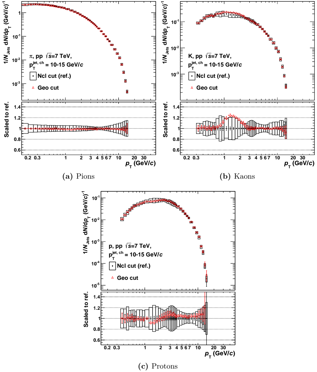
Figure 6.17.: Comparison of the corrected particle yields for the TPC geometrical cut (red open triangles) and the ncl cut (black diamonds) versus p_T^{\text{track}} for p_T^{\text{jet}} = 10 - 15 GeV/c in data. Each set of cuts is corrected with its own MC correction factors. The boxes correspond to the systematic errors for the ncl cut, including the uncertainties of the corresponding MC correction factors.
