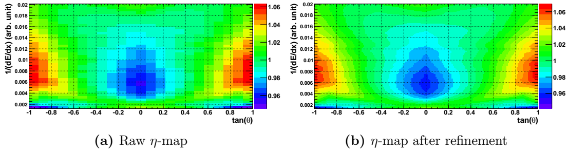
Figure 3.13.: \eta -map obtained from protons. a) shows the raw result from the fits. In b) , the refined map using interpolation is shown. The colour code shows \Delta'_p .
