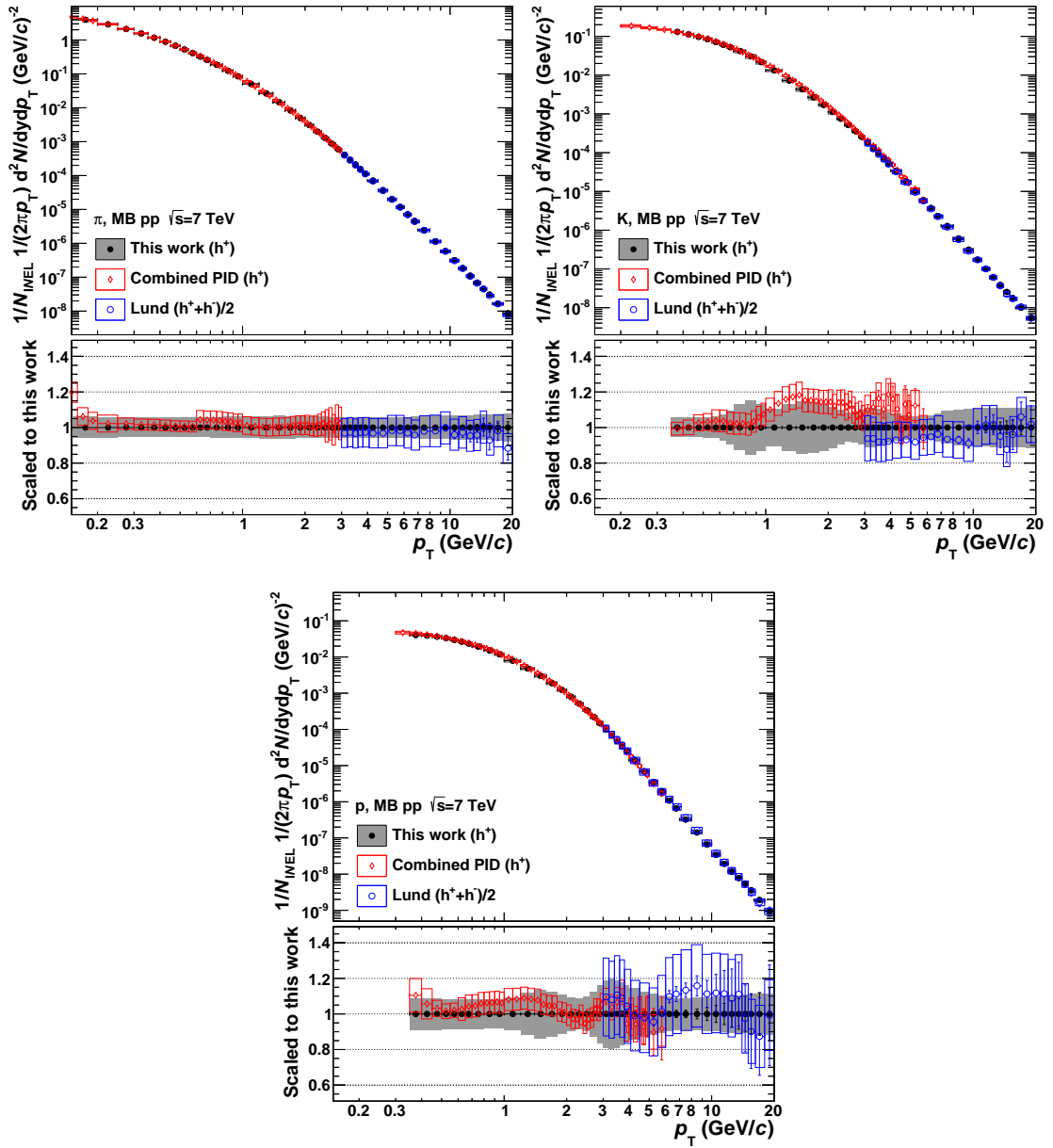
Figure H.4.: The corrected MB yields of positively charged particles are compared to the combined PID [125] and the Lund analysis [126]. The error bars indicate the statistical and the boxes the systematic uncertainties. Note that the Lund result (blue) shows the yield of both charges divided by two.
