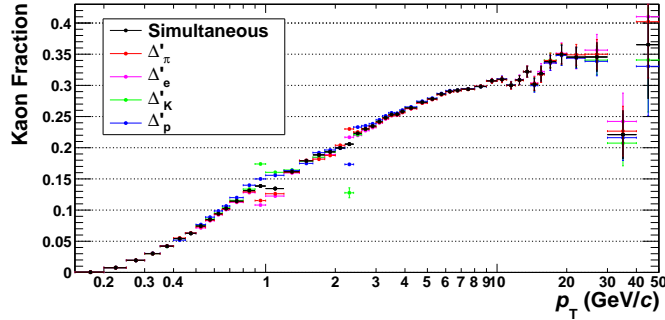
Figure 4.8.: Comparison of kaon fractions with (black points) and without (coloured points) simultaneous fitting for data. The simultaneous fit reduces the fluctuations due to binning effects in the crossing regions. Note that the special templates have been used below 0.3 GeV/c.
