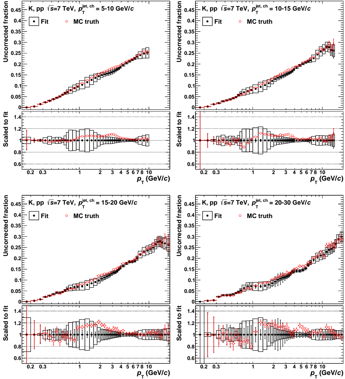
Figure 4.14.: MC blind test for kaons fitted versus p_T . The raw fractions from fitting the MC output (black) are compared to the MC truth (red). The plots show (from upper left to lower right): p_T^{\text{jet, ch}} = 5 - 10 , 10 - 15 , 15 - 20 and 20 - 30 GeV/c.
