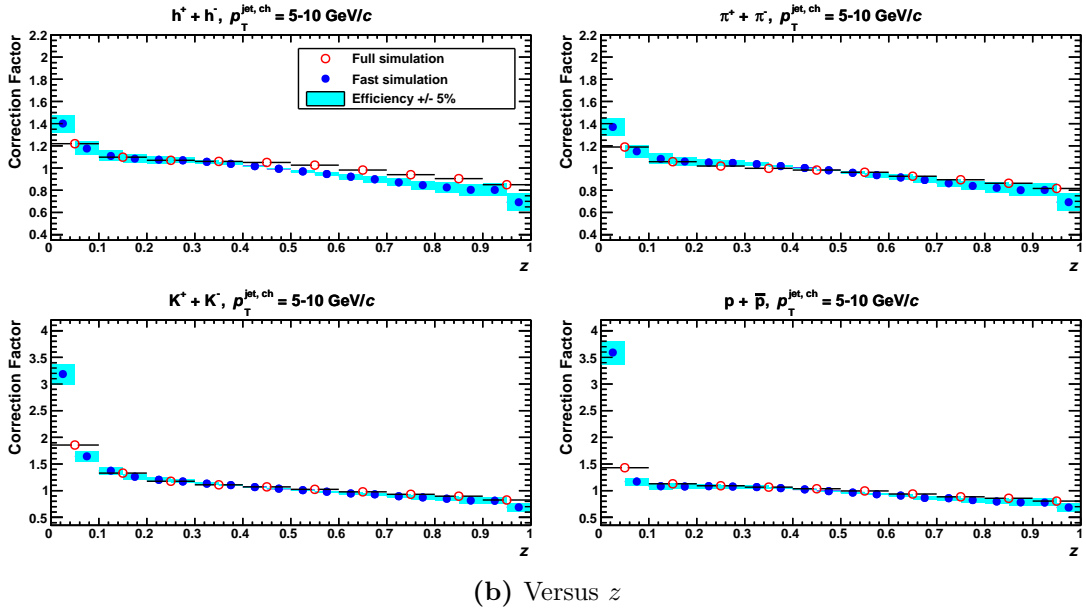
Figure 5.15.: Tracking efficiency systematics. The bin-by-bin correction factors as a function of a) p_T and b) z are shown for all charged particles, \pi , K and p for p_T^{\text{jet}} = 5 - 10 \text{ GeV}/c . The full simulation (open red points) is compared to the fast simulation (full blue points). The cyan bands indicate variations of the toy MC correction factors with efficiency.
