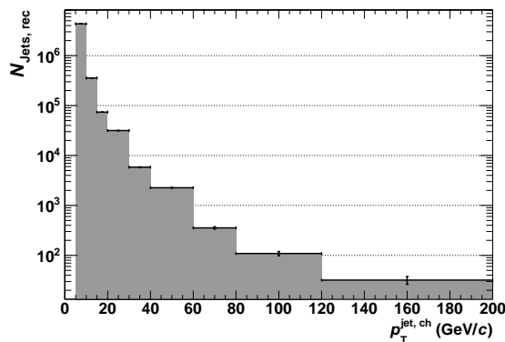
Figure 6.32.: Reconstructed (charged) jet spectrum.
