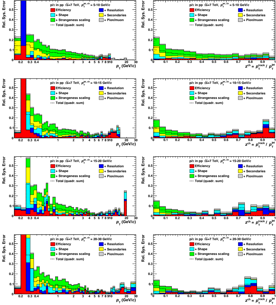
Figure E.10.: Relative systematic uncertainties of the MC correction factors for the to-pion ratios of protons. The rows show (from top to bottom) p_T^{\text{jet}} = 5 - 10, 10 - 15, 15 - 20 and 20 - 30 GeV/c, respectively, as a function of p_T^{\text{track}} (left column) and z (right column).
