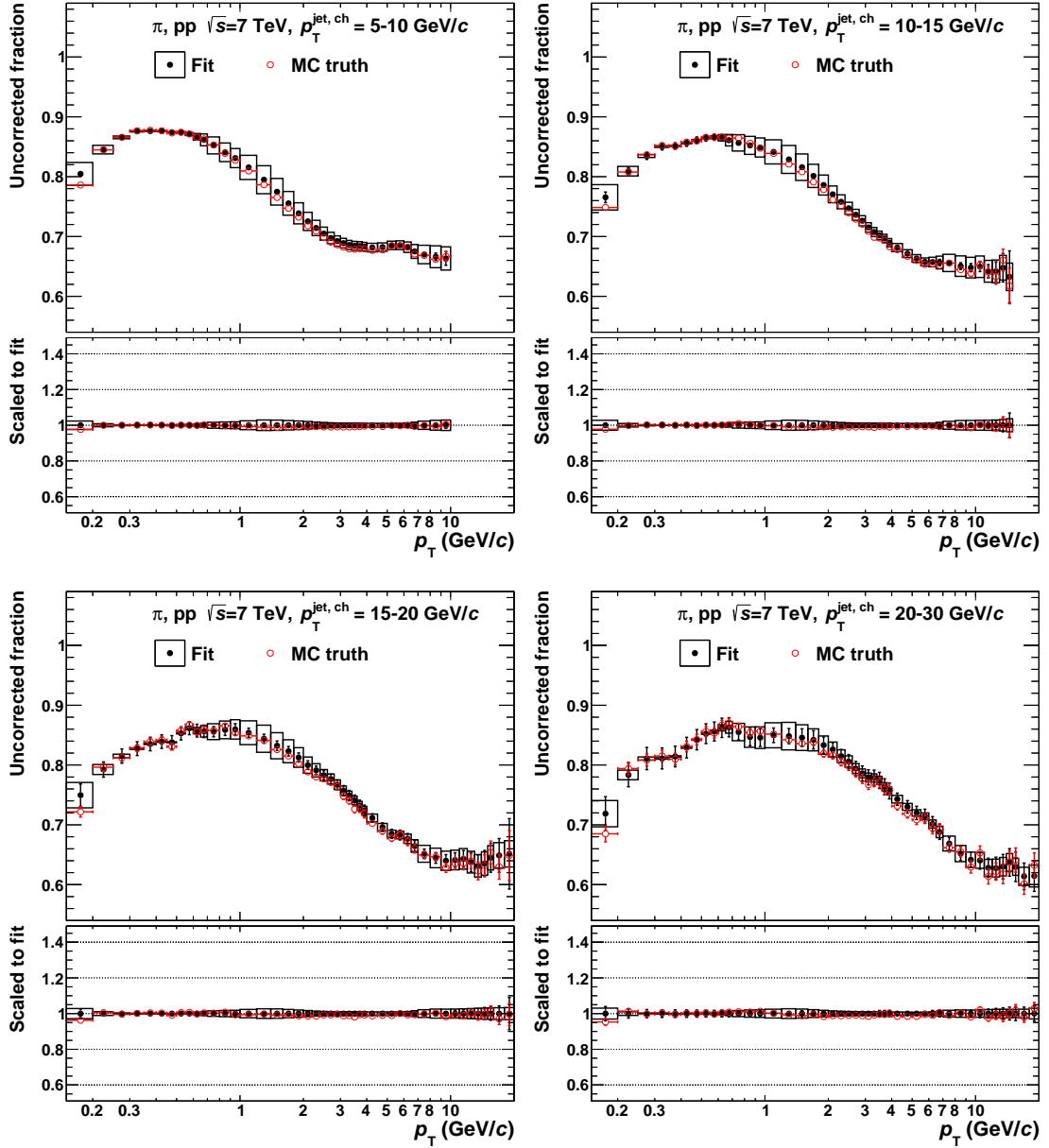
Figure 4.13.: MC blind test for pions fitted versus p_T . The raw fractions from fitting the MC output (black) are compared to the MC truth (red). The plots show (from upper left to lower right): p_T^{\text{jet}} = 5 - 10, 10 - 15, 15 - 20 and 20 - 30 \text{ GeV}/c .
