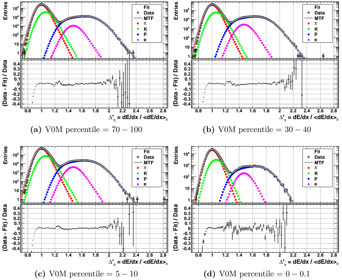
Figure F.3.: Template fits to data for different V0M percentile bins for p_T = 0.8 - 0.9 GeV/c. The V0M percentile decreases from the upper left to the lower right plot.
