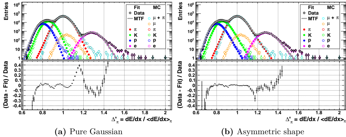
Figure 4.4.: Comparison of a) pure Gaussian and b) asymmetric response in MC. In the upper panels, the dE/dx distribution for p_T = 4.0 - 4.5 GeV/ c is shown in black together with the templates (full points), the MC true response (open points) and the fit (grey line). The lower panels show the relative deviation of the fit from data.
