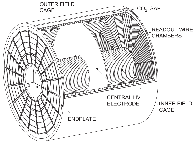
Figure 2.4.: Schematic view of the TPC. Figure from [73].
