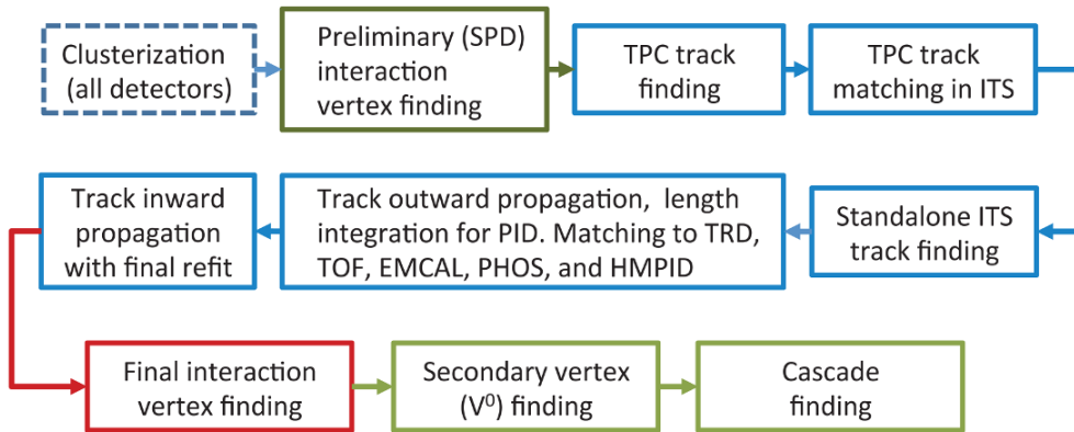
Figure 2.6.: Event reconstruction flow for the central barrel. Figure from [70].
