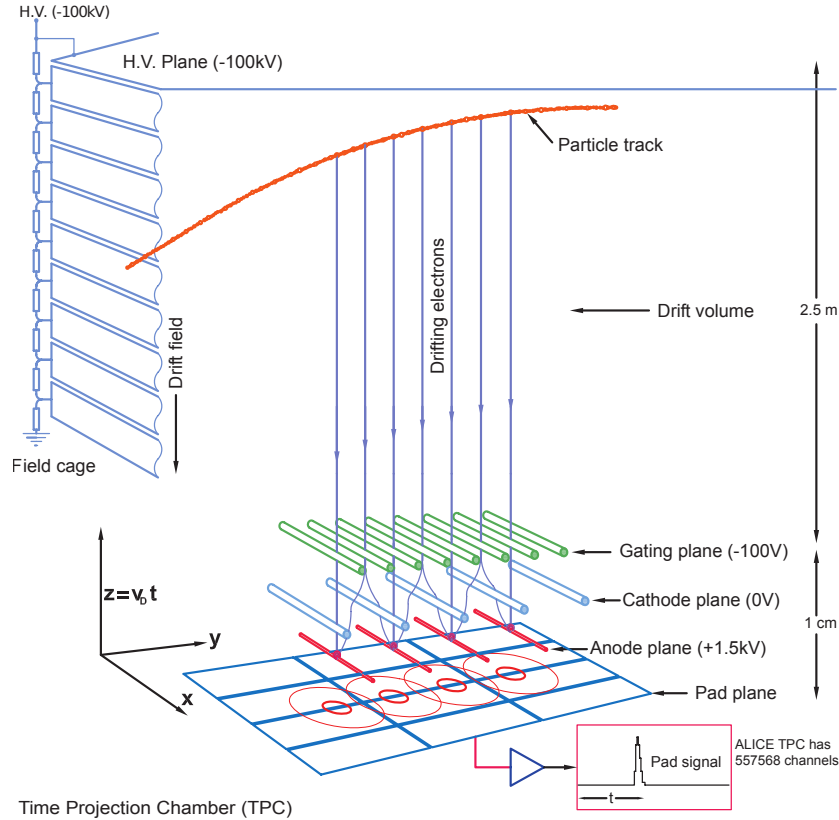
Figure 2.5.: Illustration of the TPC working principle. The field lines are shown for the case that the gating grid is “open”. Figure from [74].
