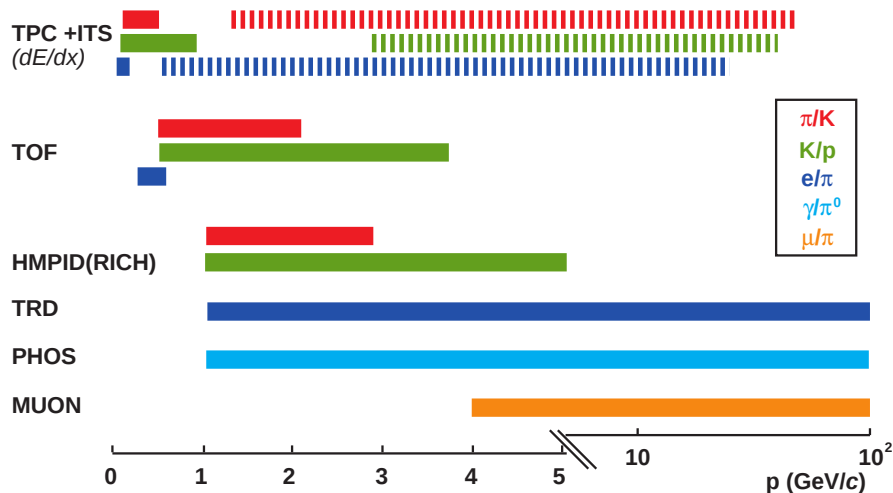
Figure 2.3.: Overview of the particle identification capabilities of the ALICE detector system. The values of this plot are based on [68]. The broken bars indicate momentum regions, in which only PID on statistical basis can be performed by the corresponding detectors. Taking all detectors together, ALICE allows to identify particles in a wide momentum range. Figure from [69].
