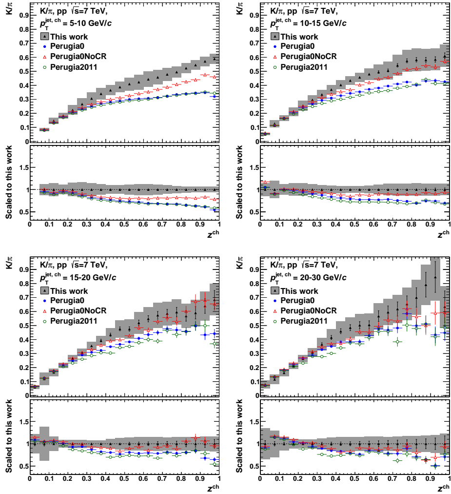
Figure K.10.: Comparison of corrected K/\pi ratios in jets to different MC predictions as a function of z . The p_T^{\text{jet}} increases from the upper left to the lower right panel.
