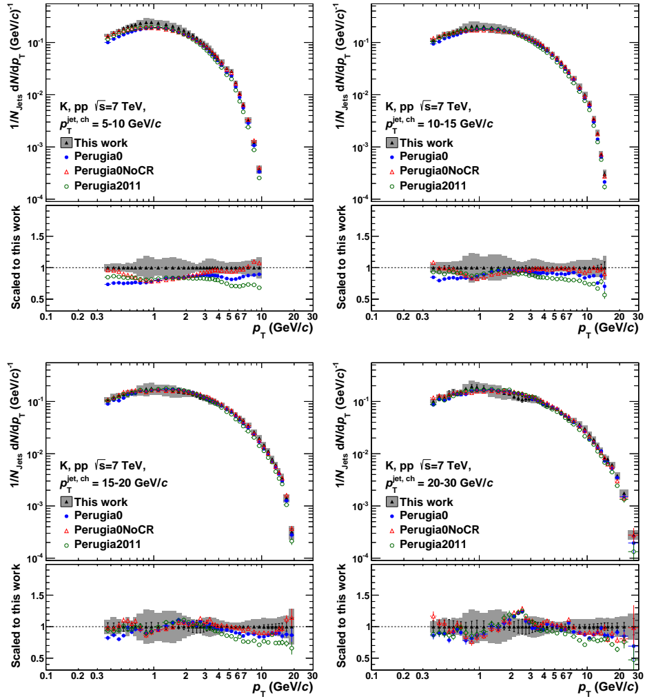
Figure K.5.: Comparison of corrected kaon yields in jets to different MC predictions as a function of p_T . The p_T^{\text{jet}} increases from the upper left to the lower right panel.
