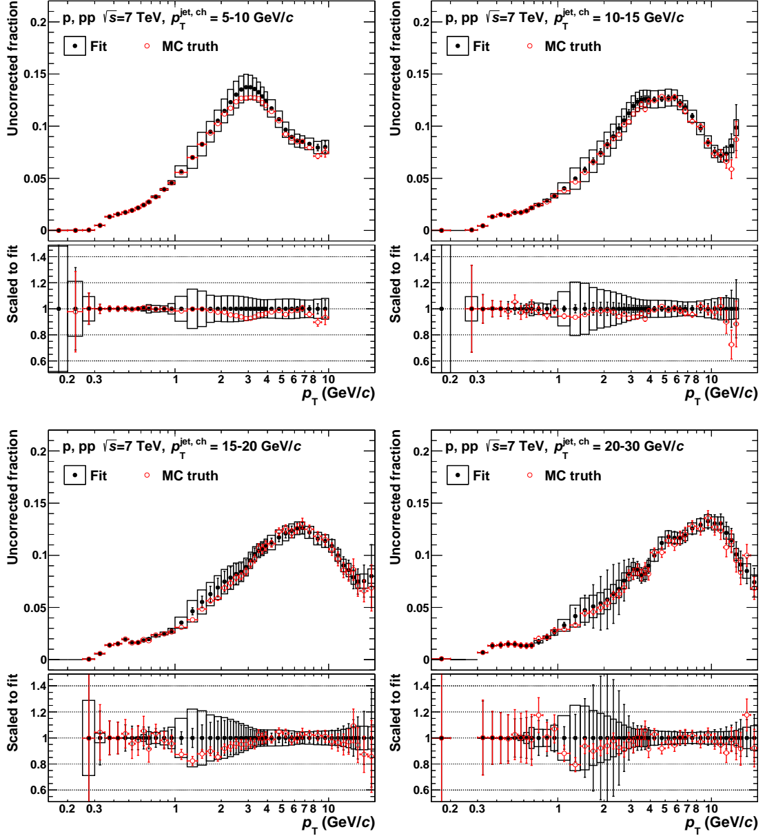
Figure 4.15.: MC blind test for protons fitted versus p_T . The raw fractions from fitting the MC output (black) are compared to the MC truth (red). The plots show (from upper left to lower right): p_T^{\text{jet}} = 5 - 10 , 10 - 15 , 15 - 20 and 20 - 30 GeV/c.
