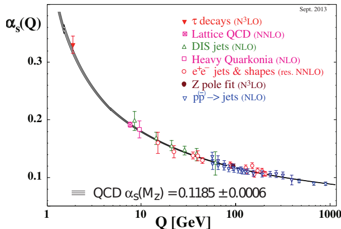
Figure 1.1.: Running of the strong coupling constant \alpha_s as a function of the momentum transfer Q . Figure from [3].
