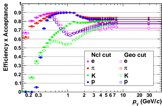
Figure 6.15.: The MC single track efficiencies of the ncl cut (dots) are compared to those of the geo cut (open boxes). Compared to the ncl cut, the geo cut is most effective around p_T = 1 GeV/ c and saturates at a 5% lower efficiency for p_T > 5 GeV/ c .
