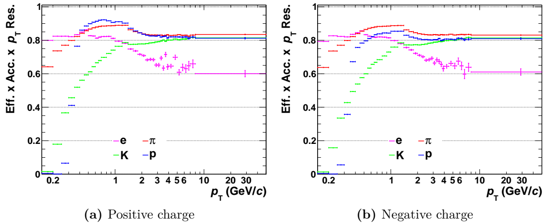
Figure 5.7.: The (inverse) efficiency \times acceptance \times p_T resolution correction factors for inclusive particle production are shown for particles with a) positive and b) negative charge. The GEANT-FLUKA correction is already included.
