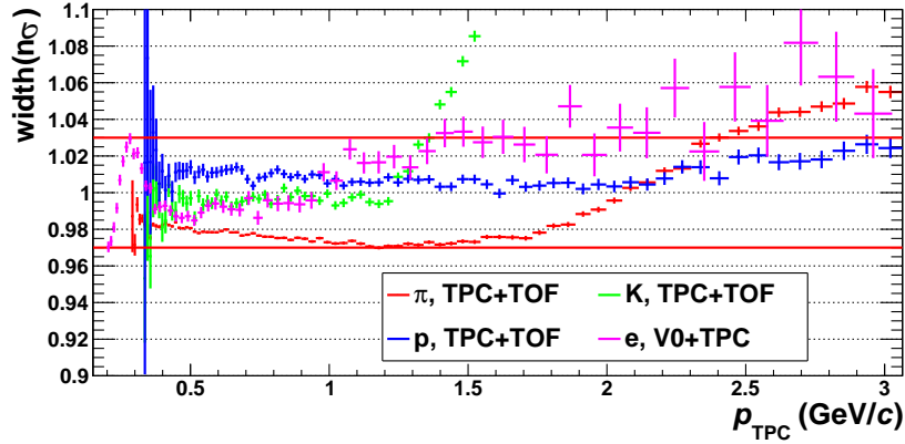
Figure 3.17.: Accuracy of the resolution map in data. The fitted Gaussian width of the n_{\sigma, \text{TPC}} distribution is shown for primary particles selected by TOF (except for the magenta data points, which are from V0's). For every data sample, a TPC cut was applied in the sense that the Gauss fit has been restricted to \pm 1.5\sigma around the expected dE/dx . Note that at some momentum contamination shifts the width to larger values. The horizontal red lines show the \pm 3\% region around unity, which largely covers the deviations of all species.
