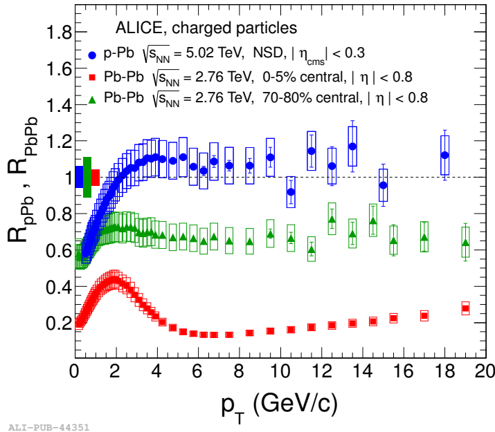
Figure 1.4.: ALICE measurement of charged particle medium modification factors in p–Pb and Pb–Pb collisions. In addition, central (red squares) and peripheral (green triangles) Pb–Pb collisions are compared. Figure from [40].
