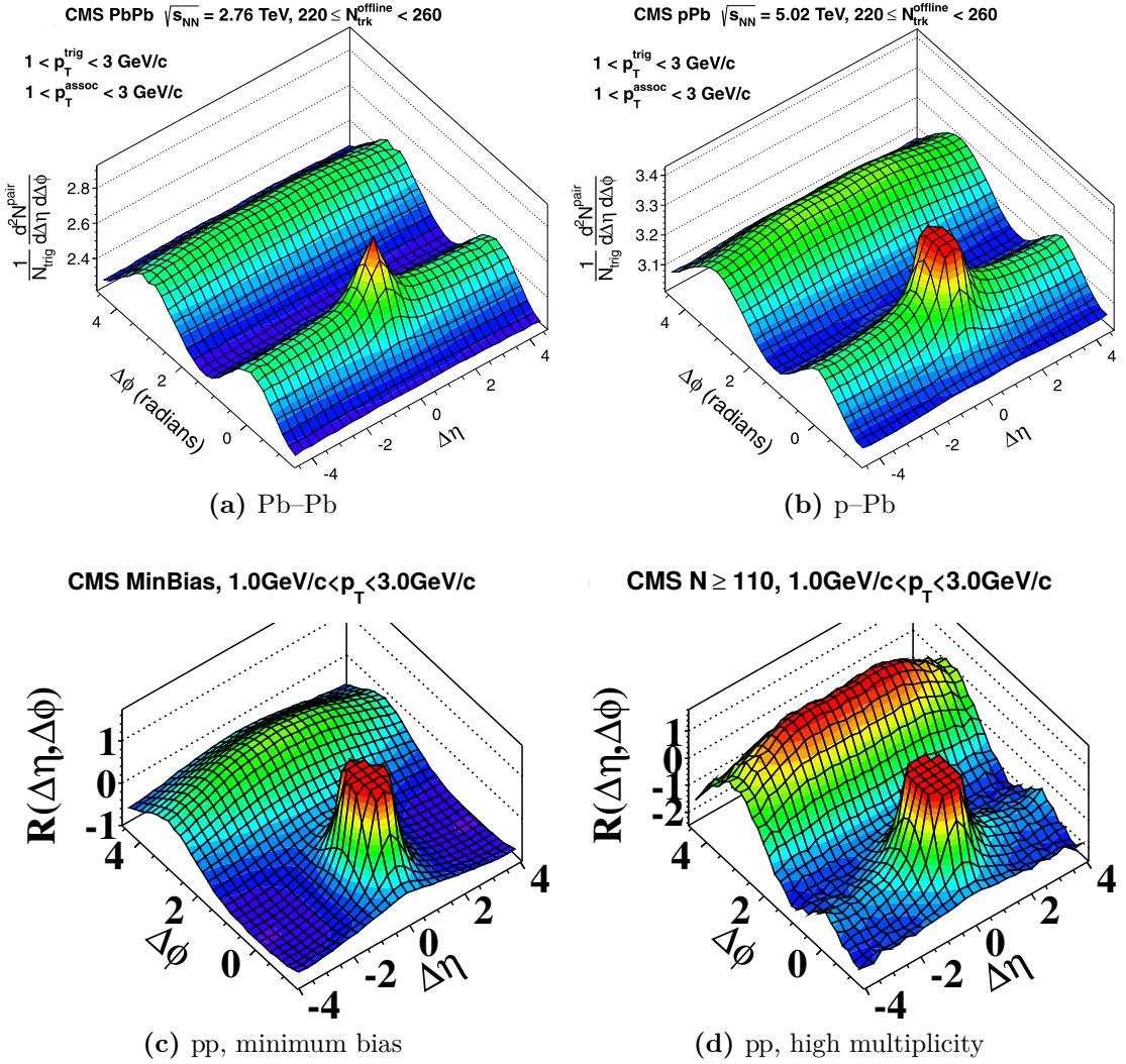
Figure 1.5.: CMS measurement of two-particle correlations in different collision systems at intermediate transverse momentum. The near-side ridge is clearly visible in a) Pb-Pb and b) p-Pb collisions (figures from [41]). In pp collisions, it is not observed for c) minimum bias, but seems to appear for d) high multiplicity (figures from [42]).
