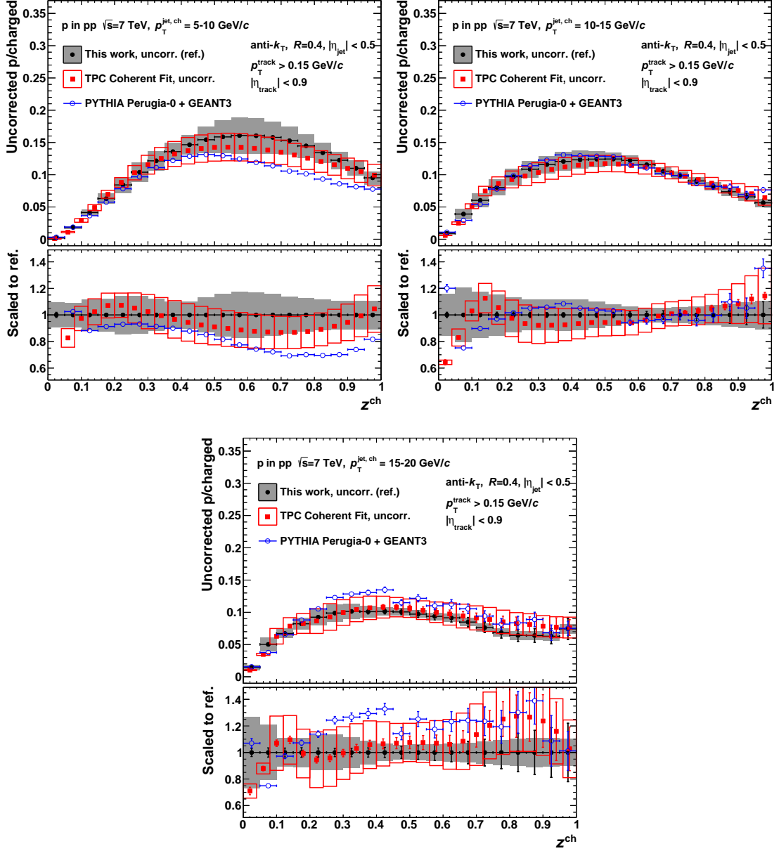
Figure H.3.: Comparison of uncorrected proton fractions as a function of z to the TPC Coherent Fit. In addition, the MC prediction from PYTHIA Perugia-0 is overlaid.
