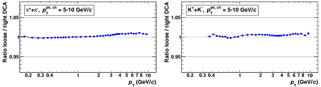
Figure 5.17.: Ratio loose/tight DCA for pions (left) and kaons (right) in jets with p_T^{\text{jet}} = 5 - 10 \text{ GeV}/c .
