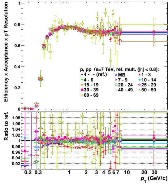
(c) Protons
