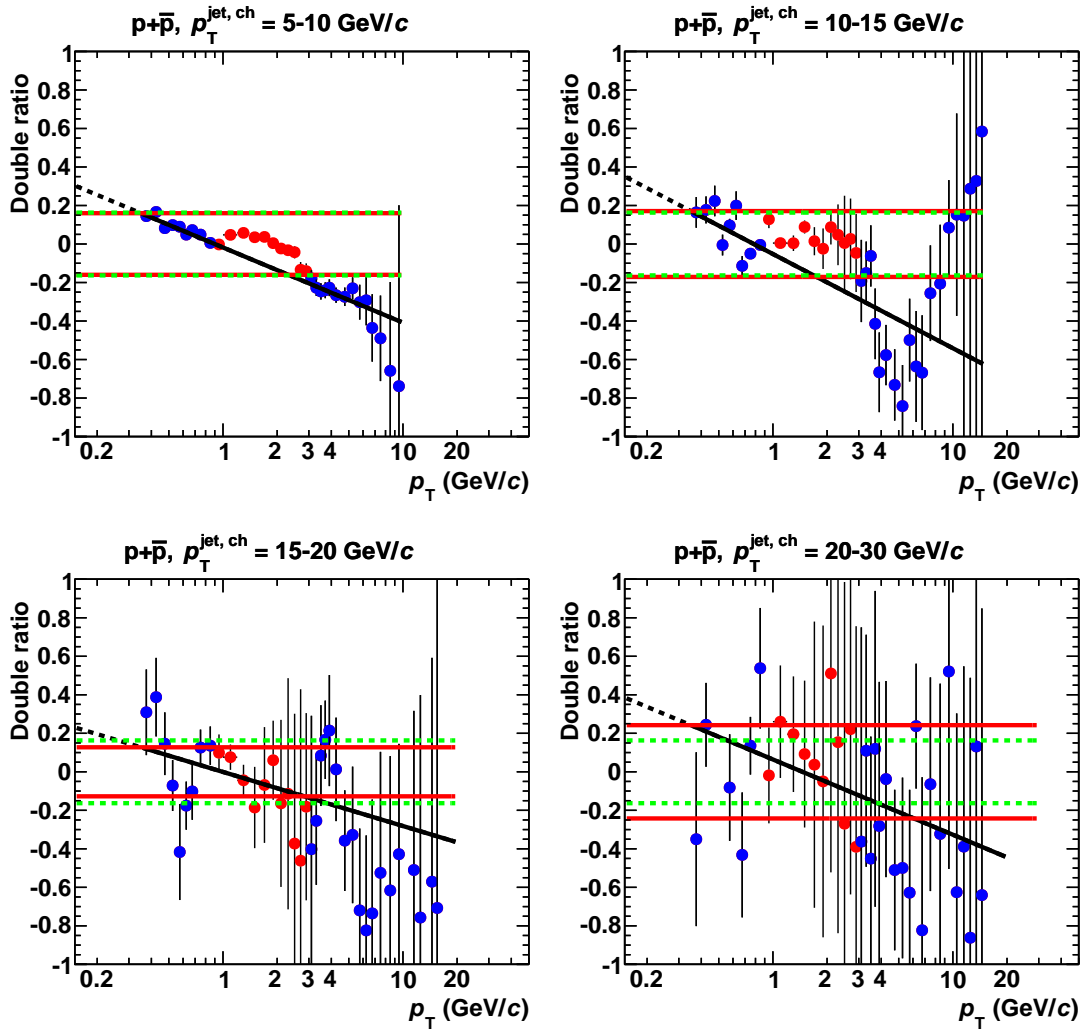
Figure 5.20.: Double ratio for protons in jets. The red points have been excluded from the fit. See discussion in the text for further details.
