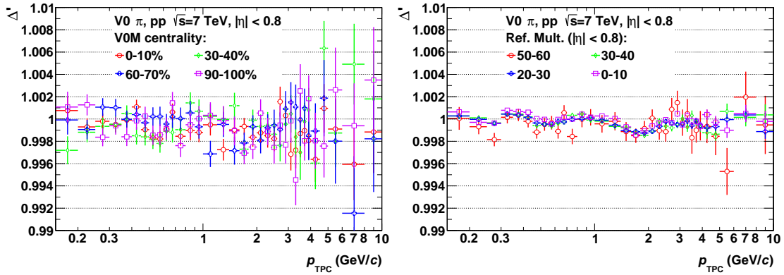
Figure 6.25.: Multiplicity dependence of the mean dE/dx for V0 pions. The left and right panels compare the \Delta' in different bins of VOM multiplicity and reference multiplicity, respectively.
