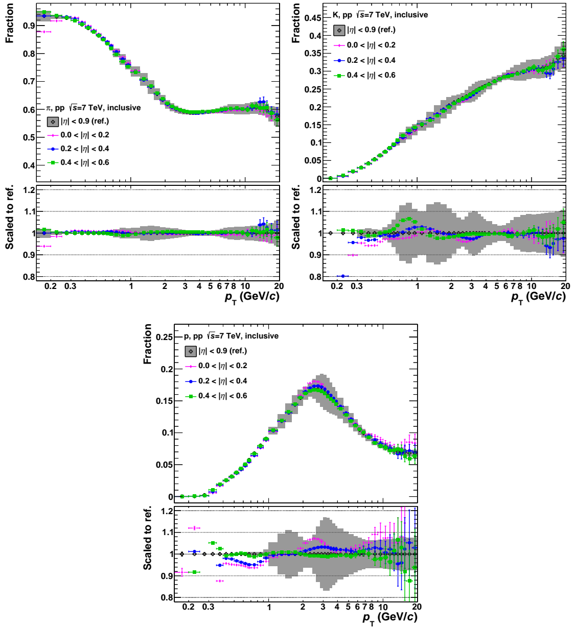
Figure G.1.: Comparison of the uncorrected particle fractions in \eta slices (coloured symbols) and in the full \eta range (black open crosses) versus p_T^{\text{track}} for the inclusive case in data. The results are shown for (from upper left to lower right) \pi , K and p. The grey area indicates the systematic uncertainties for the full \eta range.
