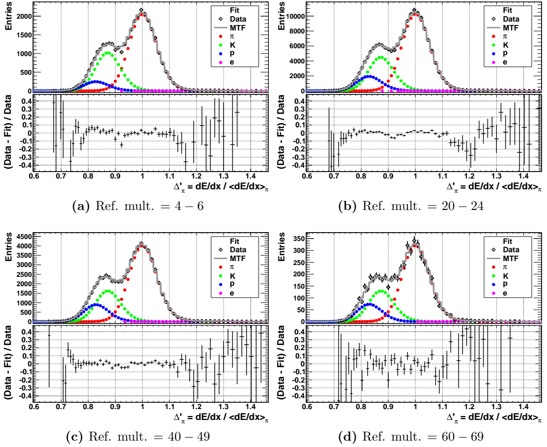
Figure 6.26.: Template fits to data for different reference multiplicity bins for p_T = 4 - 4.5 \text{ GeV}/c . The reference multiplicity increases from the upper left to the lower right plot.
