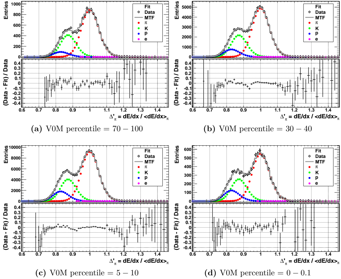
Figure F.4.: Template fits to data for different V0M percentile bins for p_T = 4 - 4.5 \text{ GeV}/c . The V0M percentile decreases from the upper left to the lower right plot.
