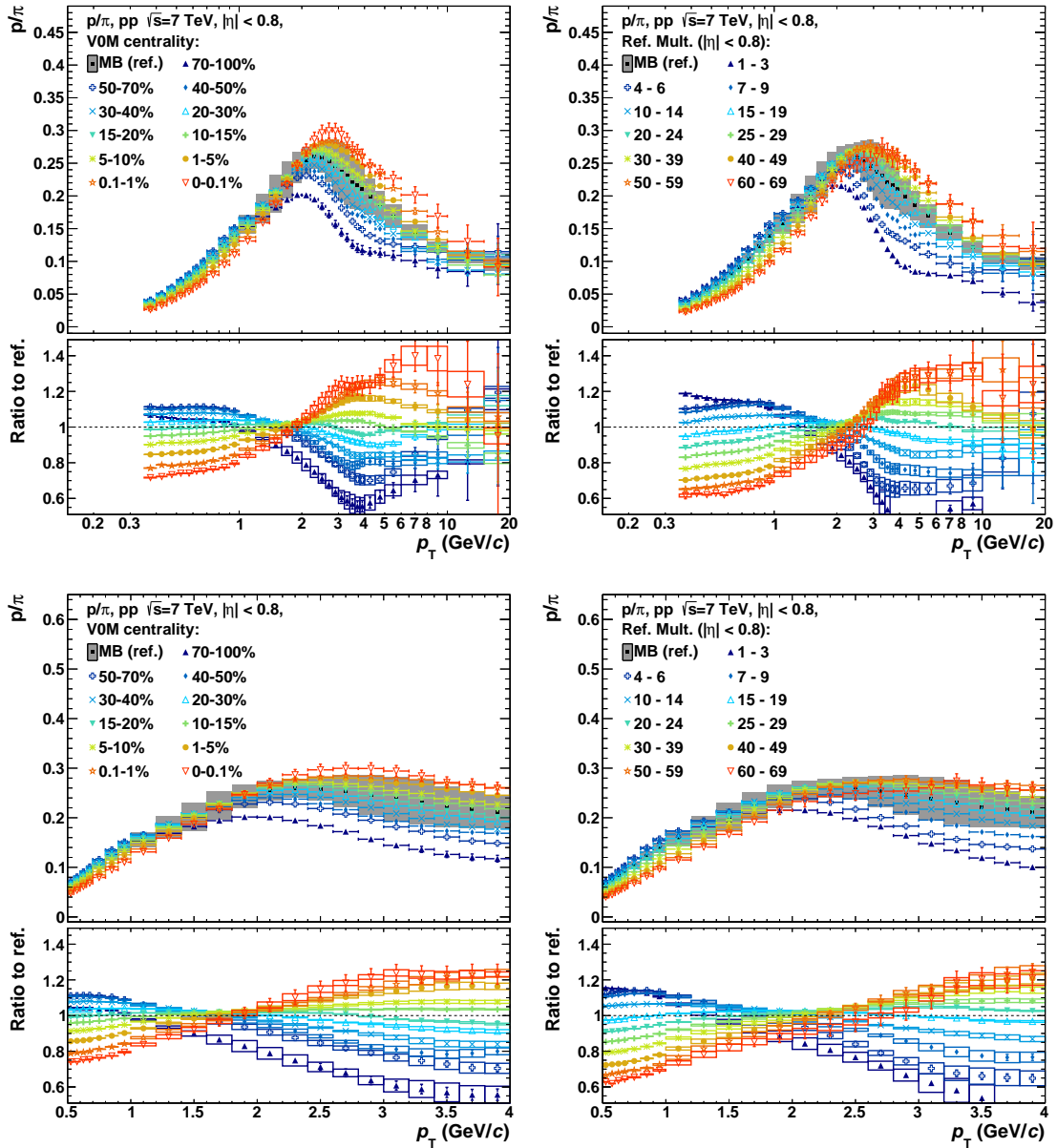
Figure 6.30.: p/\pi ratios for different bins of VOM (left) and reference multiplicity (right). For better visibility, only the systematic uncertainties of the MB data points are plotted in the upper panel of each row. The lower panel of each row shows the ratio to MB including the corresponding systematic uncertainties. The bottom row shows a zoom to the crossing point with linear p_T scale.
