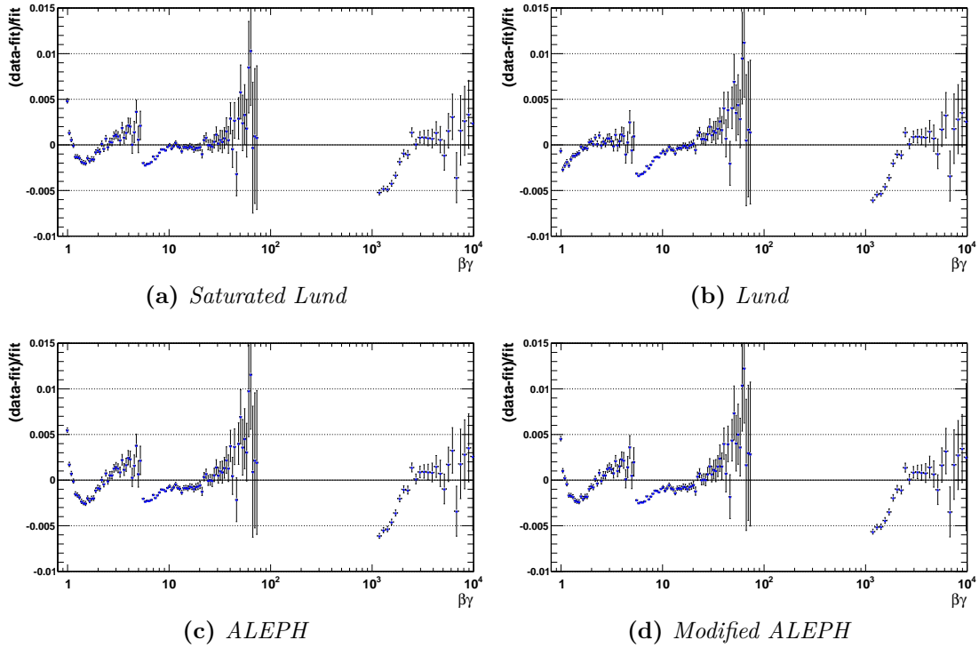
Figure 3.10.: Fit residuals of a) Saturated Lund , b) Lund , c) ALEPH and d) Modified ALEPH . The residuals are for the pure fit, without any low-momentum correction.
