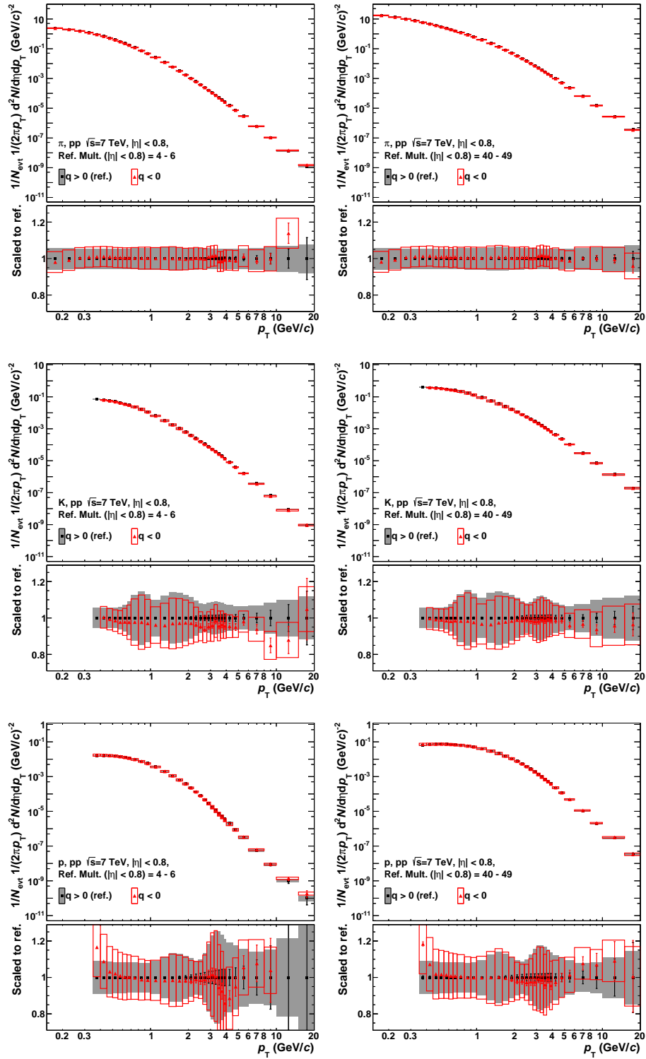
Figure J.1.: Comparison of positively ( q > 0 ) and negatively ( q < 0 ) charged particles for the reference multiplicity bins 4 – 6 (left) and 40 – 49 (right). The rows show (from top to bottom): \pi , K and p.
