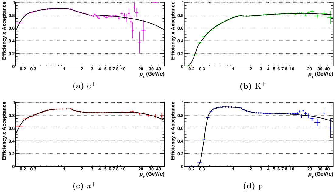
Figure 5.14.: The single track efficiencies for positive particles are shown. The black lines are a parametrisation of the data points that allow for a smooth description.
