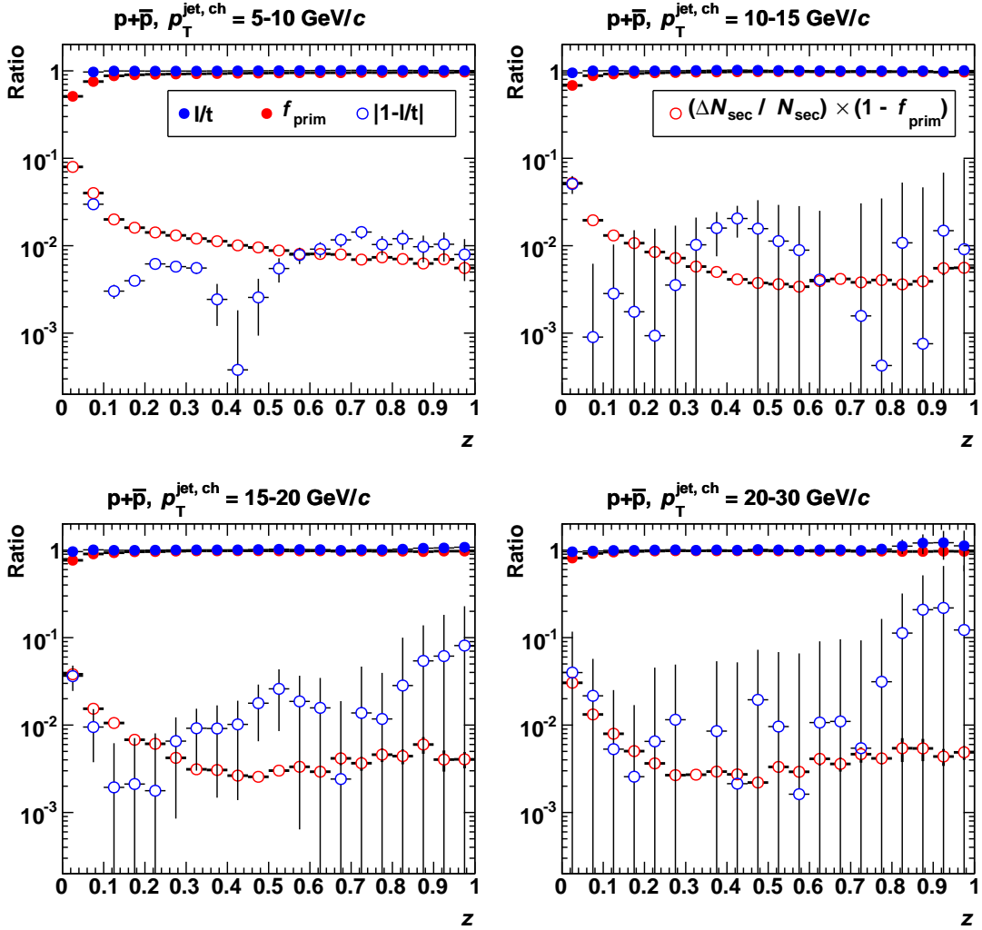
Figure E.4.: Summary plot for the systematic uncertainty estimation of the secondary correction for protons in jets as a function of z . The open red points show the relative systematic uncertainty estimate and should be compared to the open blue points, which show the relative change of spectra due to DCA cut variations.
