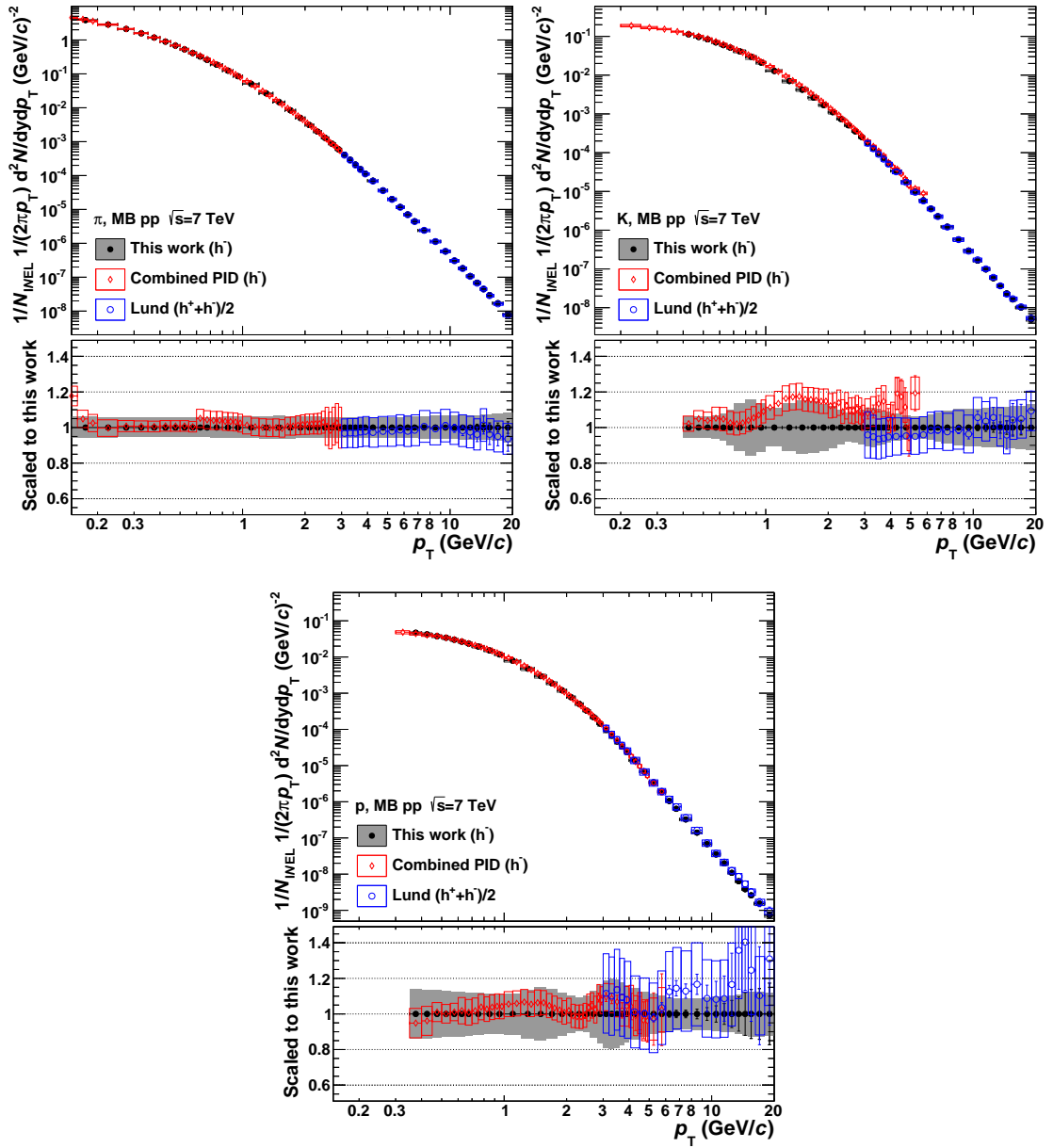
Figure 6.23.: The corrected MB yields of negatively charged particles are compared to the combined PID [125] and the Lund analysis [126]. The error bars indicate the statistical and the boxes the systematic uncertainties. Note that the Lund result (blue) shows the yield of both charges divided by two.
