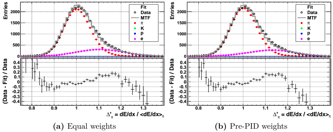
Figure 6.12.: Shape uncertainty of pre-PID weighting for p_T^{\text{track}} = 0.15 - 0.2 \text{ GeV}/c and p_T^{\text{jet}} = 10 - 15 \text{ GeV}/c in data. Effectively, there are no kaons and protons due to low detection efficiency. a) shows the template shapes created with equal weights, while in b) , the pre-PID weights with priors have been used.
