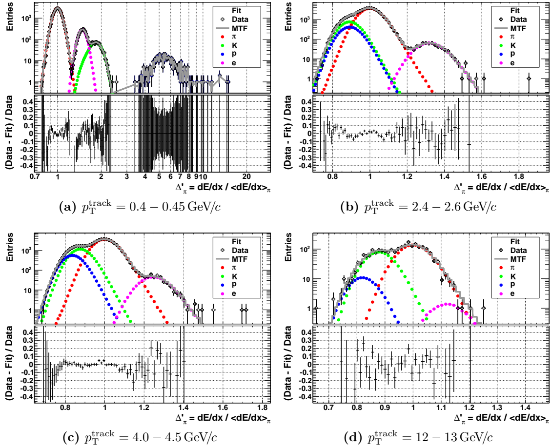
Figure 6.2.: Template fits to data in different p_T^{\text{track}} intervals for p_T^{\text{jet}} = 10 - 15 \text{ GeV}/c . The panels a) - d) show the following p_T^{\text{track}} ranges in \text{GeV}/c : 0.4 - 0.45, 2.4 - 2.6, 4.0 - 4.5 and 12 - 13. Note the different ranges of the abscissa and its logarithmic scale in a) .
