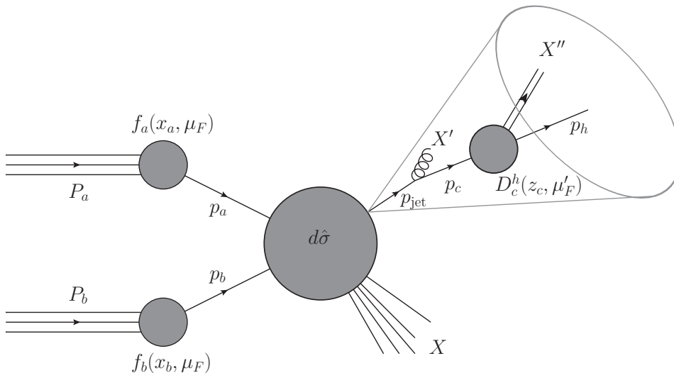
Figure 1.3.: Illustration of the semi-inclusive identified jet production. The partons a and b of the incoming protons experience a hard-scattering. The emerging parton c fragments into the hadron h , which is part of a jet.
