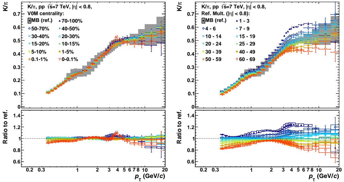
Figure 6.29.: K/\pi ratios for different bins of VOM (left) and reference multiplicity (right). For better visibility, only the systematic uncertainties of the MB data points are plotted in the upper panel. The lower panel shows the ratio to MB including the corresponding systematic uncertainties.
