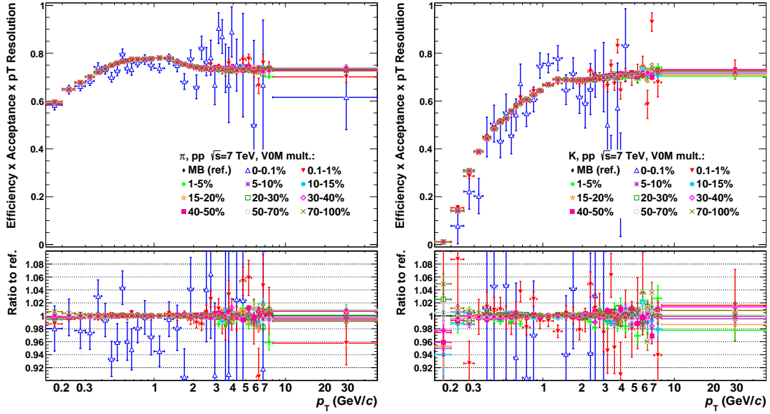
(a) Pions
