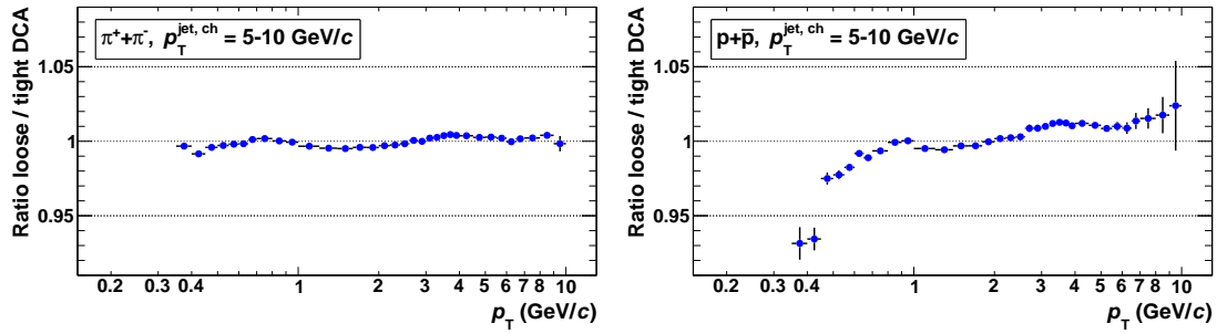
Figure 5.18.: Ratio loose/tight DCA for pions (left) and protons (right) in jets with p_T^{\text{jet}} = 5 - 10 \text{ GeV}/c after applying the kaon correction.
