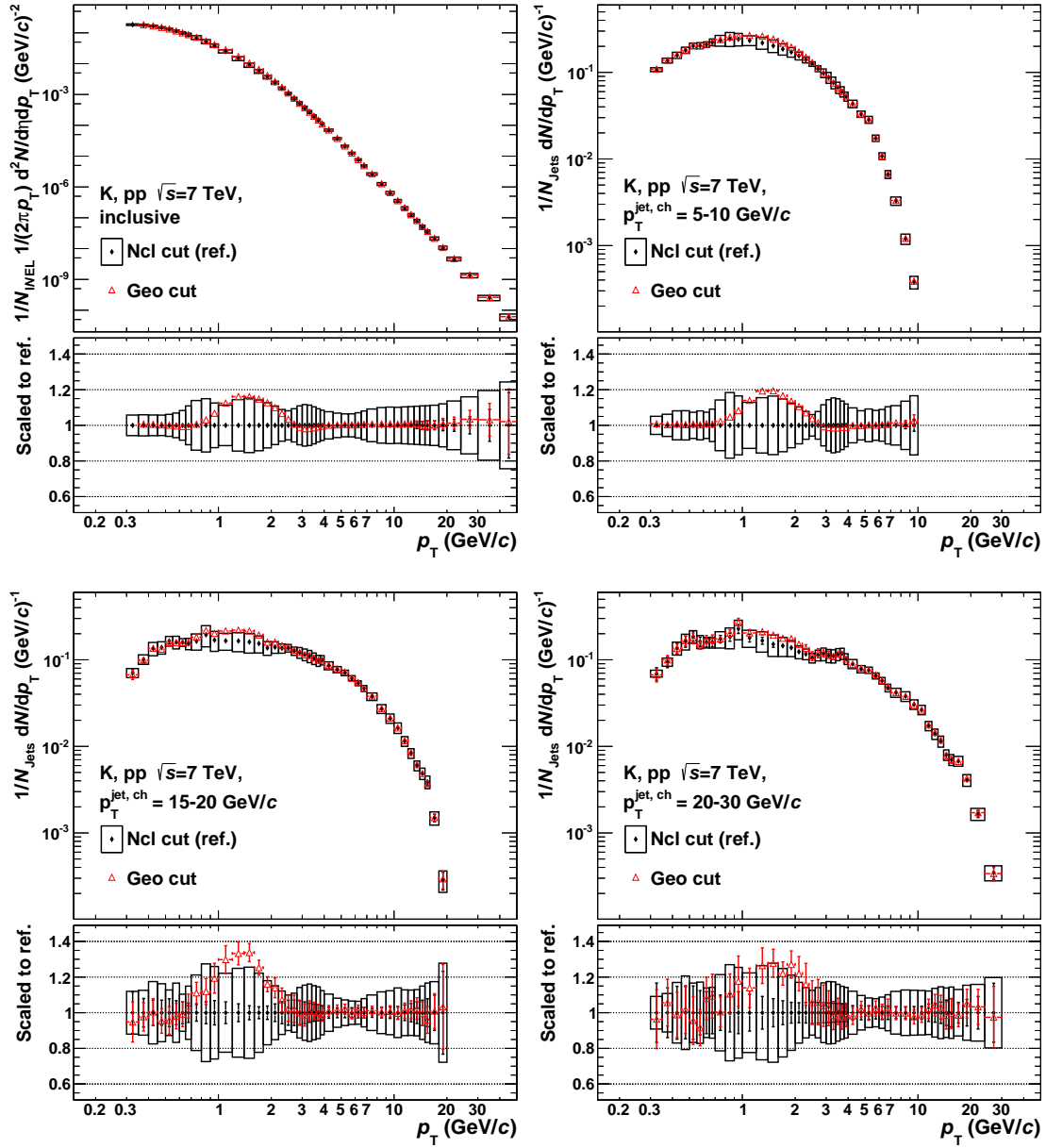
Figure I.2.: Comparison of the corrected kaon yields for the TPC geometrical cut (red open triangles) and the ncl cut (black diamonds) versus p_T^{\text{track}} in data. Each set of cuts is corrected with its own MC correction factors. The boxes correspond to the systematic errors for the ncl cut, including the uncertainties of the corresponding MC correction factors.
