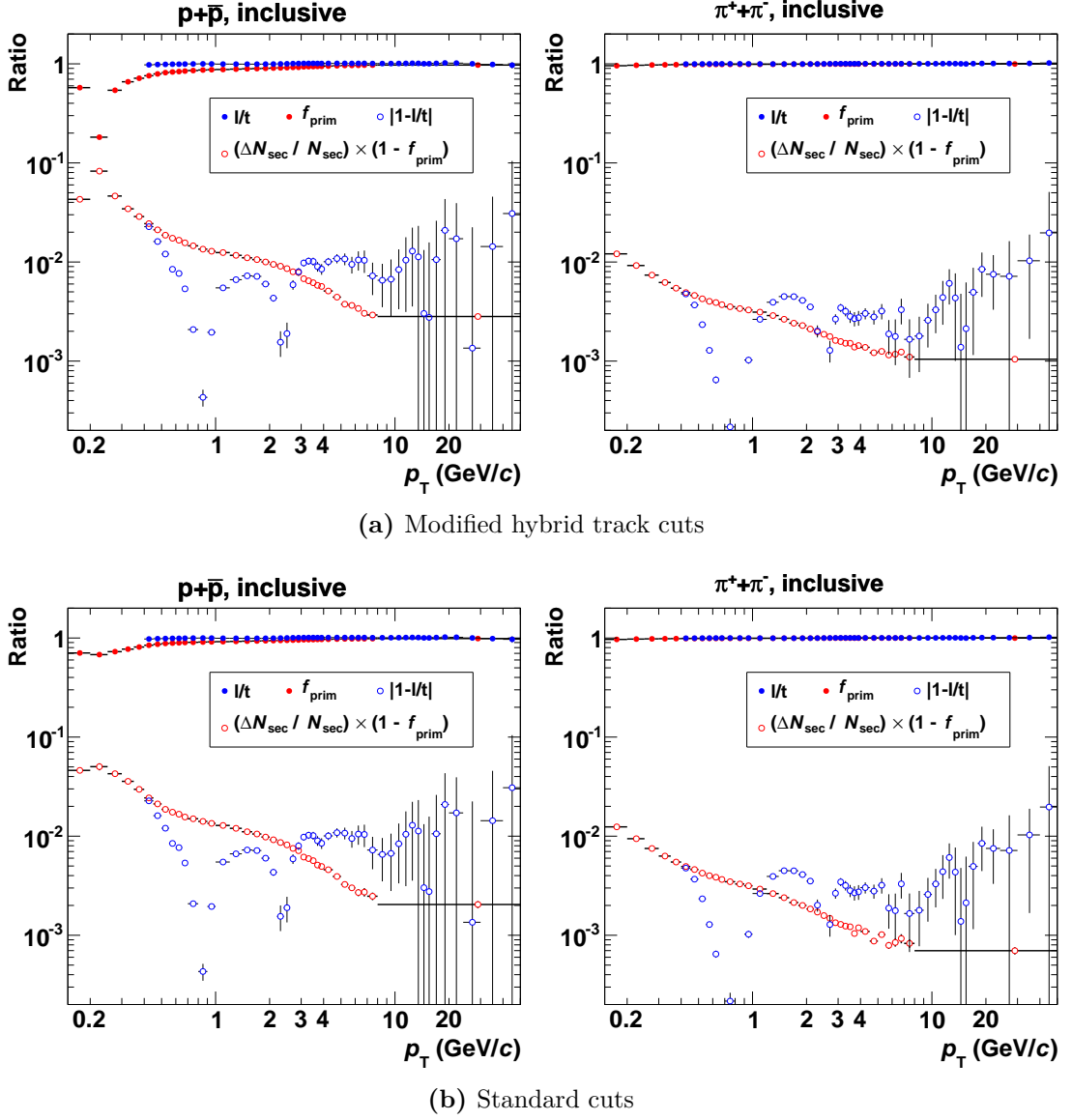
Figure E.3.: Summary plot for the systematic uncertainty estimation of the secondary correction for protons (left) and pions (right) in the inclusive case. The modified hybrid track cuts (a) are compared to the standard cuts (b). The open red points show the relative systematic uncertainty estimate and should be compared to the open blue points, which show the relative change of spectra due to DCA cut variations.
