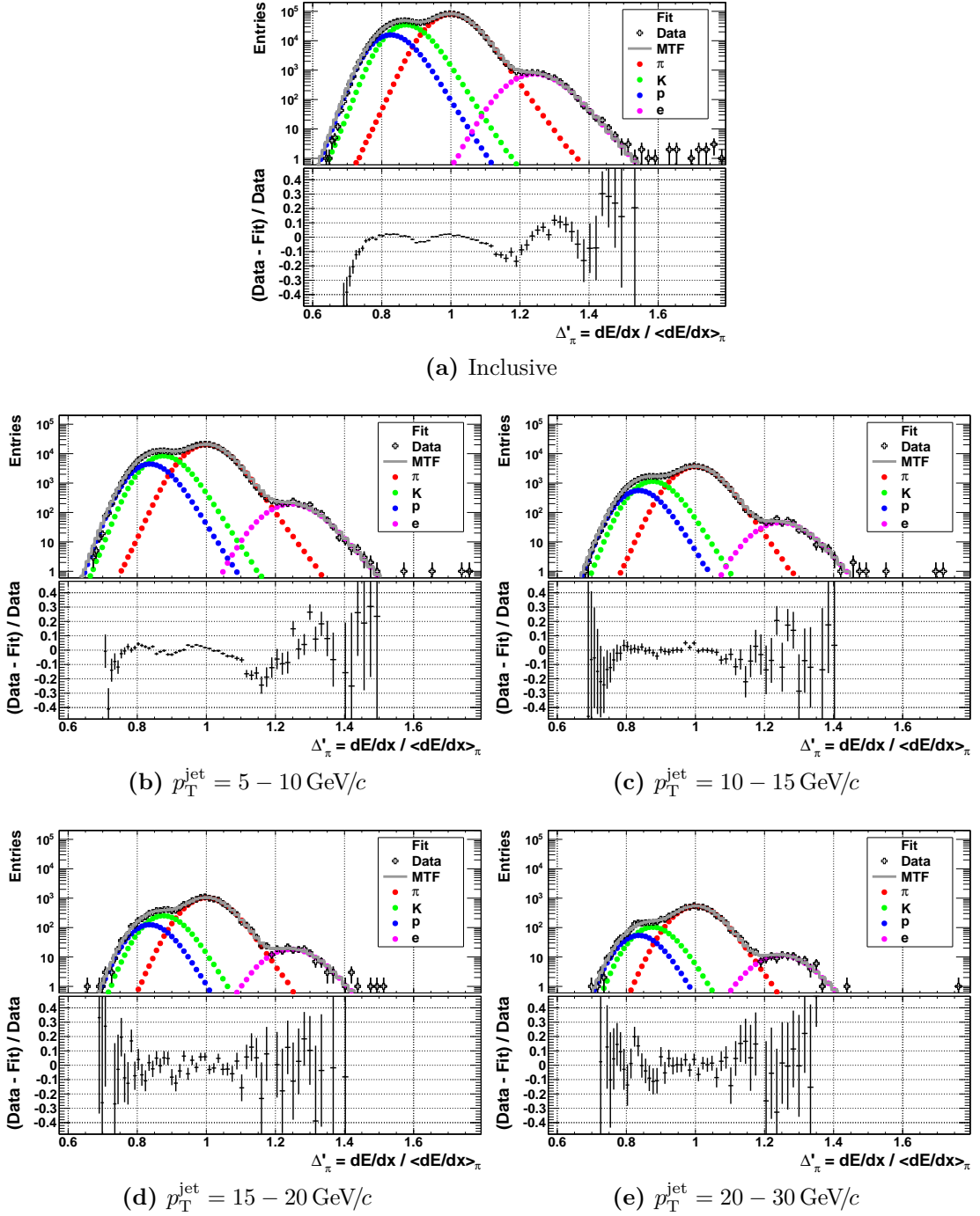
Figure 6.3.: Comparison of the template fits for minimum bias data and jet constituents. The fits are shown for p_T^{\text{track}} = 4 - 4.5 \text{ GeV}/c .
