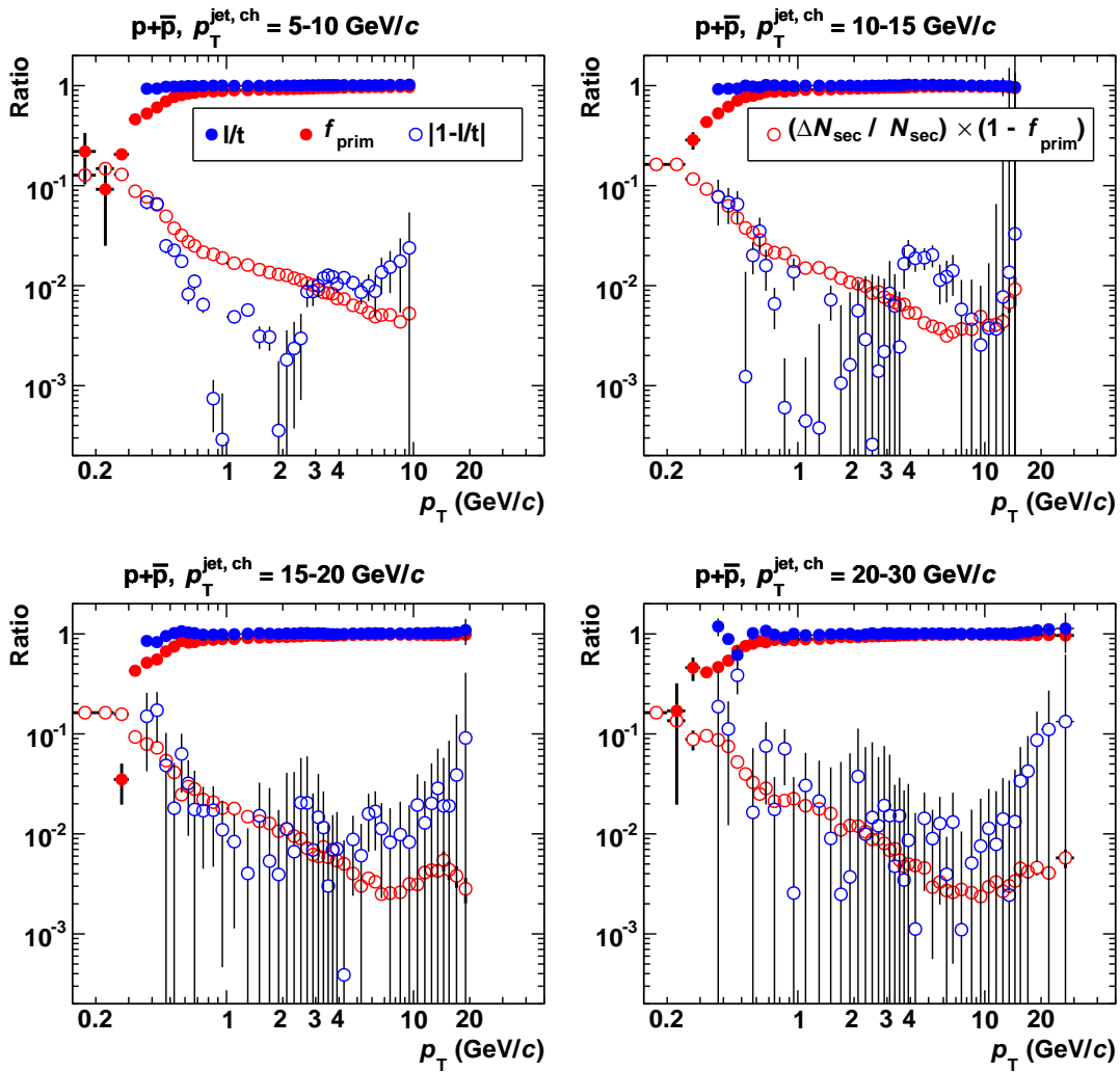
Figure 5.22.: Summary plot for the systematic uncertainty estimation of the secondary correction for protons in jets as a function of p_T . The open red points show the relative systematic uncertainty estimate and should be compared to the open blue points, which show the relative change of spectra due to DCA cut variations.
