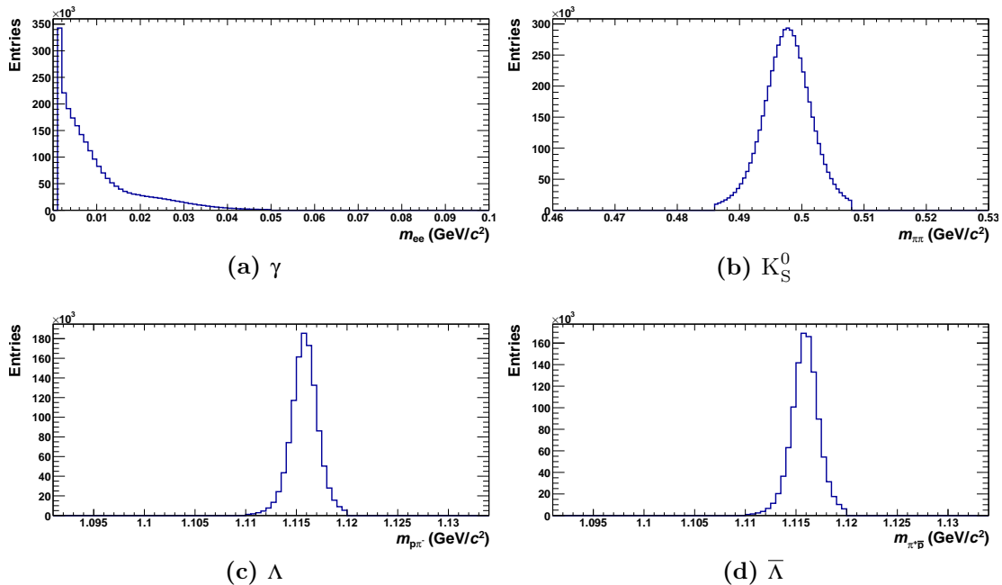
Figure 3.5.: Invariant mass distributions of V0 mothers of particles used to extract the TPC PID response. The cuts have already been applied.
