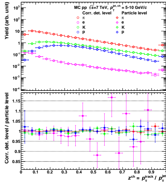
(c) p_T^{\text{jet}} = 5 - 10 GeV/c, versus z
