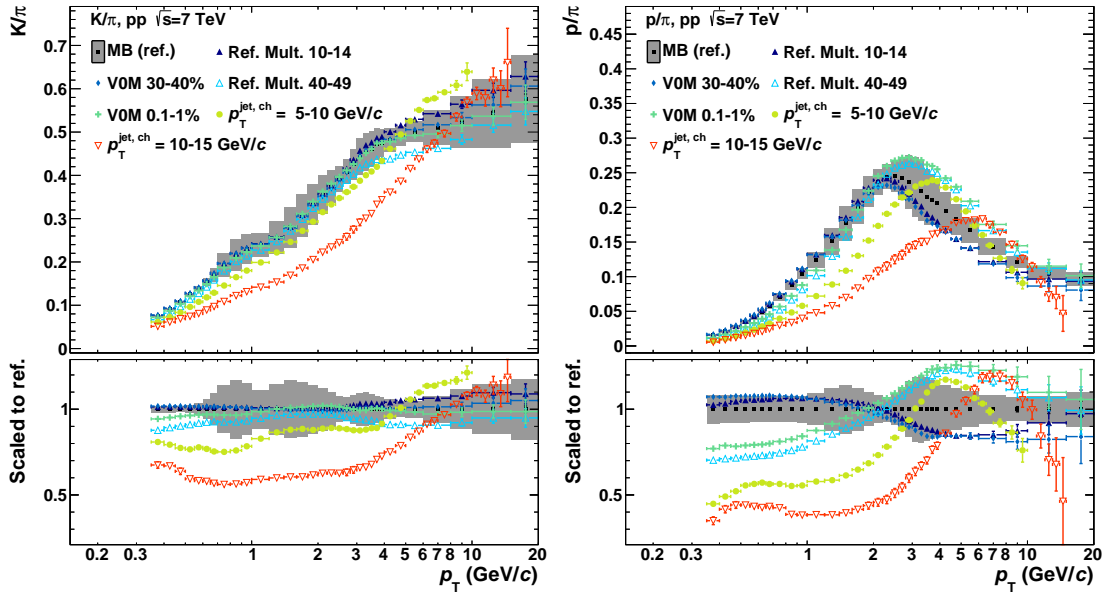
Figure 6.44.: Comparison of K/\pi (left) and p/\pi (right) for different multiplicity estimators and jets, see discussion in the text. Note that for this comparison, the conversion from pseudo-rapidity to rapidity was not applied, neither to the jet, nor to the multiplicity results. The jet results are for |\eta| < 0.9 , those for multiplicity for |\eta| < 0.8 , which should have negligible impact on this comparison.
