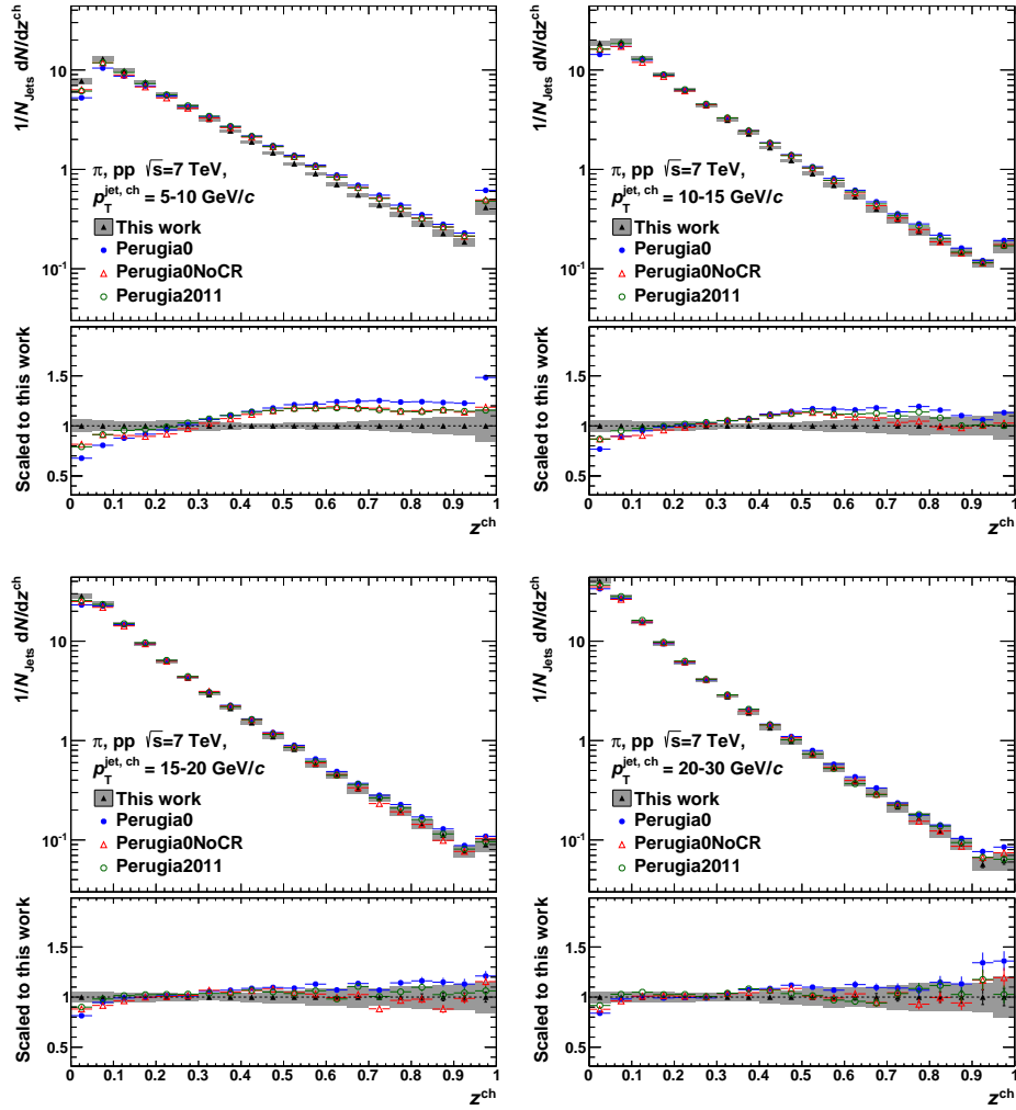
Figure K.7.: Comparison of corrected pion yields in jets to different MC predictions as a function of z . The p_T^{\text{jet}} increases from the upper left to the lower right panel.
