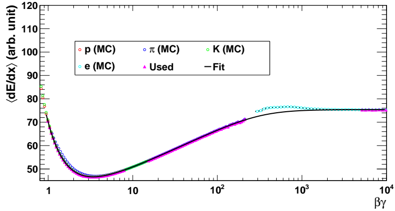
(c) Bethe-Bloch fit for MC
