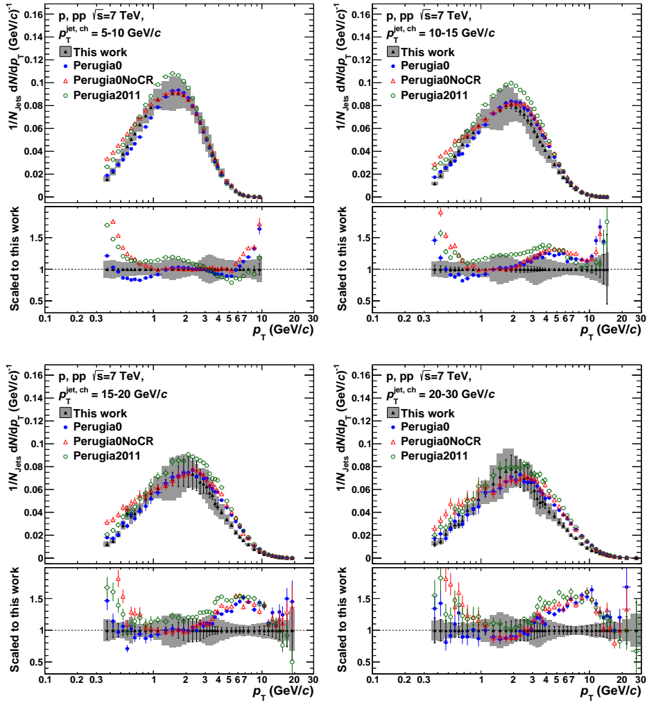
Figure 6.38.: Comparison of corrected proton yields in jets to different MC predictions as a function of p_T . The p_T^{\text{jet}} increases from the upper left to the lower right panel.
