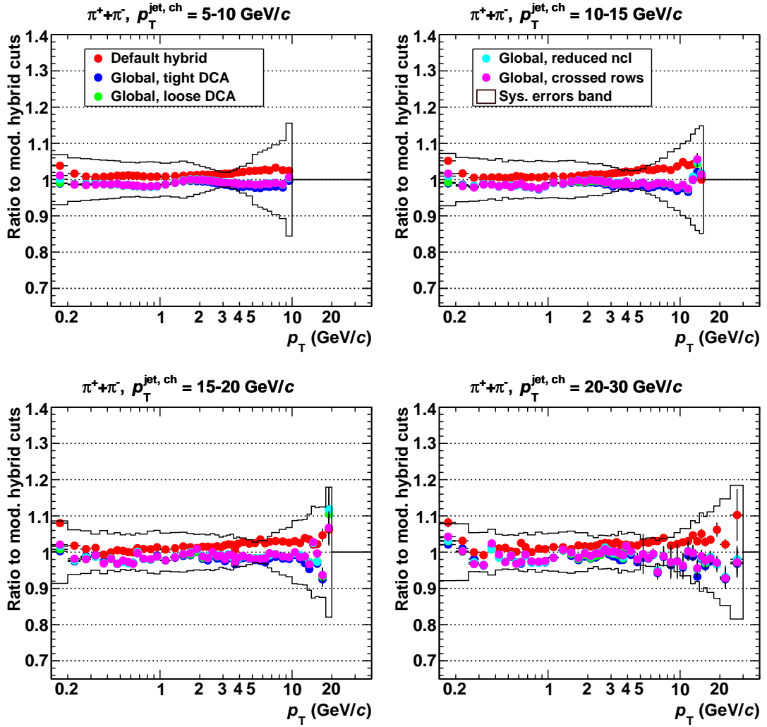
Figure 6.18.: Cut variations for pions in jets. The ratio to the modified hybrid track cuts is shown. Each set of cuts is corrected with its own MC correction factors. The systematic error band shows the total uncertainty from fit and MC corrections.
