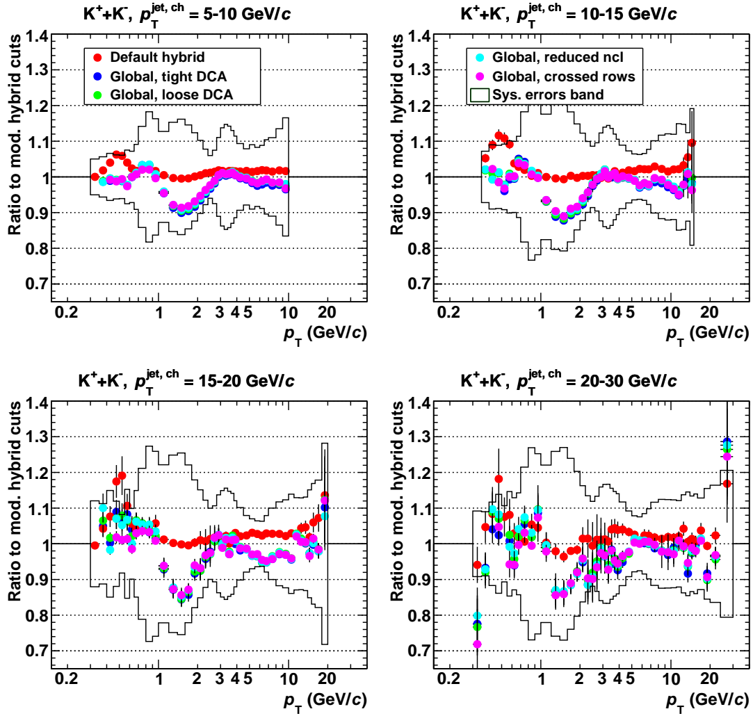
Figure 6.19.: Cut variations for kaons in jets. The ratio to the modified hybrid track cuts is shown. Each set of cuts is corrected with its own MC correction factors. The systematic error band shows the total uncertainty from fit and MC corrections.
