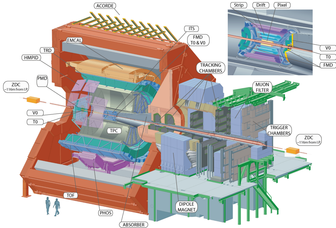
Figure 2.2.: Layout of the ALICE detector system in LHC run 1. The detector can be divided into 2 parts: the central barrel and the muon arm in forward direction. The central barrel is embedded in the L3 solenoid and consists of several subdetectors. The inset shows the ITS.
