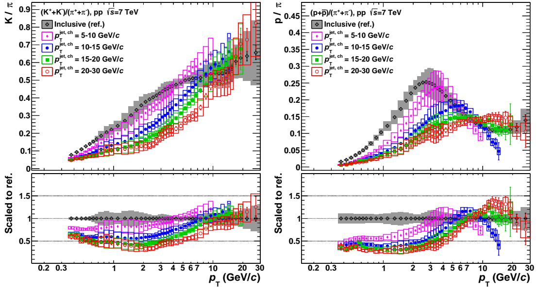
Figure 6.34.: Comparison of the corrected to-pion ratios for different p_T^{\text{jet}} in data as a function of particle p_T . The inclusive case is shown in black (open crosses). The left panel shows the kaon-to-pion and the right panel the proton-to-pion ratio.
