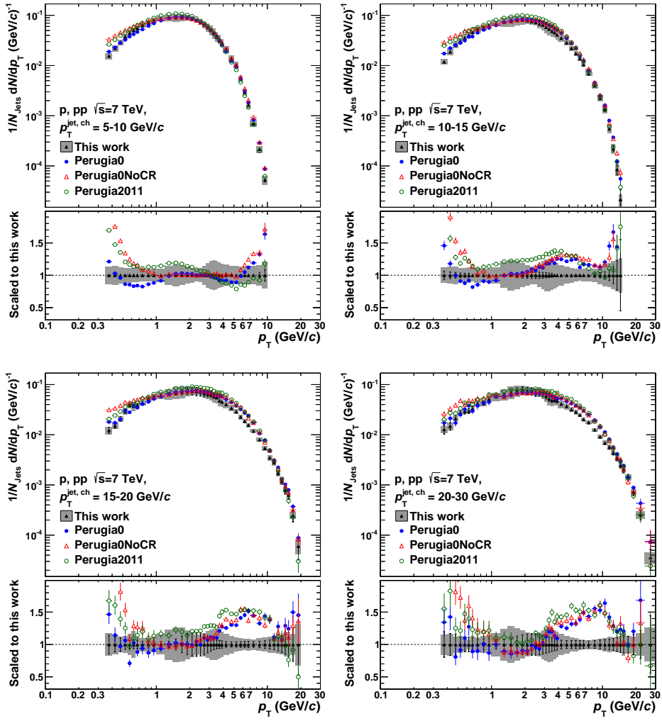
Figure K.6.: Comparison of corrected proton yields in jets to different MC predictions as a function of p_T . The p_T^{\text{jet}} increases from the upper left to the lower right panel.
