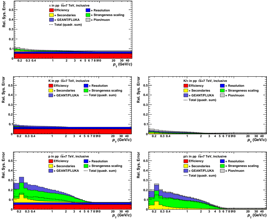
Figure 5.24.: Relative systematic uncertainties of the MC correction factors for the inclusive yields (left column) and to-pion ratios (right column) as a function of p_T^{\text{track}} . The rows show (from top to bottom) \pi , K and p, respectively.
