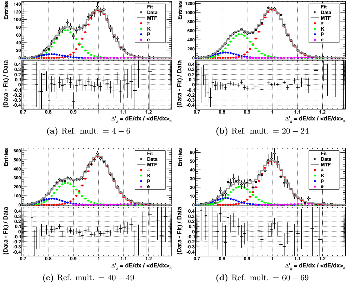
Figure F.2.: Template fits to data for different reference multiplicity bins for p_T = 8 - 10 \text{ GeV}/c . The multiplicity increases from the upper left to the lower right plot.
