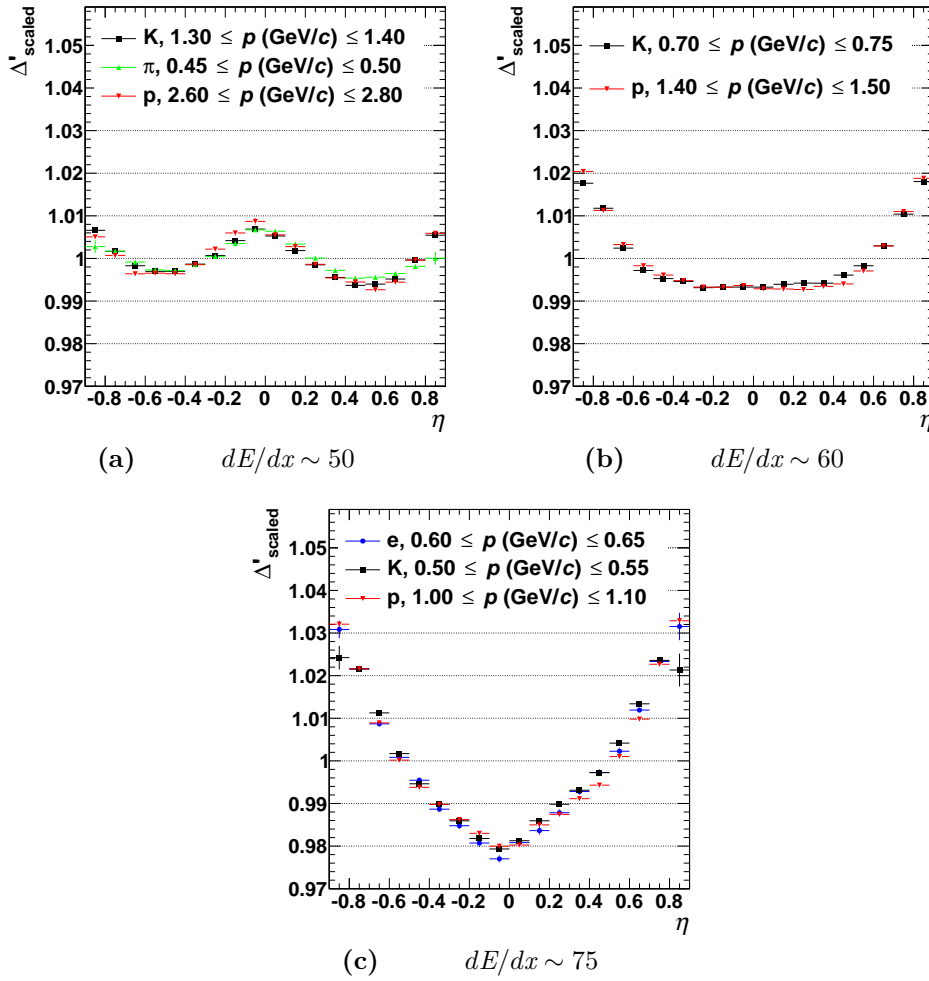
Figure 3.12.: \eta dependence of dE/dx for different species at different momenta, but similar mean dE/dx . The data points are for primary candidates selected via TPC+TOF. The ordinate shows the corresponding \Delta'_{\text{species}} scaled such that the integral equals that of a flat distribution at unity.
