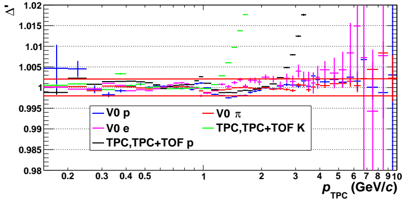
Figure 3.8.: Accuracy of the splines in data. The \Delta' on the vertical axis uses as reference the type of the corresponding species. Note that for the data points from primary particles (green and black), contamination shifts the \Delta' away from unity above some momentum threshold. The horizontal red lines show the \pm 0.2\% region around unity, which largely covers the most extreme deviations of all species.
