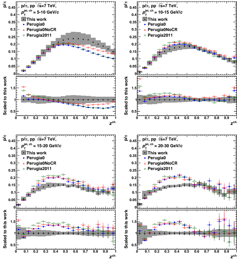
Figure K.11.: Comparison of corrected p/\pi ratios in jets to different MC predictions as a function of z . The p_T^{\text{jet}} increases from the upper left to the lower right panel.
