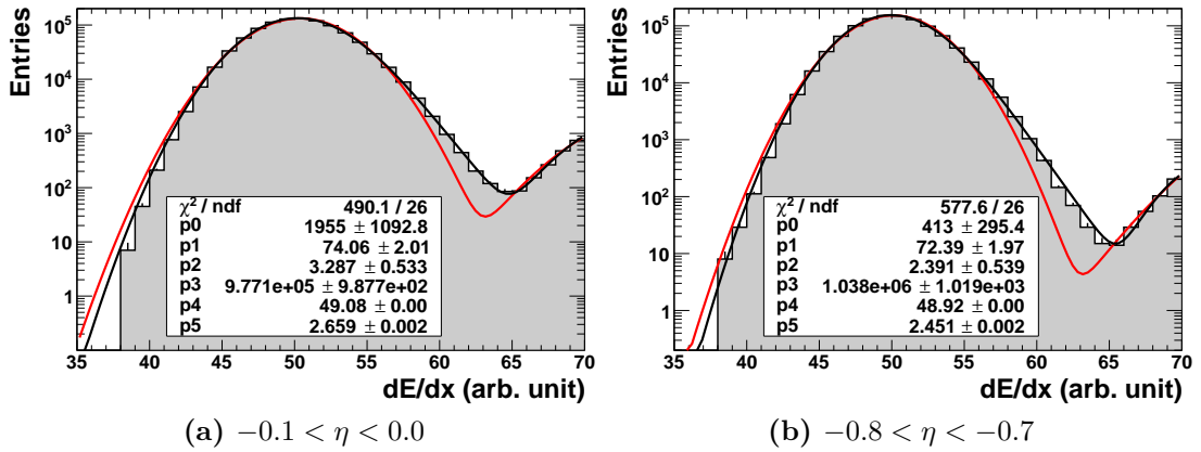
Figure 4.3.: Asymmetry of the dE/dx response around the minimum ionising region in data. The red curve is a double-Gauss fit to the data points, whereas the black curve uses the asymmetric description for the pion response. The asymmetry of the response is visible at a) small \eta as well as at b) large eta. The data points are for negative particles with p_{TPC} = 0.45 - 0.5 \text{ GeV}/c .
