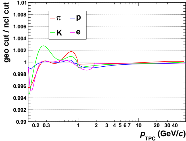
Figure 6.16.: The splines extracted from the geometrical cut sample ( geo cut ) are compared to the ones of the default ncl cut sample ( ncl cut ) in MC. Their ratio is shown as a function of momentum for the individual species. In both cases, the particle level truth was used to “identify” particles.
