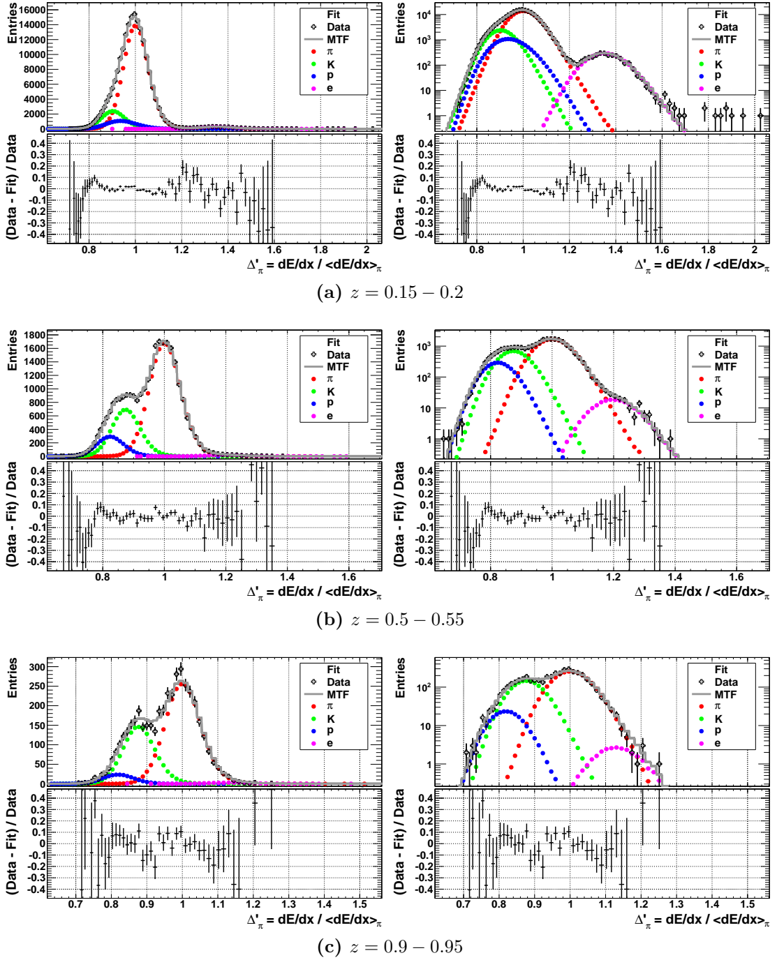
Figure F.7.: Template fits to data in different z intervals for p_T^{\text{jet}} = 10 - 15 \text{ GeV}/c . The left panel shows the plots with linear vertical axis, the right panel with logarithmic axis. The rows show (starting from the top) the following z ranges: 0.15 - 0.2 , 0.5 - 0.55 and 0.9 - 0.95 . Note the different ranges of the abscissa.
