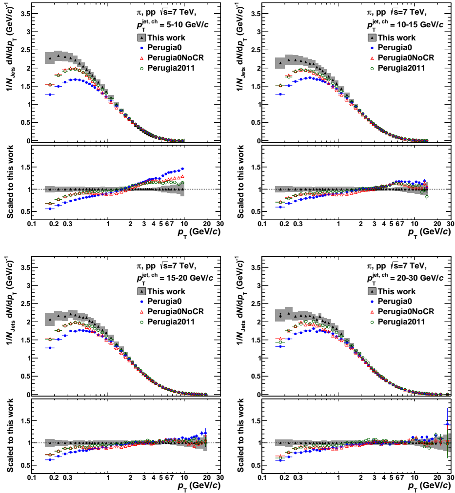
Figure 6.36.: Comparison of corrected pion yields in jets to different MC predictions as a function of p_T . The p_T^{\text{jet}} increases from the upper left to the lower right panel.
