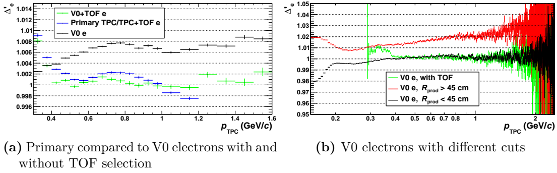
Figure 3.3.: Comparison of the mean dE/dx normalised to some common reference of primary and V0 electrons. In a) , the pure V0 selection without TOF (black) deviates from that with TOF (green), where the latter is in agreement with primary electrons (blue). The reason of the deviation is illustrated in b) , which splits the pure V0 electron sample into two sets with different cuts on the production radius R_{\text{prod}} .
