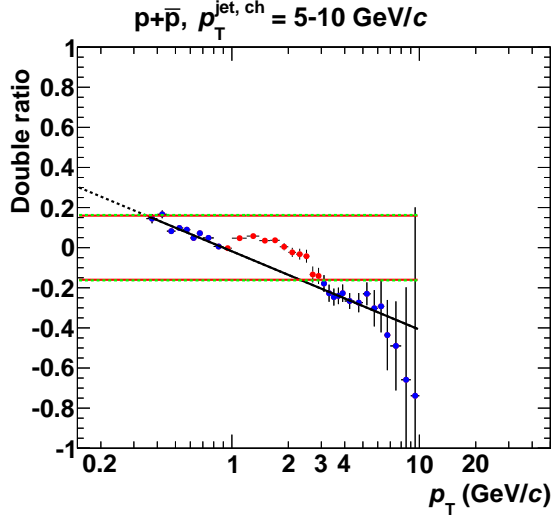
Figure 5.19.: Double ratio for protons in jets with p_T^{\text{jet, ch}} = 5 - 10 \text{ GeV}/c . The red points have been excluded from the fit. See discussion in text for further details.
