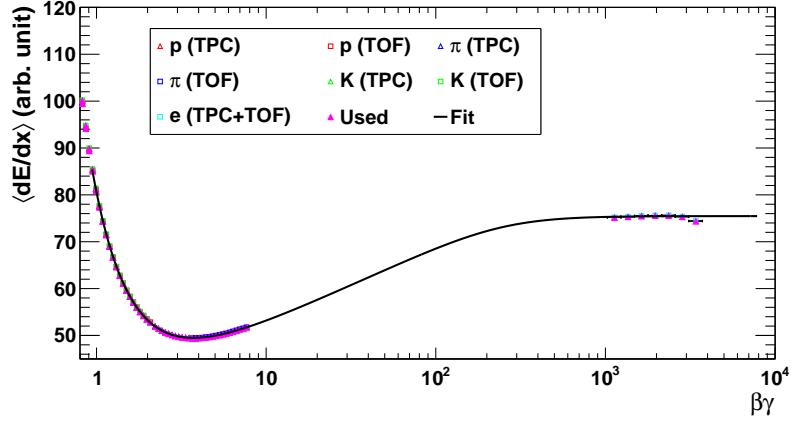
(a) Bethe-Bloch fit without V0 information
