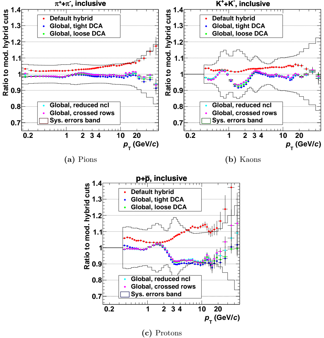
Figure I.7.: Cut variations for pions (a), kaons (b) and protons (c) in the inclusive case. The ratio to the modified hybrid track cuts is shown. Each set of cuts is corrected with its own MC correction factors. The systematic error band shows the total uncertainty from fit and MC corrections.
