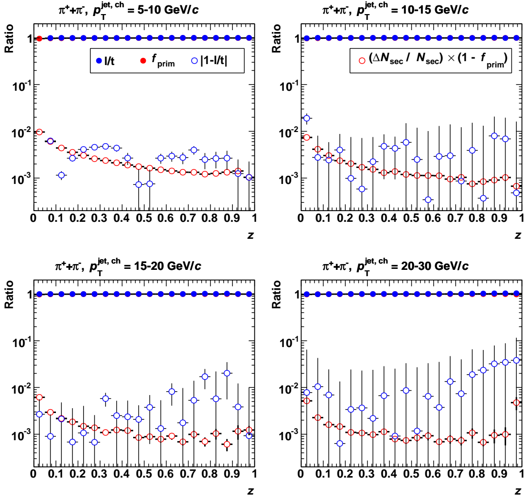
Figure E.5.: Summary plot for the systematic uncertainty estimation of the secondary correction for pions in jets as a function of z . The open red points show the relative systematic uncertainty estimate and should be compared to the open blue points, which show the relative change of spectra due to DCA cut variations.
