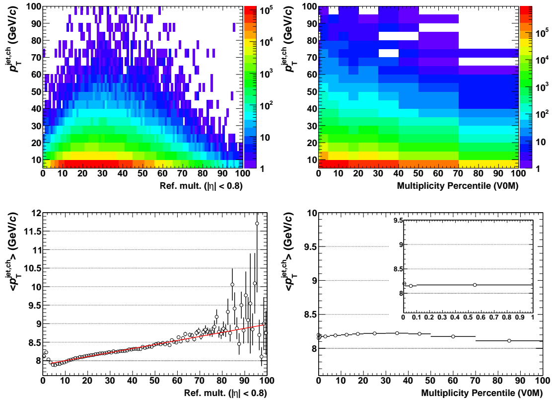
Figure 6.43.: Correlation between p_T^{\text{jet}} and multiplicity for the reference multiplicity (left) and the V0M multiplicity (right). The upper panel shows the scatter plots, the lower panel depicts the profiles of the corresponding mean p_T^{\text{jet}} in each multiplicity bin. The colour code gives the number of jets. The red line in the lower left panel is a linear fit.
