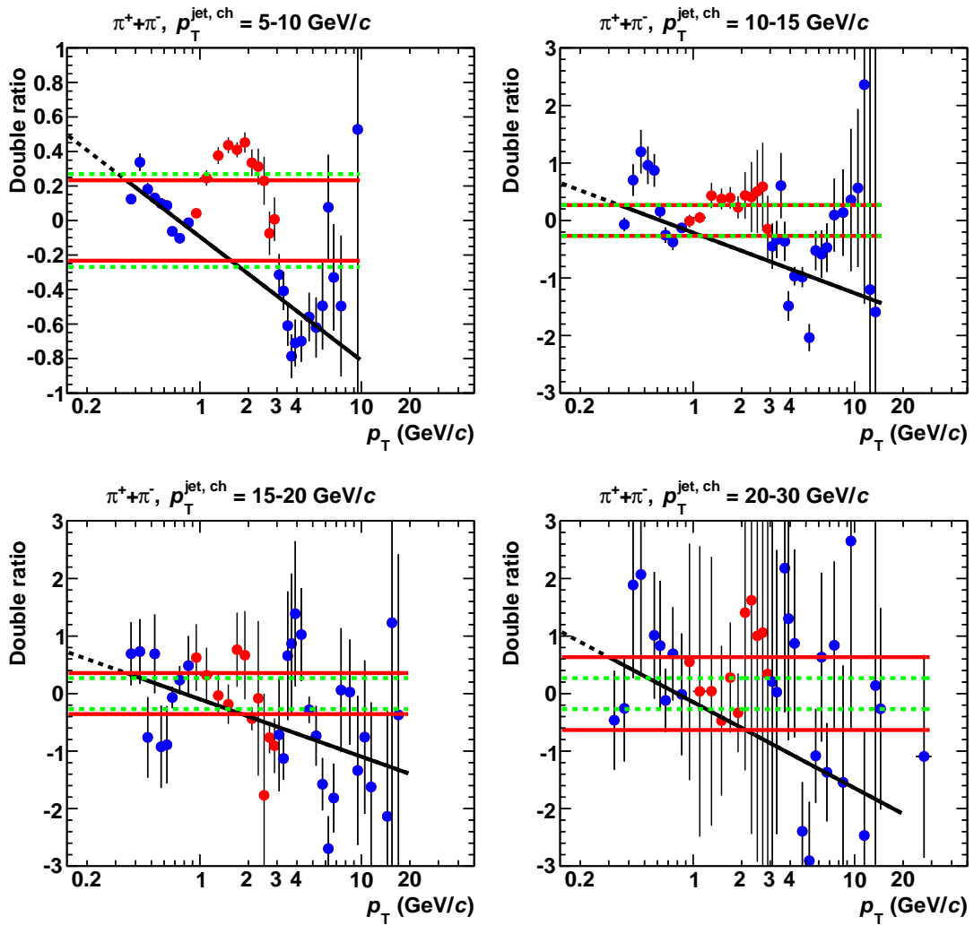
Figure 5.21.: Double ratio for pions in jets. The red points have been excluded from the fit. See discussion in the text for further details. Note the different ranges for the vertical axis.
