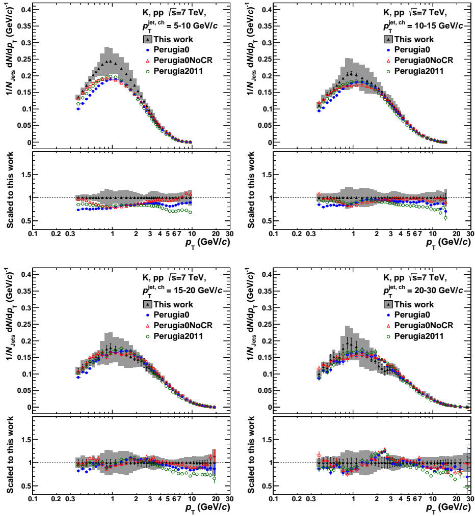
Figure 6.37.: Comparison of corrected kaon yields in jets to different MC predictions as a function of p_T . The p_T^{\text{jet}} increases from the upper left to the lower right panel.
