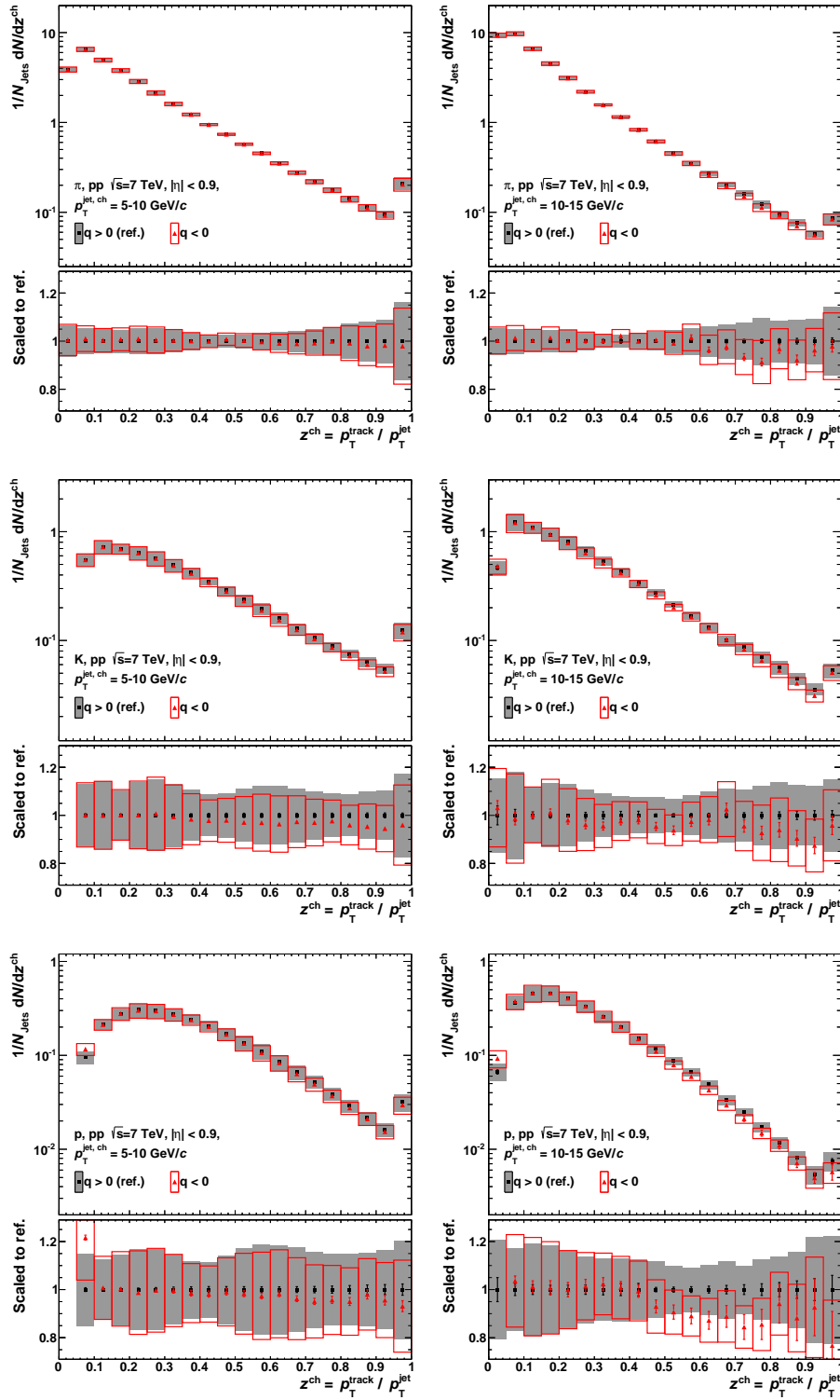
Figure 6.41.: Comparison of positively ( q > 0 ) and negatively ( q < 0 ) charged particles in jets with p_T^{\text{jet}} = 5 - 10 (left) and 10 - 15 GeV/c (right). The rows show (from top to bottom): \pi , K and p.
