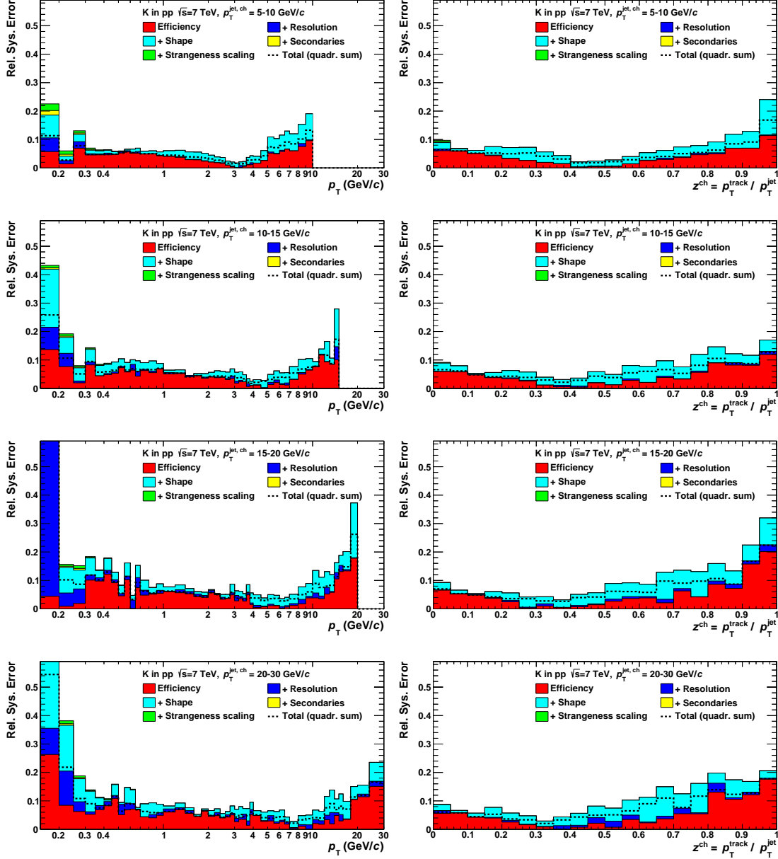
Figure E.7.: Relative systematic uncertainties of the MC correction factors for the kaon yields. The rows show (from top to bottom) p_T^{\text{jet}} = 5 - 10, 10 - 15, 15 - 20 and 20 - 30 GeV/c, respectively, as a function of p_T^{\text{track}} (left column) and z (right column).
