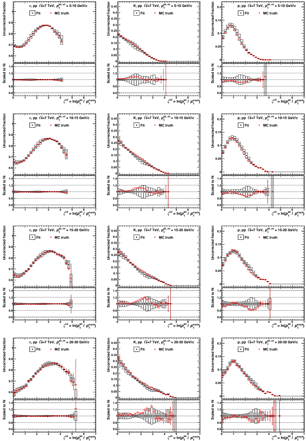
Figure D.3.: MC blind test for fitting versus \xi . The raw fractions from fitting the MC output (black) are compared to the MC truth (red) for (from left to right): pions, kaons and protons. The rows show (from top to bottom): p_T^{\text{jet}} = 5 - 10 , 10 - 15 , 15 - 20 and 20 - 30 GeV/c.
