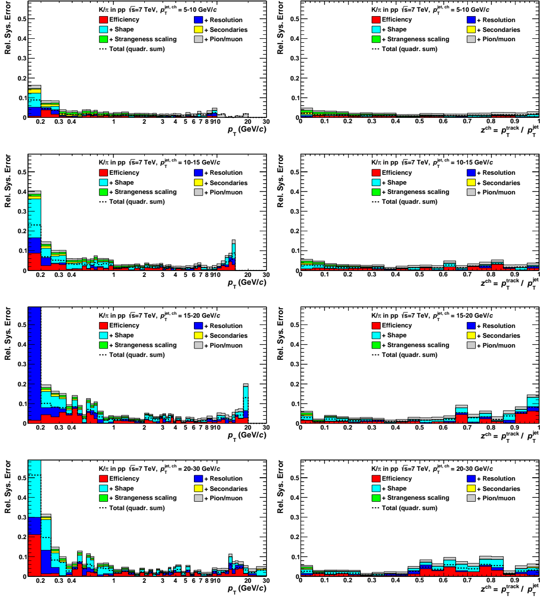
Figure E.9.: Relative systematic uncertainties of the MC correction factors for the topion ratios of kaons. The rows show (from top to bottom) p_T^{\text{jet}} = 5-10, 10-15, 15-20 and 20-30 GeV/c, respectively, as a function of p_T^{\text{track}} (left column) and z (right column).
