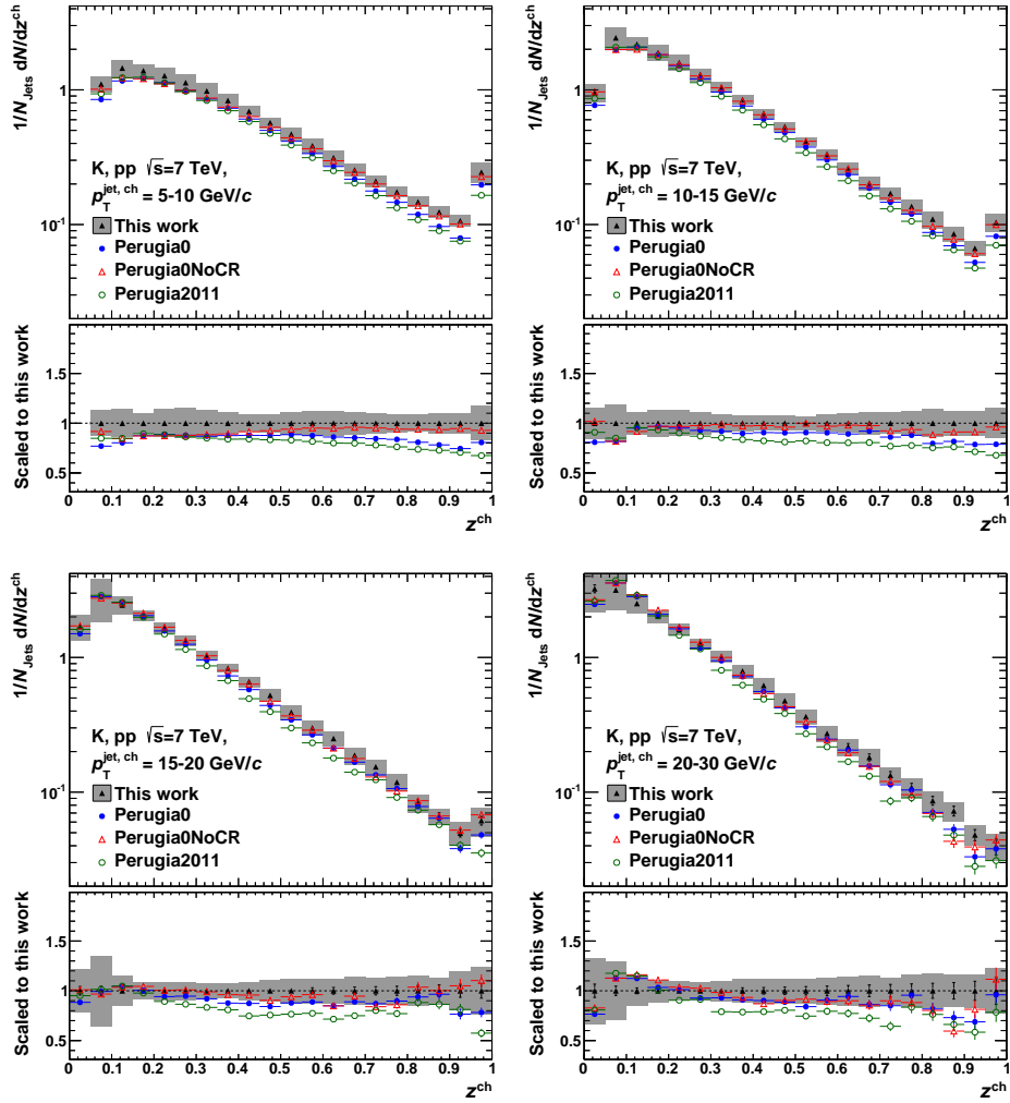
Figure K.8.: Comparison of corrected kaon yields in jets to different MC predictions as a function of z . The p_T^{\text{jet}} increases from the upper left to the lower right panel.
