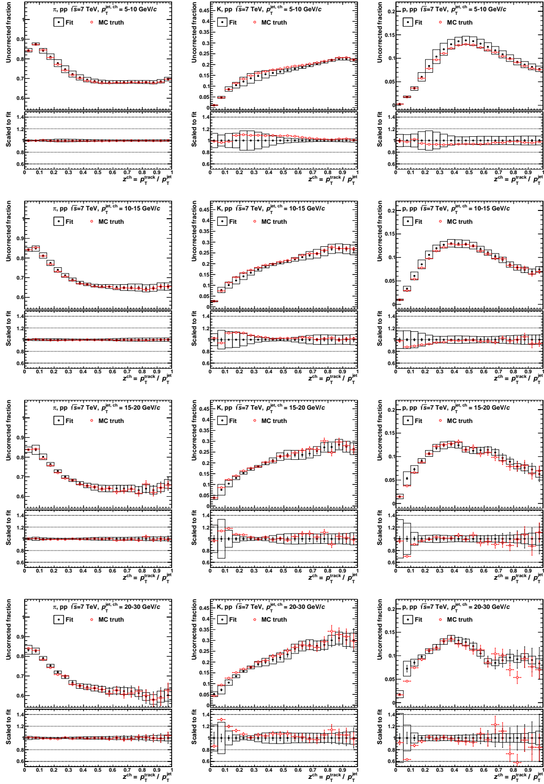
Figure D.2.: MC blind test for fitting versus z . The raw fractions from fitting the MC output (black) are compared to the MC truth (red) for (from left to right): pions, kaons and protons. The rows show (from top to bottom): p_T^{\text{jet}} = 5 - 10 , 10 - 15 , 15 - 20 and 20 - 30 GeV/ c .
