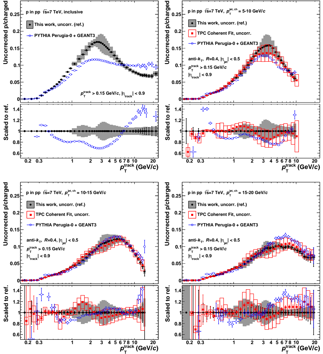
Figure 6.6.: Comparison of uncorrected proton fractions as a function of p_T to the TPC Coherent Fit. In addition, the MC prediction from PYTHIA Perugia-0 is overlaid. Note that there are no results from the TPC Coherent Fit for the inclusive case.
