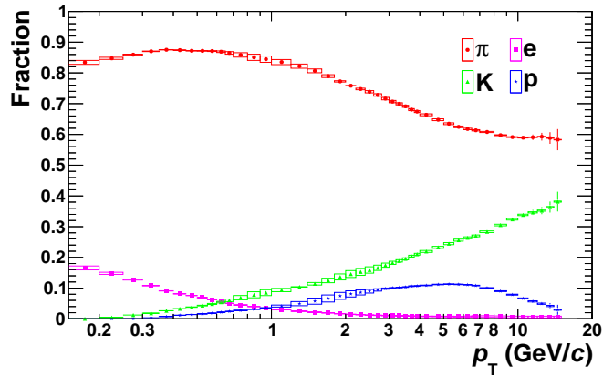
Figure 6.10.: The uncorrected particle fractions are shown for particles in jets with p_T^{\text{jet}} = 10\text{--}15\text{ GeV}/c in data. The boxes show the systematic error due to uncertainties of the shape of the dE/dx response.
