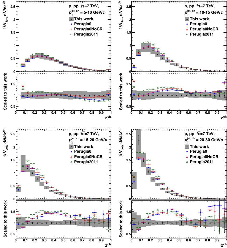
Figure K.3.: Comparison of corrected proton yields in jets to different MC predictions as a function of z . The p_{\text{T}}^{\text{jet}} increases from the upper left to the lower right panel.
