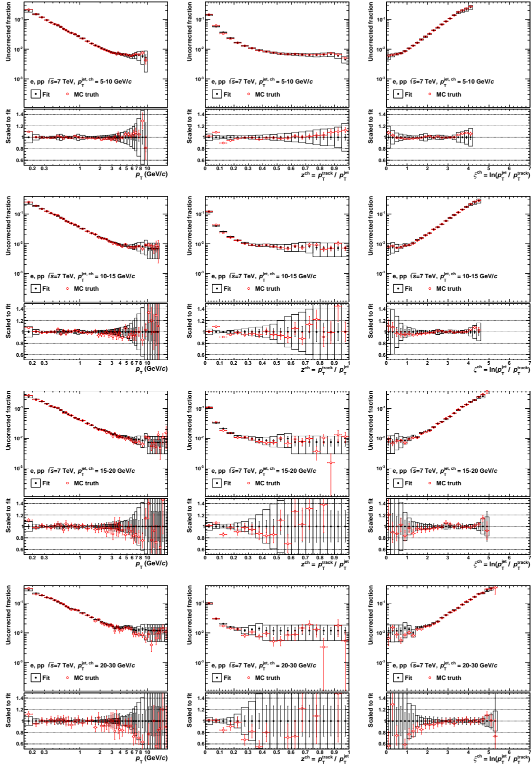
Figure D.4.: MC blind test for electrons in jets. The raw fractions from fitting the MC output (black) are compared to the MC truth (red) for fitting versus (from left to right): p_T , z and \xi . The rows show (from top to bottom): p_T^{\text{jet}} = 5 - 10 , 10 - 15 , 15 - 20 and 20 - 30 GeV/c.
