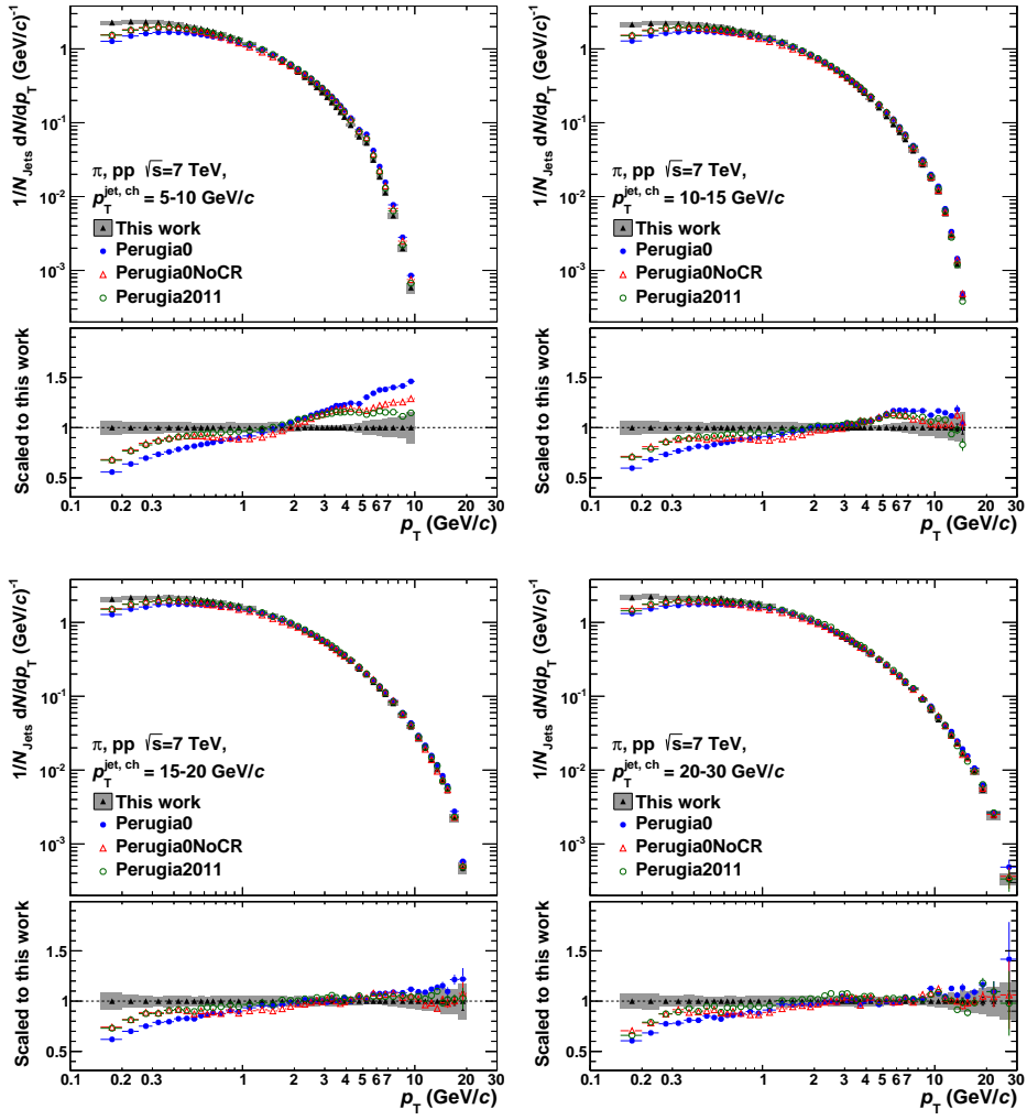
Figure K.4.: Comparison of corrected pion yields in jets to different MC predictions as a function of p_T . The p_T^{\text{jet}} increases from the upper left to the lower right panel.
