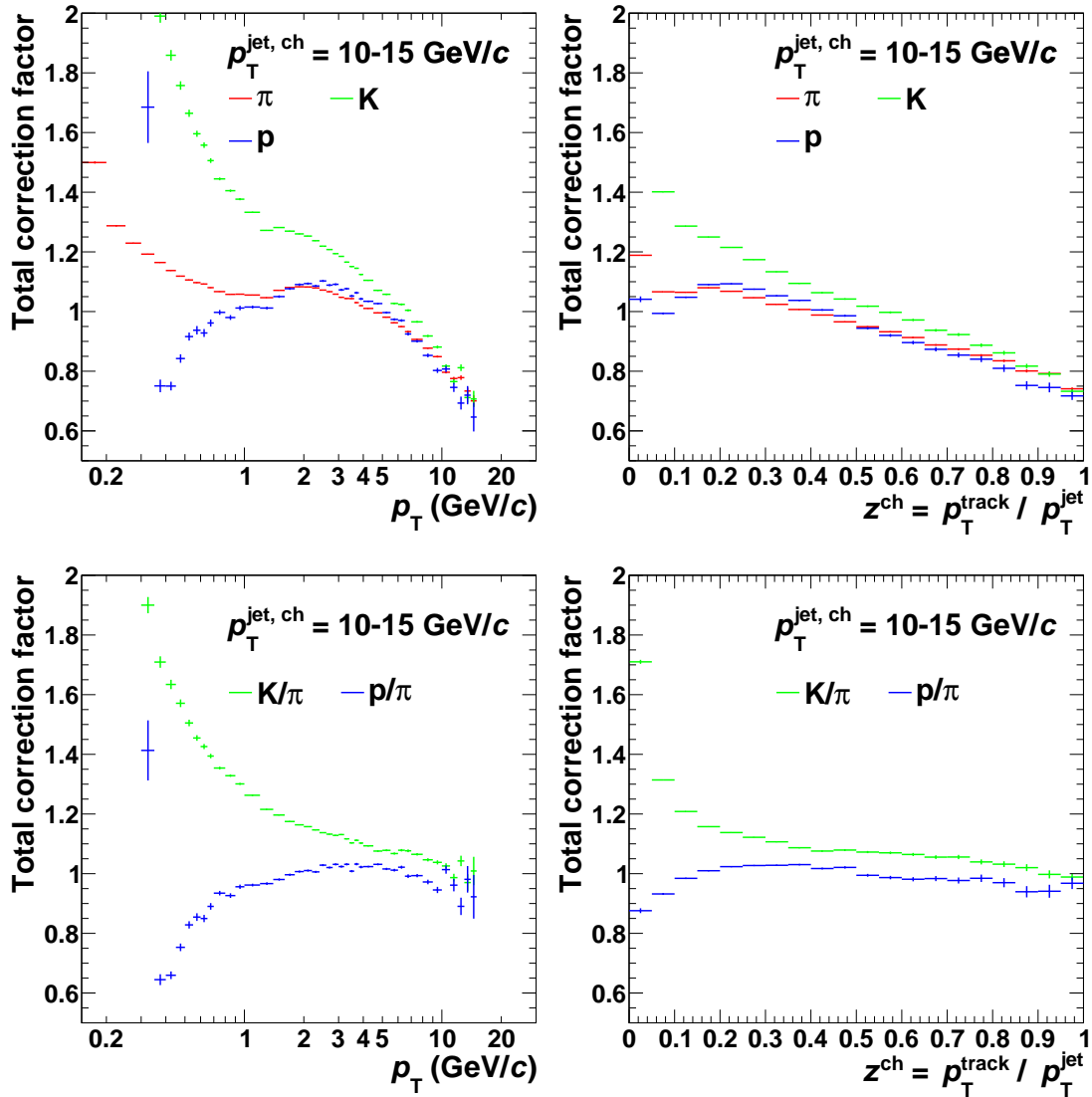
Figure 5.5.: Combined MC correction factors for the yields (top row) and to-pion ratios (bottom row) in jets with p_T^{\text{jet}} = 10 - 15 \text{ GeV}/c as a function of p_T^{\text{track}} (left) and z (right).
