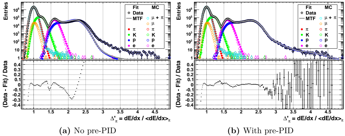
Figure 4.1.: Template generation and fit quality in MC a) without and b) with using pre-PID. In the upper panels, the dE/dx distribution for p_T = 0.6 - 0.65 \text{ GeV}/c is shown in black together with the templates (full points), the MC true response (open points) and the fit (grey line). The lower panels show the relative deviation of the fit from data.
