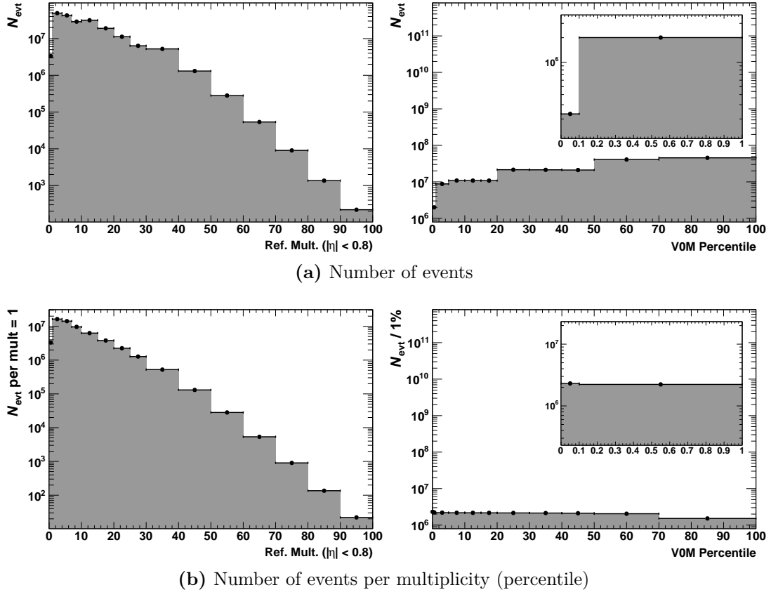
Figure 6.24.: Number of events after all selections as a function of the reference multiplicity (left) and the V0M percentile (right). Note that no normalisation to the bin width is applied in (a), which causes jumps in the histograms. After normalising to the bin width (b), the distribution for the V0M percentile is largely flat. Also note that the horizontal axis in the left panel shows the multiplicity and not a percentile, i.e. low percentiles correspond to high multiplicities.
