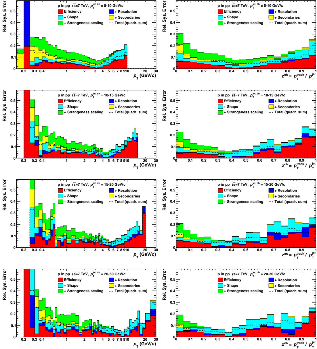
Figure E.8.: Relative systematic uncertainties of the MC correction factors for the proton yields. The rows show (from top to bottom) p_T^{\text{jet}} = 5 - 10, 10 - 15, 15 - 20 and 20 - 30 GeV/c, respectively, as a function of p_T^{\text{track}} (left column) and z (right column).
