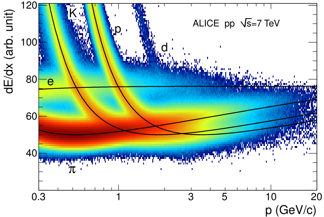
Figure 3.1.: Specific energy loss dE/dx of tracks in the ALICE TPC. The black lines are fits with a Bethe-Bloch parametrisation to the individual particle species.
