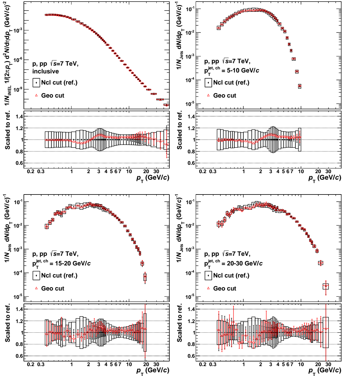
Figure I.3.: Comparison of the corrected proton yields for the TPC geometrical cut (red open triangles) and the ncl cut (black diamonds) versus p_T^{\text{track}} in data. Each set of cuts is corrected with its own MC correction factors. The boxes correspond to the systematic errors for the ncl cut, including the uncertainties of the corresponding MC correction factors.
