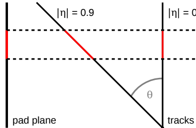
Figure 3.11.: Influence of the local polar angle \theta on the effective track length per pad.
