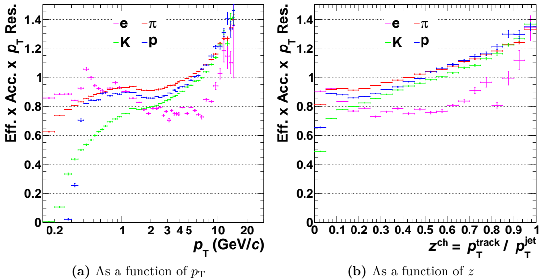
Figure 5.1.: The (inverse) efficiency \times acceptance \times p_T resolution correction factors for particles in jets with p_T^{\text{jet}} = 10 - 15 \text{ GeV}/c for both charges are shown as a function of a) p_T and b) z . The impact of the p_T resolution is discussed in the text.
