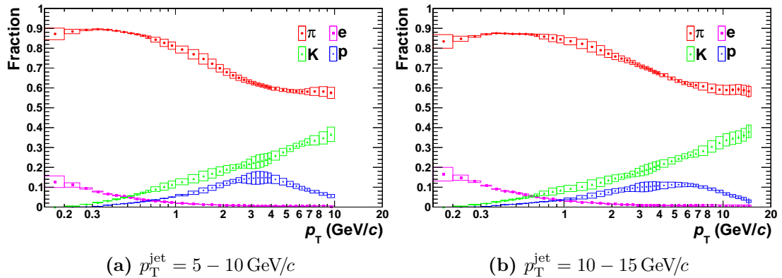
Figure 6.1.: The uncorrected particle fractions are shown for particles in jets with p_T^{\text{jet}} = 5 - 10 (a) and 10 - 15 \text{ GeV}/c (b) in data. The boxes show the total systematic uncertainty.
