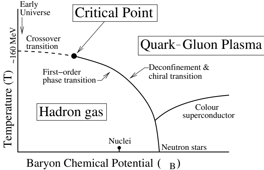
Figure 1.2.: QCD phase diagram with the temperature on the ordinate and the baryon chemical potential, which is directly connected to the baryon density, on the abscissa. Figure from [21].
