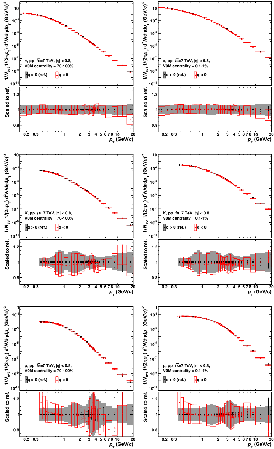
Figure 6.31.: Comparison of positively ( q > 0 ) and negatively ( q < 0 ) charged particles for the V0M multiplicity bins 70 – 100% (left) and 0.1 – 1% (right). The rows show (from top to bottom): \pi , K and p.
