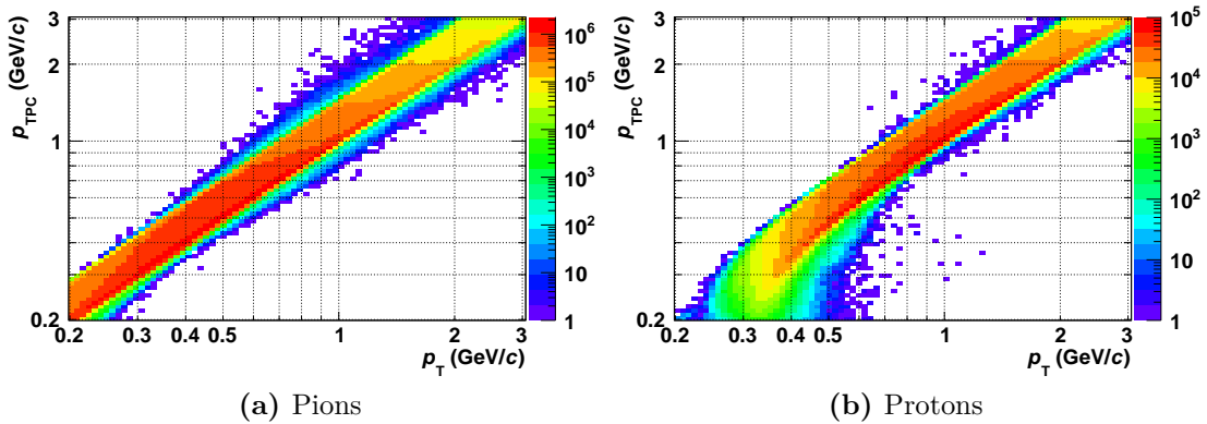
Figure 4.2.: Correlation between transverse momentum, p_T , and the momentum at the TPC inner wall, p_{\text{TPC}} , for a) pions and b) protons in MC. The MC label was used to determine the particle species. The colour code shows the number of accepted tracks within |\eta| < 0.9 .
