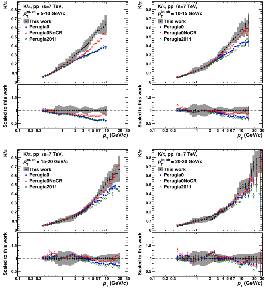
Figure 6.39.: Comparison of corrected K/\pi ratios in jets to different MC predictions as a function of p_T . The p_T^{\text{jet}} increases from the upper left to the lower right panel.
