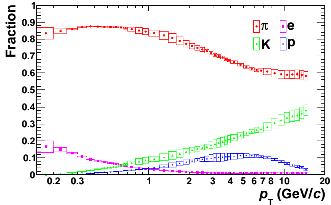
Figure 6.13.: The uncorrected particle fractions are shown for particles in jets with p_T^{\text{jet}} = 10 - 15 \text{ GeV}/c in data. The boxes show the total systematic error as the quadratic sum of all sources.
