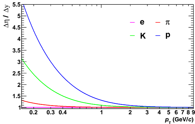
Figure 6.22.: Comparison of the normalisation factors for rapidity ( \Delta y ) and pseudo-rapidity ( \Delta\eta = 2 \cdot 0.8 = 1.6 ). The ratio \Delta\eta/\Delta y is the conversion factor to change the normalisation of the yields from pseudo-rapidity to rapidity. In the relevant p_T range, p_T > 0.15 GeV/ c , the conversion factor is unity for electrons, smaller than 1.4 for pions and can go up to 5.5 for protons. It drops rapidly with increasing p_T and approaches unity for all species around p_T = 6 GeV/ c .
