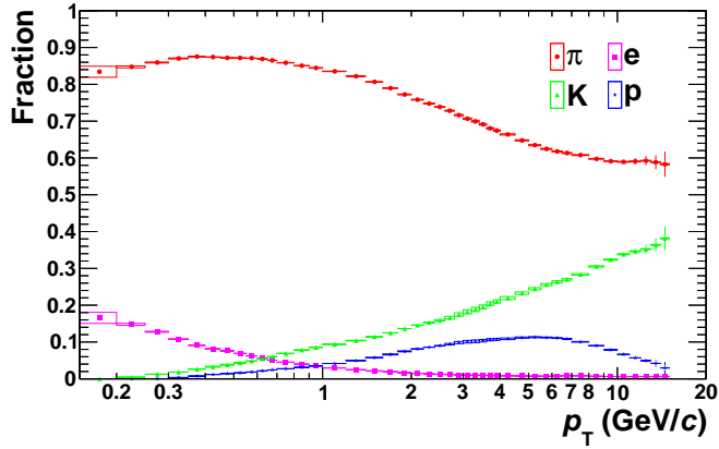
Figure 6.11.: The uncorrected particle fractions are shown for particles in jets with p_T^{\text{jet}} = 10\text{--}15\text{ GeV}/c in data. The boxes show the systematic error due to uncertainties of the PID weighting.
