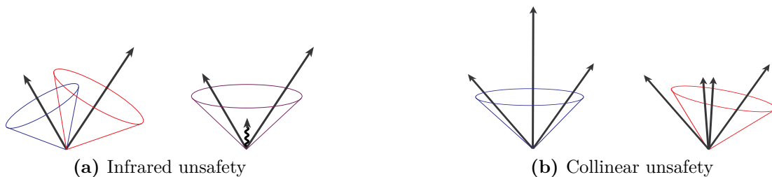
Figure 2.7.: Illustration of an infrared and collinear unsafe jet finder. The result of the jet finding is changed if a) an arbitrarily soft particle (curly line) is added (infrared unsafe) or b) the leading track is split into two collinear tracks with similar momenta (collinear unsafe), cf. discussion in the text. Figure from [93].
