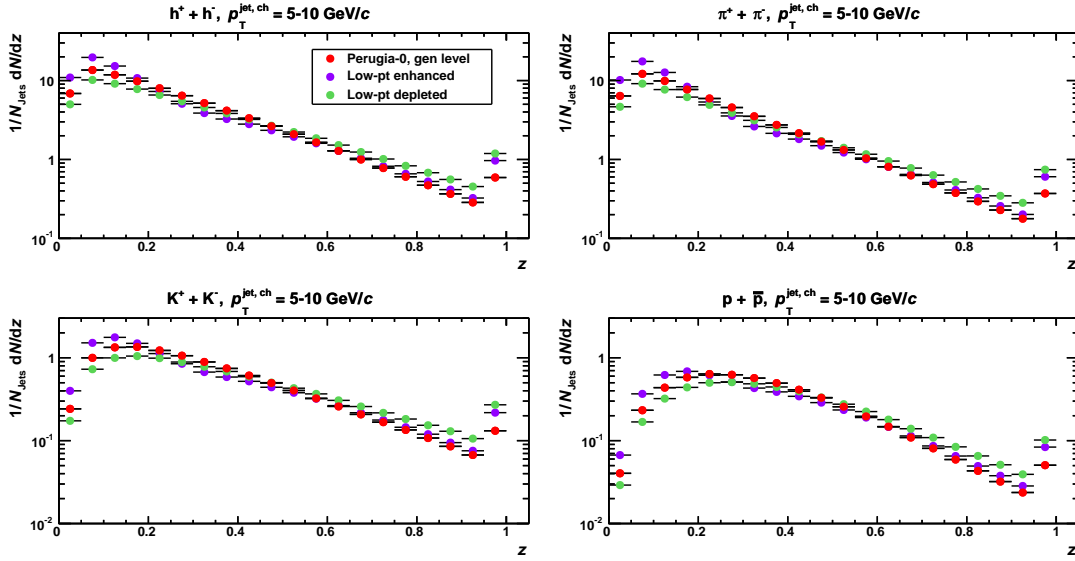
Figure 5.16.: Modified fragmentation distributions (green and violet) are compared to the case without modifications (red). The comparison is shown for all charged particles, \pi , K and p in jets with p_T^{\text{jet}} = 5 - 10 \text{ GeV}/c .
