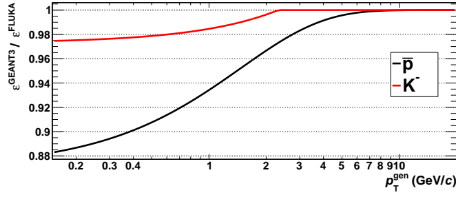
Figure 5.6.: GEANT-FLUKA correction factors for the efficiency of anti-protons (black) and negative kaons (red).
