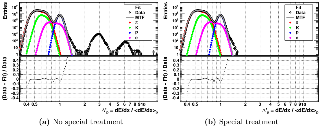
Figure 4.6.: Demonstration of the special treatment of light nuclei: in a) , no special treatment is applied to light nuclei, whereas in b) , light nuclei are rejected if safely possible and remainders contribute differently to the templates. The plots are for data and show tracks with p_{\text{T}}^{\text{track}} = 0.7 - 0.8 \text{ GeV}/c .
