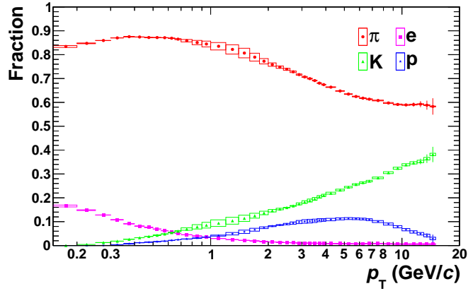
Figure 6.9.: The uncorrected particle fractions are shown for particles in jets with p_T^{\text{jet}} = 10\text{--}15\text{ GeV}/c in data. The boxes show the systematic error due to uncertainties of the resolution.
