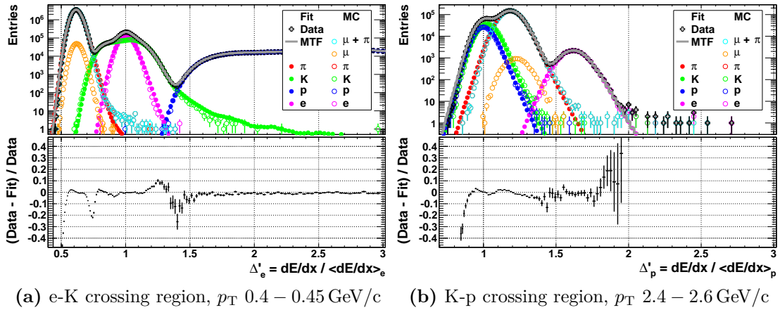
Figure 4.10.: Comparison of templates in the a) e-K and b) K-p crossing regions for MC. The full points are the generated templates, the open points indicate the dE/dx distribution of the MC truth. The crossing of e and K is steep and the templates are correspondingly very different, whereas the K and p templates look similar for the flat K-p crossing. Note the different \Delta'_{\text{species}} on the abscissa. Also note that the deviations from zero in the lower panels are restricted to the edges of the pion distribution (a) and of the kaon and proton distributions (b), respectively. Their impact on the integral of the distribution and, thus, the fitted fractions is negligible.
