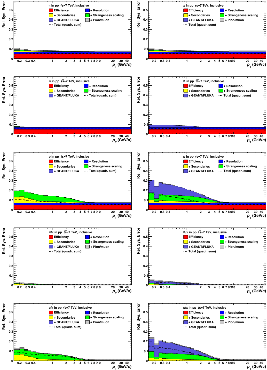
Figure 5.26.: Relative systematic uncertainties of the MB MC correction factors in the multiplicity analysis. The left column is for positively, the right column for negatively charged particles. The rows show (from top to bottom): pions, kaons, protons, K/ \pi and p/ \pi .
