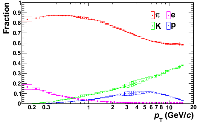
Figure 6.8.: The uncorrected particle fractions are shown for particles in jets with p_T^{\text{jet}} = 10\text{--}15\text{ GeV}/c in data. The boxes show the systematic error due to uncertainties of the \eta correction.
