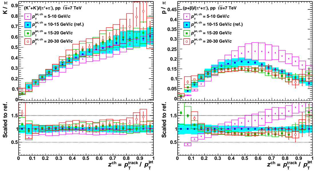
Figure 6.35.: Comparison of the corrected to-pion ratios for different p_T^{\text{jet}} in data as a function of z . The left panel shows the kaon-to-pion and the right panel the proton-to-pion ratio.
