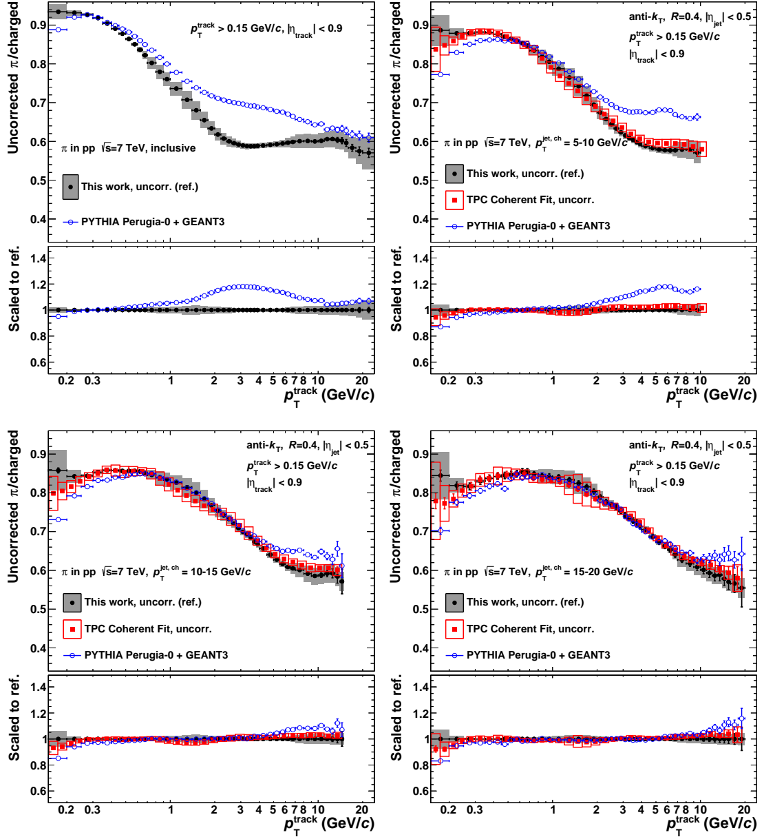
Figure 6.4.: Comparison of uncorrected pion fractions as a function of p_T to the TPC Coherent Fit. In addition, the MC prediction from PYTHIA Perugia-0 is overlaid. Note that there are no results from the TPC Coherent Fit for the inclusive case.
