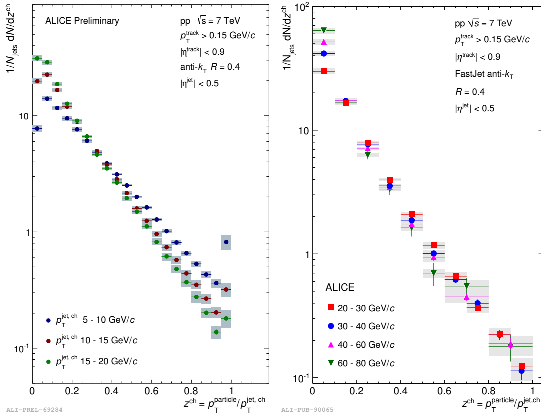
Figure 6.42.: ALICE measurement of charged particle yields in charged jets as a function of z . The left panel shows lower p_{\text{T}}^{\text{jet}} bins complementary to the right panel. Note that the left plot is for inclusive jets without subtraction of the underlying event [124], whereas the right plot shows leading jet results after underlying event subtraction [34].
