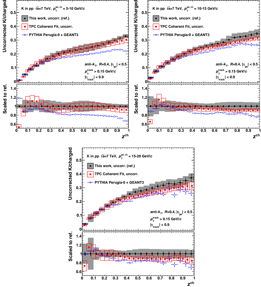
Figure H.2.: Comparison of uncorrected kaon fractions as a function of z to the TPC Coherent Fit. In addition, the MC prediction from PYTHIA Perugia-0 is overlaid.
