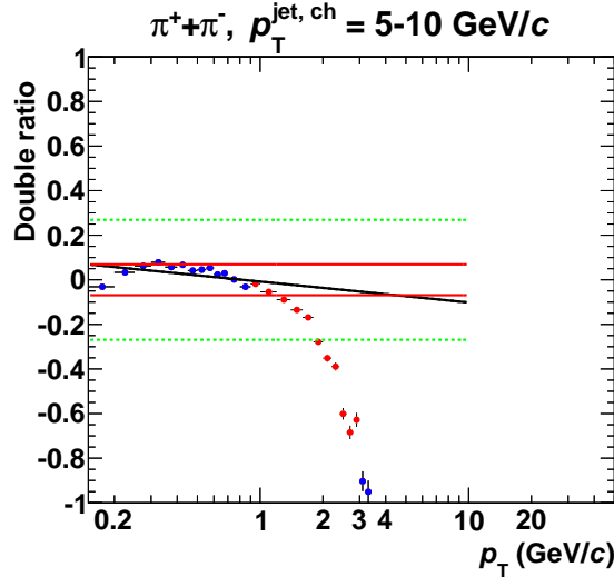
Figure E.1.: Double ratio for pions in jets with p_T^{\text{jet}} = 5 - 10 \text{ GeV}/c without applying the kaon correction. The red points have been excluded from the fit.
