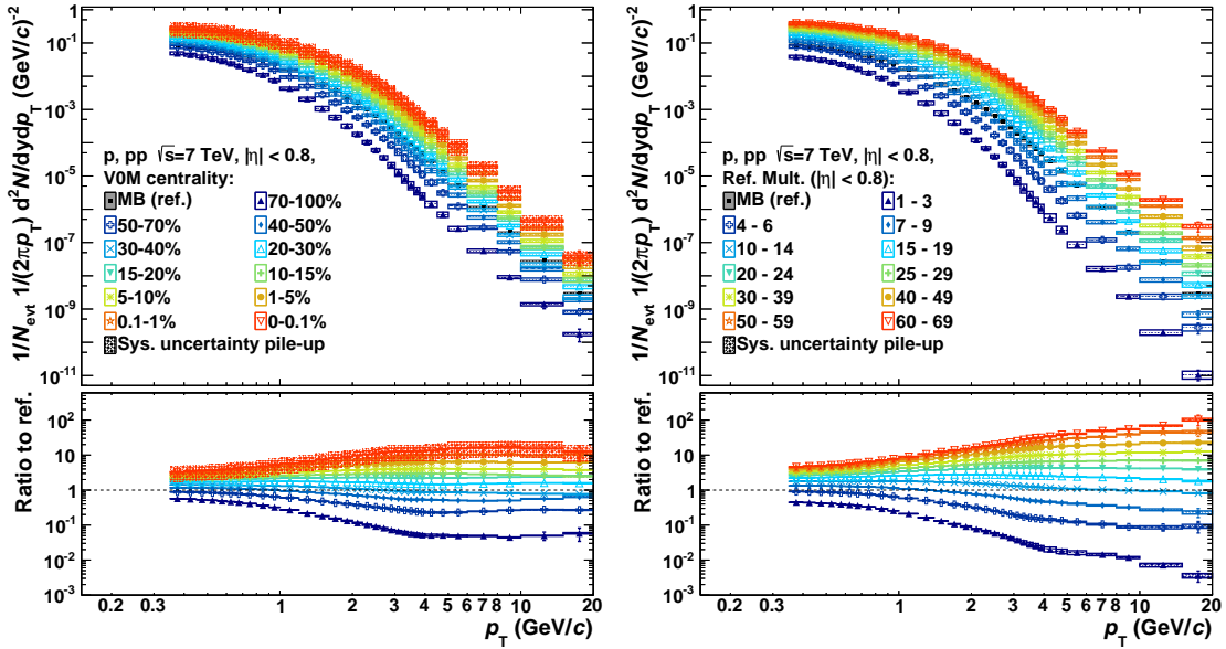
Figure 6.28.: p spectra for different bins of V0M (left) and reference multiplicity (right). The lower panels show the ratio to MB. Note that the MB data points are normalised to N_{\text{evt}}(\text{INEL}) instead of N_{\text{evt}}(\text{MB} \& \text{Vtx} \& \text{Zvtx}) .
