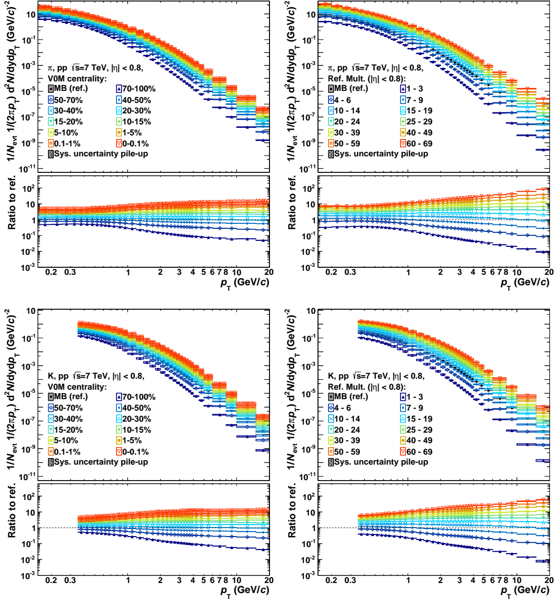
Figure 6.27.: \pi (top) and K (bottom) spectra for different bins of VOM (left) and reference multiplicity (right). The lower panels show the ratio to MB. Note that the MB data points are normalised to N_{\text{evt}}(\text{INEL}) instead of N_{\text{evt}}(\text{MB} \& \text{Vtx} \& \text{Z}_{\text{vtx}}) .
