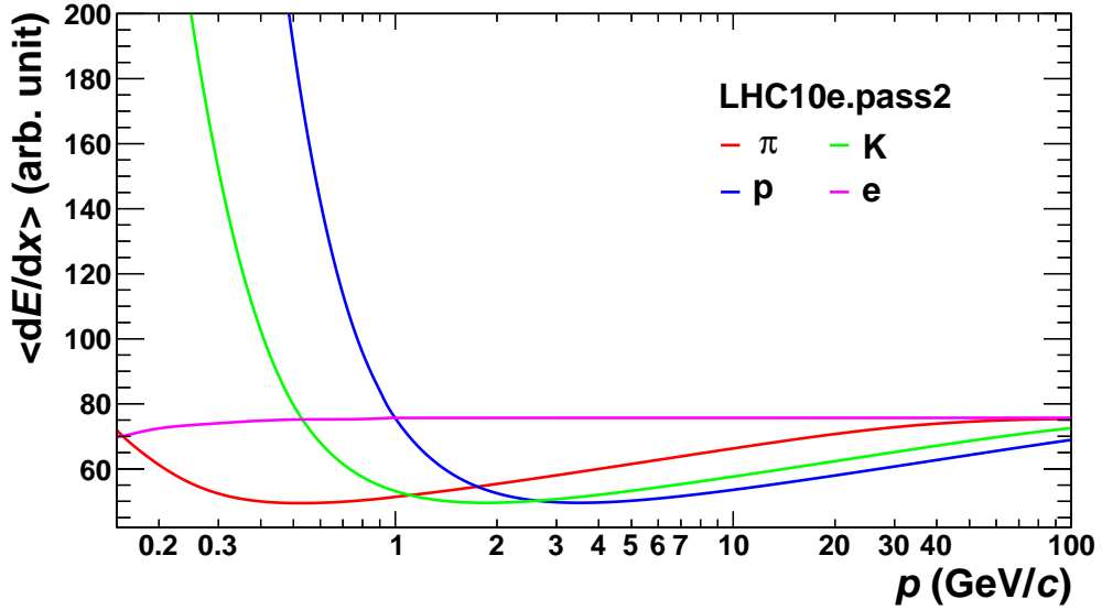
Figure 3.18.: Limitations of statistical PID with the ALICE TPC. The plot shows the mean dE/dx parametrisations extracted for the LHC10e period of the 2010 pp data taking with \sqrt{s} = 7 TeV. Around p = 40 - 50 GeV/ c , the curves for electrons and pions get close to each other, making a (statistical) identification impossible. The same holds for the (statistical) identification of pions and kaons at p \sim 100 GeV/ c .
