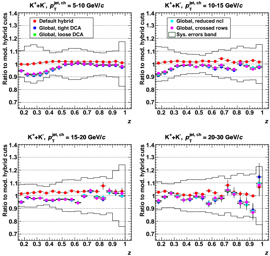
Figure I.5.: Cut variations for kaons in jets as a function of z . The ratio to the modified hybrid track cuts is shown. Each set of cuts is corrected with its own MC correction factors. The systematic error band shows the total uncertainty from fit and MC corrections.
