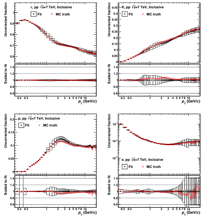
Figure D.1: MC blind test for the inclusive particle production. The raw fractions from fitting the MC output (black) are compared to the MC truth (red) for (from upper left to lower right): pions, kaons, protons and electrons.
