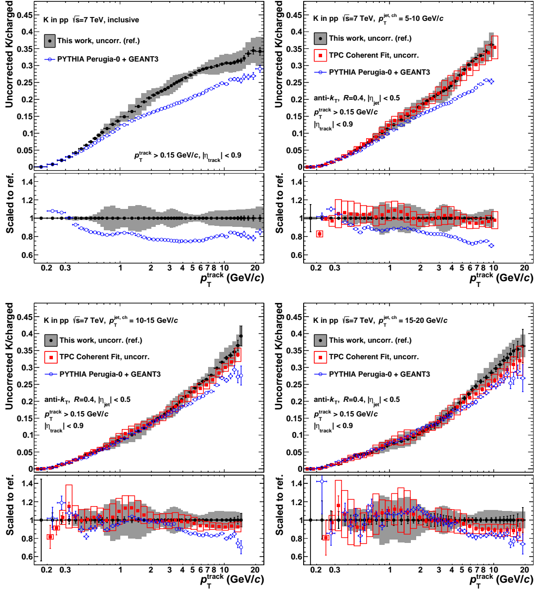
Figure 6.5.: Comparison of uncorrected kaon fractions as a function of p_T to the TPC Coherent Fit. In addition, the MC prediction from PYTHIA Perugia-0 is overlaid. Note that there are no results from the TPC Coherent Fit for the inclusive case.
