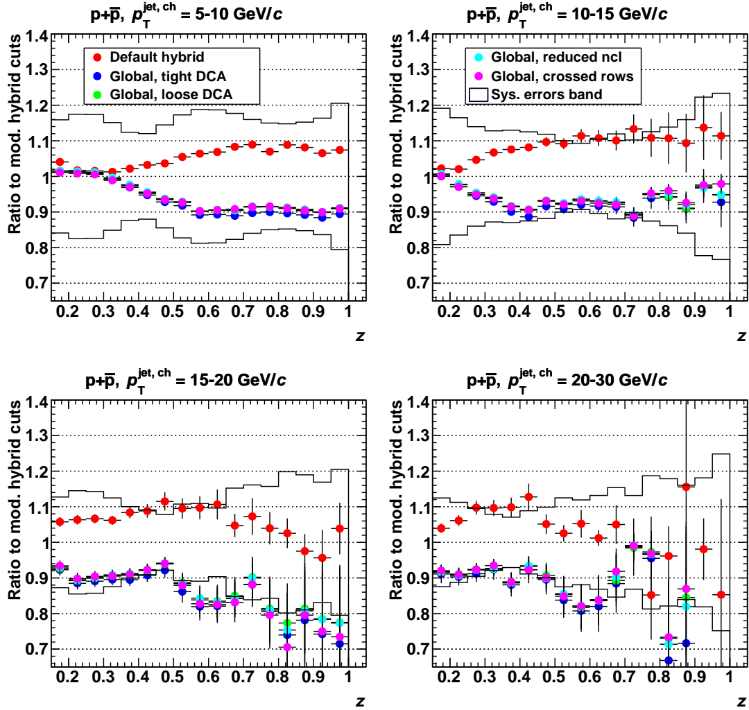
Figure I.6.: Cut variations for protons in jets as a function of z . The ratio to the modified hybrid track cuts is shown. Each set of cuts is corrected with its own MC correction factors. The systematic error band shows the total uncertainty from fit and MC corrections.
