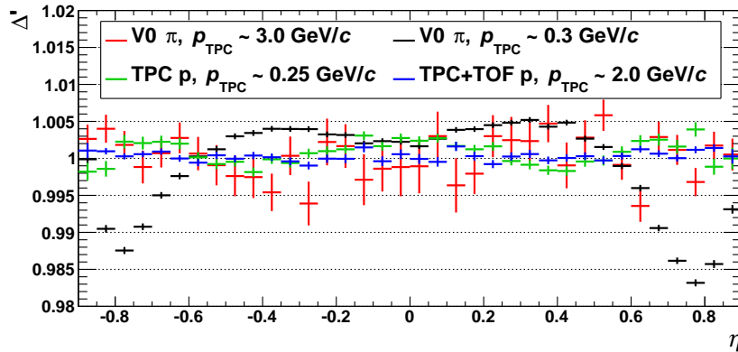
Figure 3.14.: \eta -map quality for different species at various momenta. The vertical axis is the dE/dx divided by the expected dE/dx for the corresponding species.
