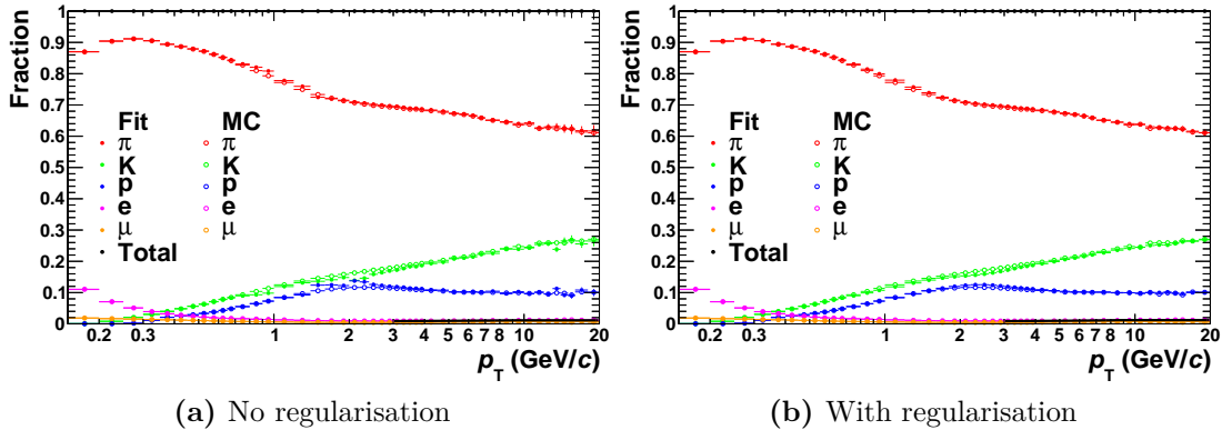
Figure 4.9.: Effect of the regularisation demonstrated for MC. The full points of the fit should be compared with the open points from the MC truth. Note that no regularisation is applied to the MC truth.
