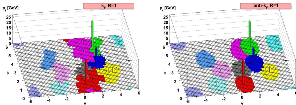
Figure 2.8.: The k_T (left) and anti- k_T (right) jet reconstruction algorithms are illustrated for a sample parton level event (generated with HERWIG [99]). By adding many random soft ghost particles, the jet areas can be determined (coloured cells). Figure from [98].
