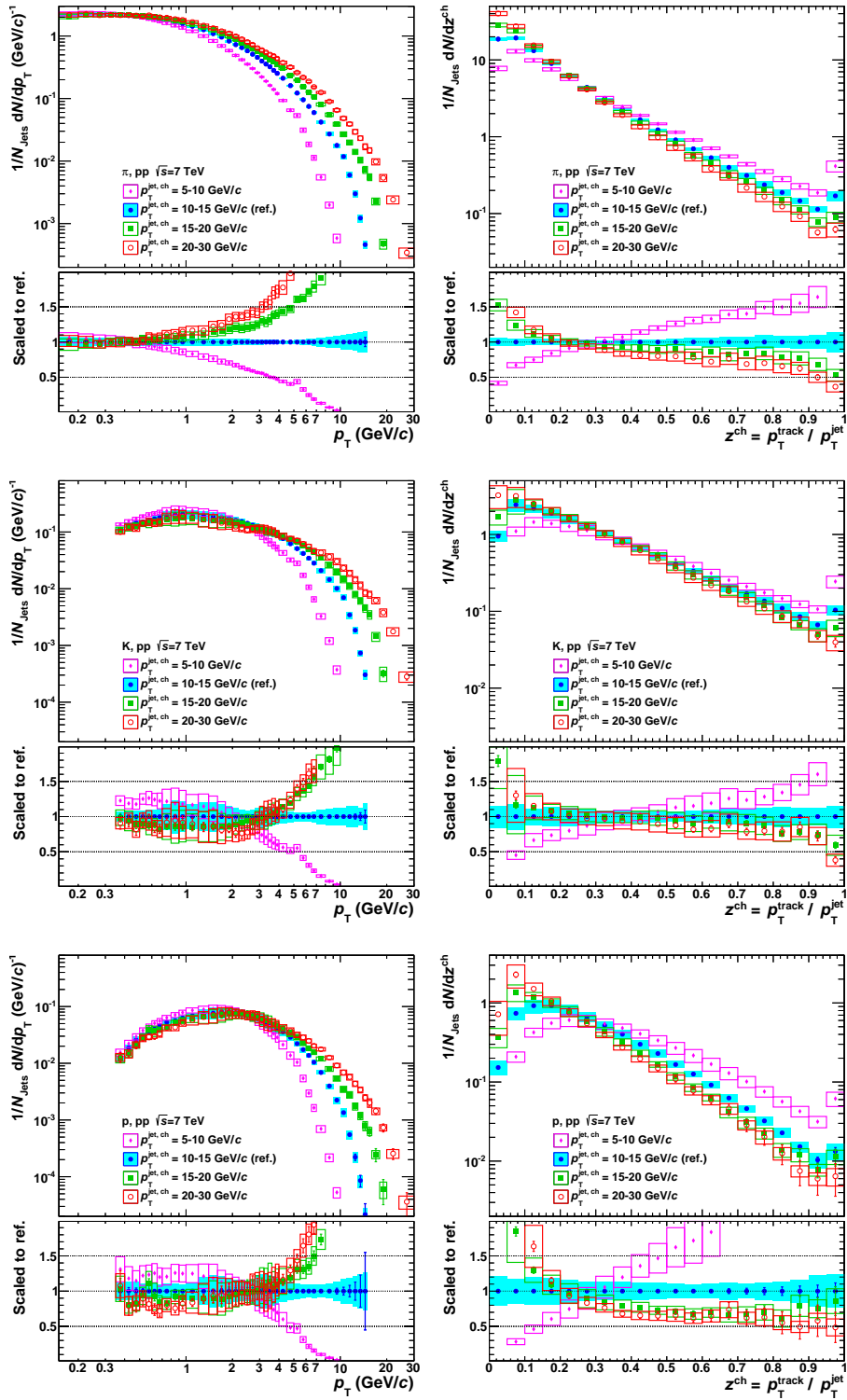
Figure 6.33.: Comparison of the corrected charged \pi/K/p yields for different p_T^{\text{jet}} in data as a function of particle p_T (left) and z (right). The rows show (from top to bottom) pions, kaons and protons.
