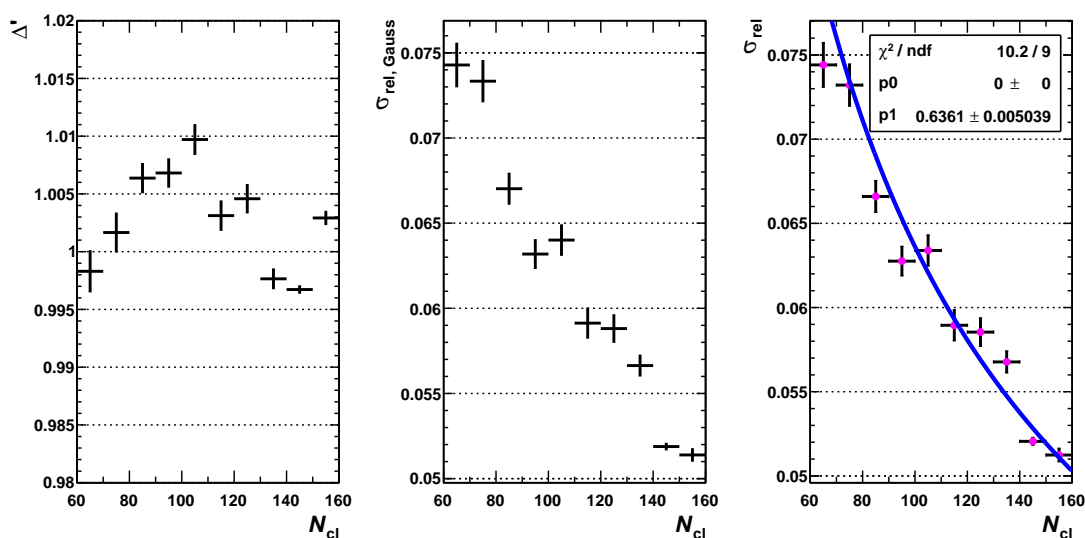
Figure 3.15.: Determination of the resolution as a function of the number of clusters.
