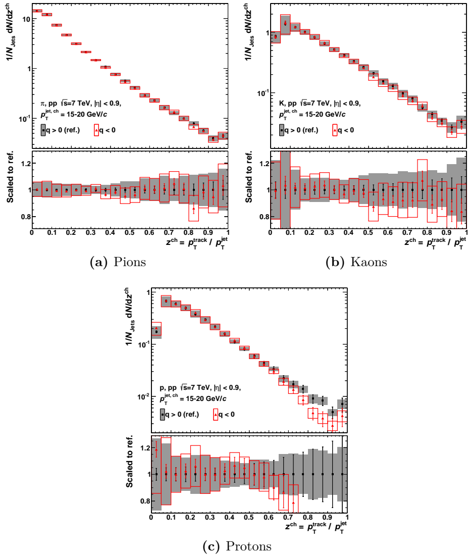
Figure J.2.: Comparison of positively ( q > 0 ) and negatively ( q < 0 ) charged particles in jets with p_T^{\text{jet}} = 15 - 20 \text{ GeV}/c . The results are shown for pions (a), kaons (b) and protons (c).
