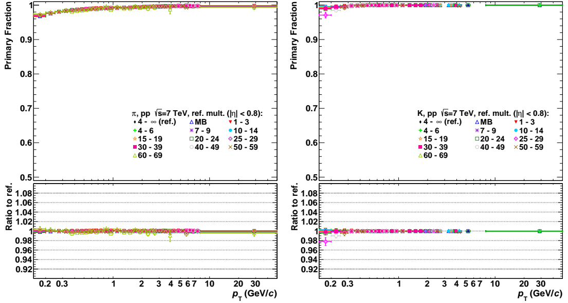
(a) Pions
