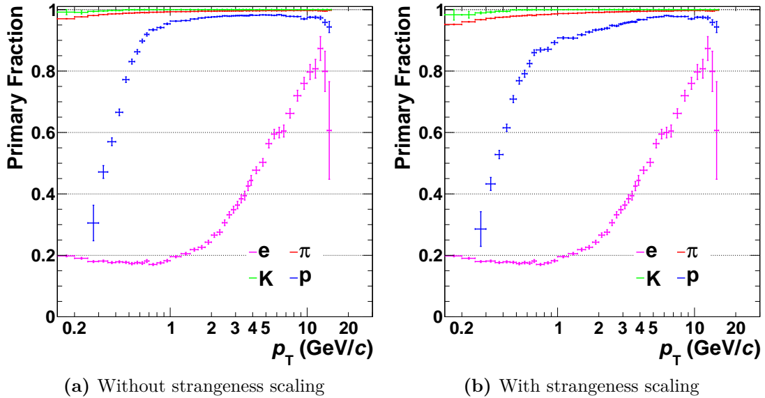
Figure 5.3.: The primary fractions for tracks in jets with p_T^{\text{jet}} = 10 - 15 GeV/c are shown as a function of p_T a) without and b) with strangeness scaling. The results are for both charges.
