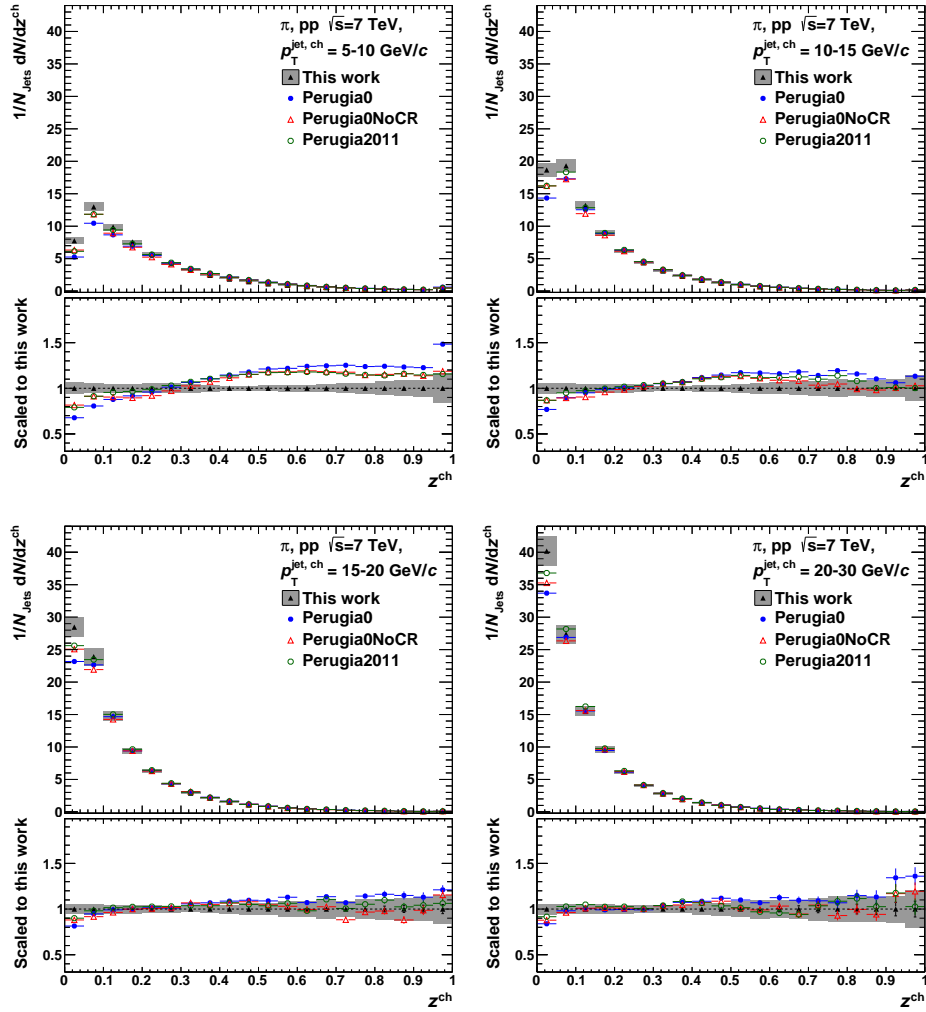
Figure K.1.: Comparison of corrected pion yields in jets to different MC predictions as a function of z . The p_T^{\text{jet}} increases from the upper left to the lower right panel.
