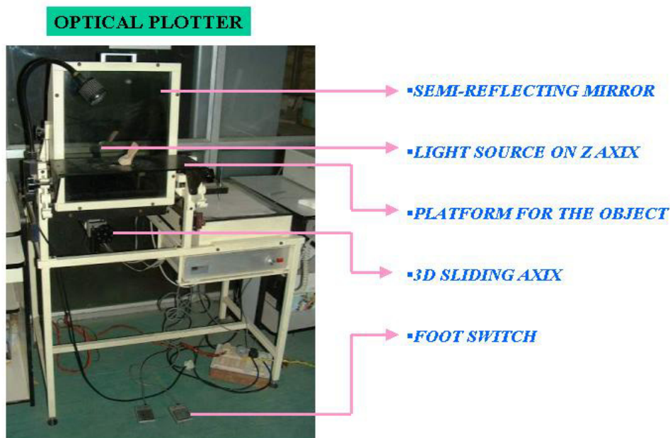
Figure 1. Optical plotter used by HNBGU.
