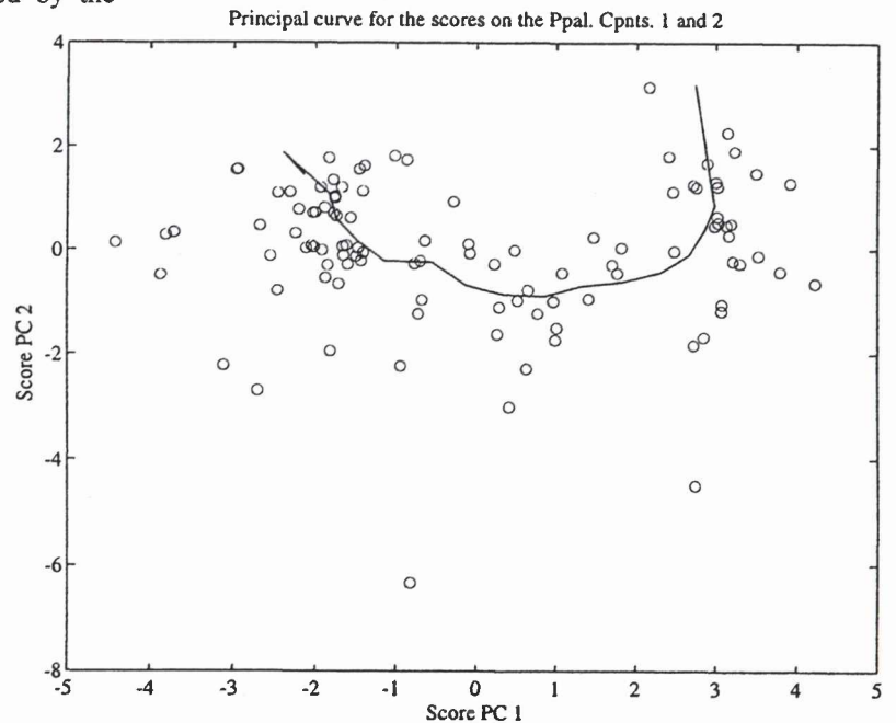
Figure 5. Example 4.2. Principal curve for Romano-British waste glass.
