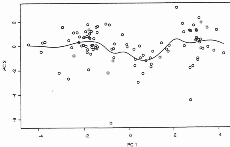
Figure 2. Example 2.1. Nonparametric regression for Romano-British waste glass.
