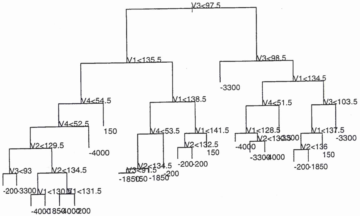
Figure 4. Example 2.3. CART for Egyptian skulls.
