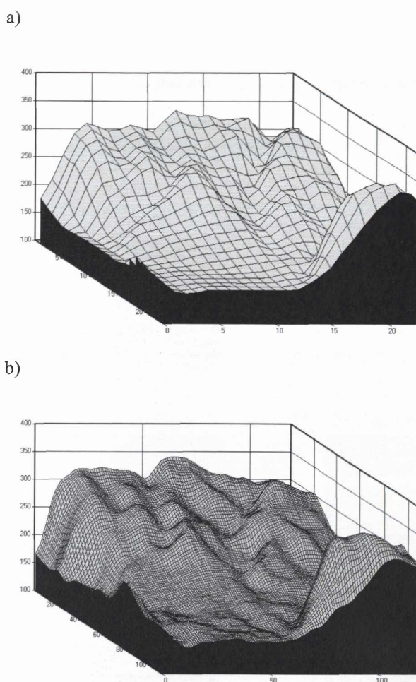
Fig. 5. Visual comparison of governmental DEM 100 (a) and interferometric InSAR DEM 25 (b). The later can be used much more effectively in applications such as archaeological modeling
