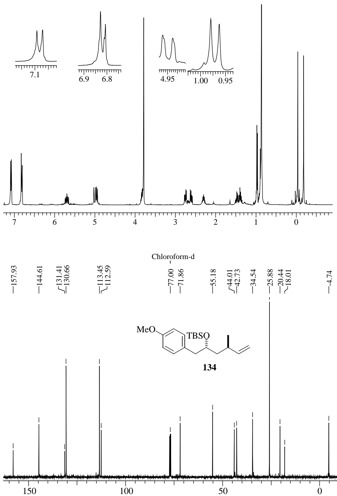
1 H- and 13 C-NMR spectra of compound 134 .
