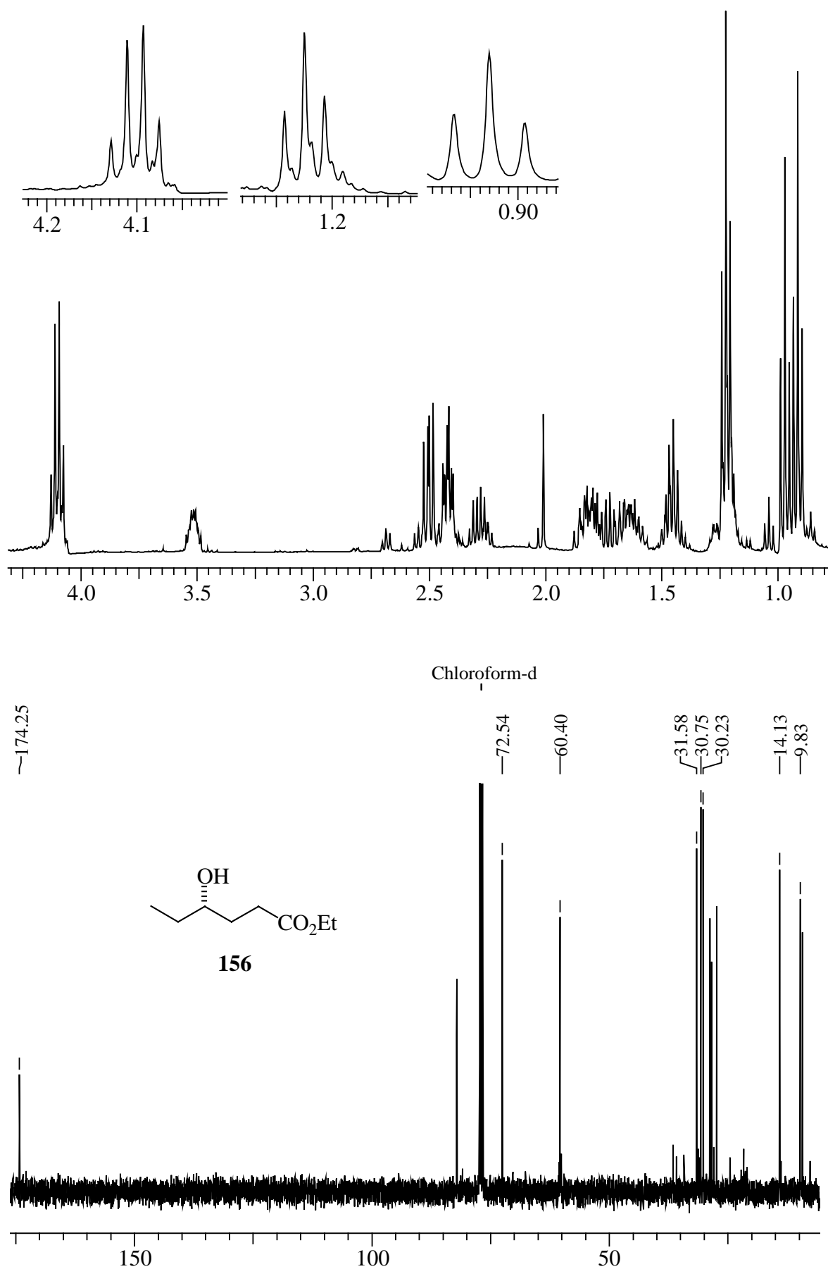
^1\text{H} - and ^{13}\text{C} -NMR spectra of compound 156 .
