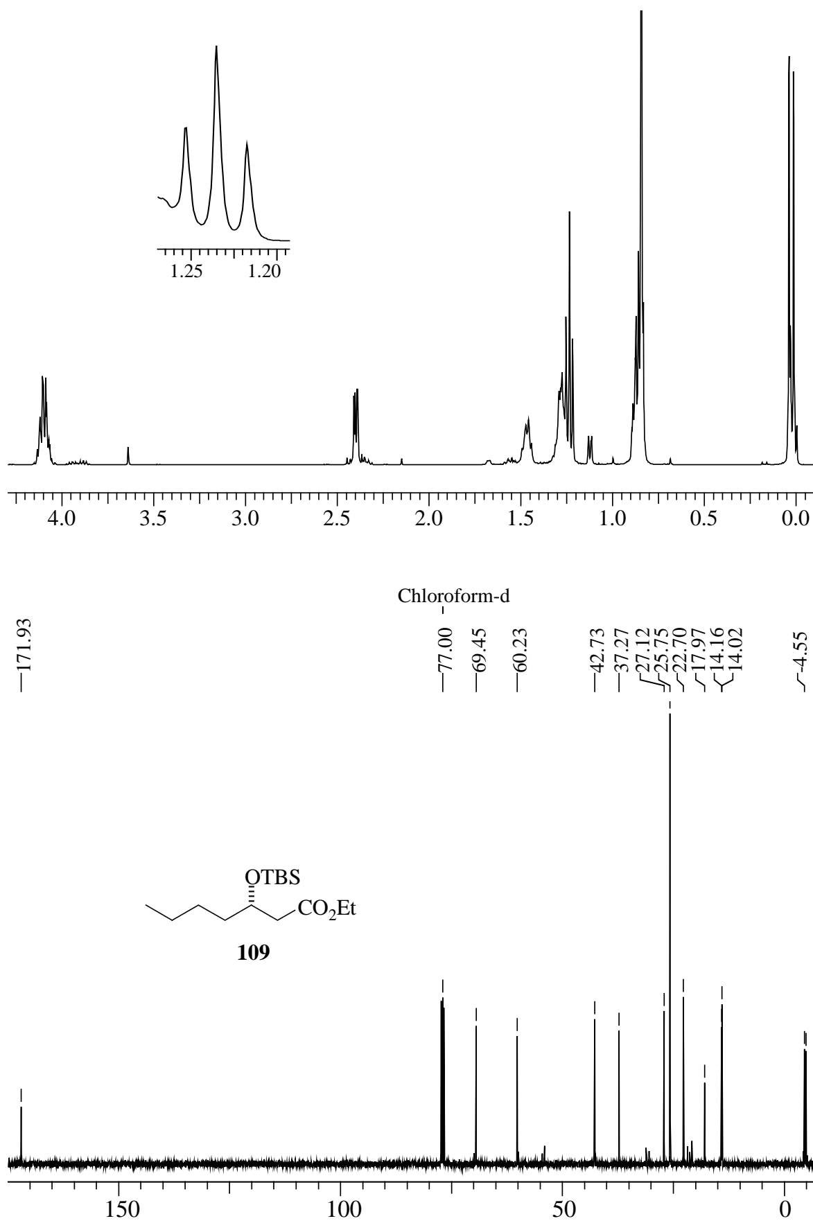
^1\text{H} - and ^{13}\text{C} -NMR spectra of compound 109 .
