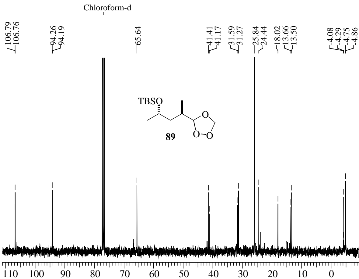
^1\text{H} - and ^{13}\text{C} -NMR spectra of compound 89 .
