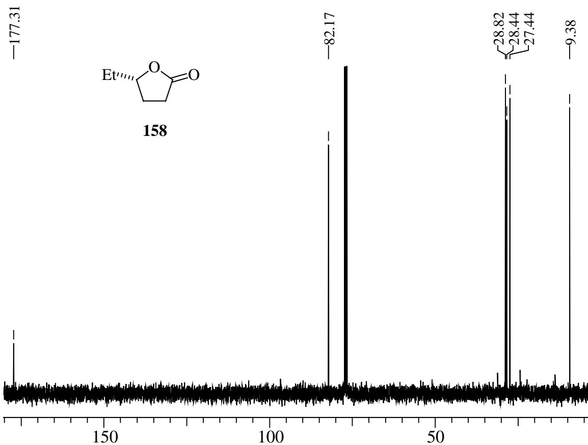
^1\text{H} - and ^{13}\text{C} -NMR spectra of compound 158 .
