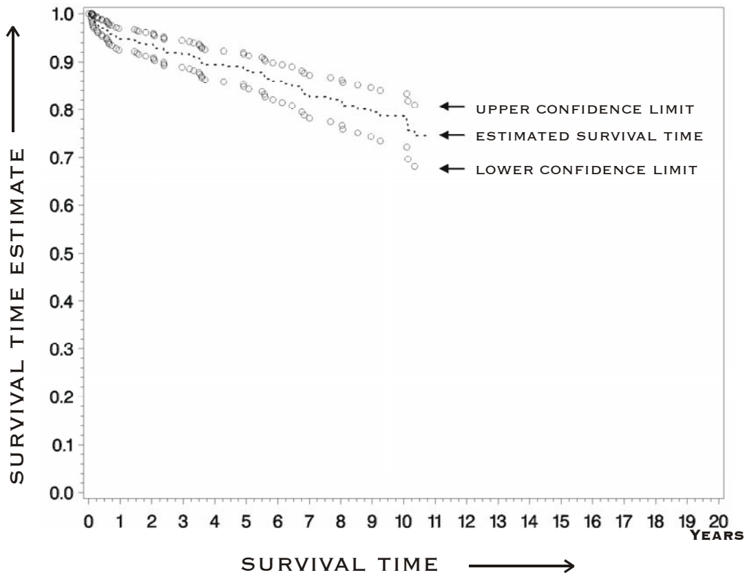
Fig. 1: Sample view of survival rate probability after Kaplan-Meier with 95% confidence interval
