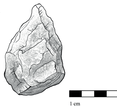
Fig. 143. Survey find AZ-14-262-PS-12. Biface made of quartzite found in the area that was dominated by Palaeolithic material south of the modern village of Azután.
