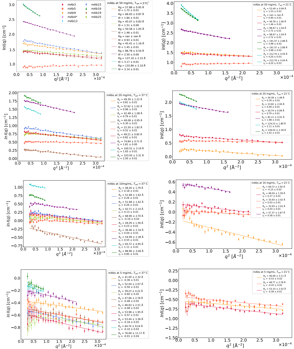
Fig. 6.14. Guinier representation, \ln(I) vs q^2 , of the SANS data (symbols) of the mAbs at different c_p (50, 20, 10, 5 mg/mL from top to bottom) and temperatures (left: 37°C; right: 21°C). Solid lines are Guinier fits to the data, from which the radius of gyration R_g and the intensity I_0 with their uncertainties were calculated (see legends). The range of the fits, or “Guinier region”, is [q_{\min}, q_{\max}] , where q_{\min} is the least value accessible by the instrument and q_{\max} is defined by q_{\max} \cdot R_g \leq 1.3 .
