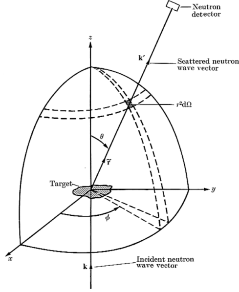
Fig. 3.1. Geometry of a neutron scattering experiment. The incoming neutron with scattering vector \vec{k} aligned along the z -axis hits the target sample. It is then scattered along the direction \vec{r} (at an angle \theta with the z -axis and an angle \phi in the (x, y) -plane) with a scattering vector \vec{k}' and falls onto the detector. The two angles \theta and \phi define the scattering geometry and determine the solid angle r^2 d\Omega . Image from Ref. [293].
