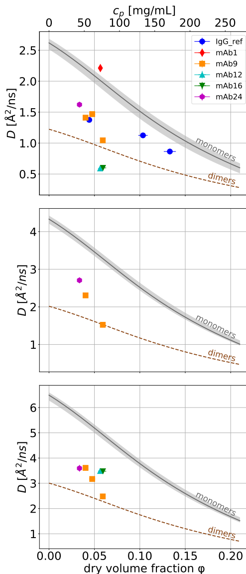
Fig. 5.5. Observable apparent diffusion coefficients D (symbols, obtained from global fits of QENS data) of the mAbs and polyclonal IgG vs protein dry volume fraction \varphi (lower) and concentration c_p (upper x-axis) in solution at T = 280 K (top), T = 295 K (center), T = 310 K (bottom). Grey solid lines denote the average value of D^{\text{theo}} for monomers of all mAbs, murine and human IgG [424], obtained using a colloid physics hard-sphere model as explained in section 5.5.4. Grey shaded areas are delimited by D^{\text{theo}} for 1IGT (lower) and mAb12 (upper limit). Dashed brown lines are the approximated dimer curves obtained by rescaling the monomer ones by the dilute limit D^{\text{theo}}(0) of the dimeric immunoglobulin structure 2QTJ [425]. Symbols below the monomer lines corroborate the presence of clusters due to their larger hydrodynamic size. However, these clusters are mainly dimers or formed by few monomers and they dissociate at increasing temperature (from approximately storage to body temperature).
