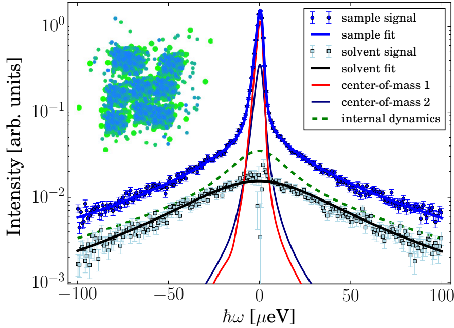
Fig. 7.3. Example spectrum recorded on BSA at c_p = 240 mg/ml in D 2 O with c_s = 27 mM LaCl 3 , at T = 310 K and q = 0.55 Å -1 (upper circle symbols). The lower square symbols denote the corresponding pure D 2 O solvent spectrum scaled by (1 - \varphi) . In both spectra the container contribution was subtracted. The thick solid lines superimposed on the spectra are fits to the data. The narrow solid lines represent the Lorentzians accounting for the two separate global center-of-mass diffusion coefficients attributed to the dense and dilute phase, respectively, subsequent to the convolution with the resolution function, explaining the peculiar shape of the narrowest Lorentzian. The dashed line represents the sum of the internal diffusion of the two phases, Equation 7.3. The inset artistic schematic illustrates the cluster distributions in the LLPS regime with local dense and dilute regions described by the Flory-Stockmayer model (cf. main text).
