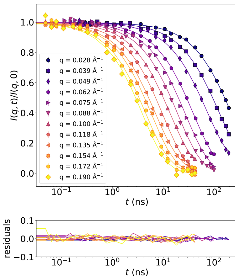
Fig. 6.4. Intermediate scattering function I(q, t)/I(q, 0) (neutron echoes vs Fourier time t ) of mAb5 at c_p = 50 \text{ mg/mL} and T = 37^\circ\text{C} , in solution with 20 mM His-HCl buffer at pD 6.4, measured with IN15 spectrometer. The experimental points obtained are the combination of the four different instrument configurations used (wavelength of incident neutron and detector angle). Each data series, denoted by a specific symbol and colour, corresponds to the neutron echo at a specific value of the momentum transfer q , ranging from 0.028 (dark purple dots) to 0.19 \text{ Å}^{-1} (yellow diamonds). Solid lines in corresponding colours are fits to the data with a cumulant expansion of the exponential (Equation 6.4) using all Fourier times. Data are presented in lin-log scale (top) with the corresponding fit residuals at each q depicted with the same color code (bottom).
