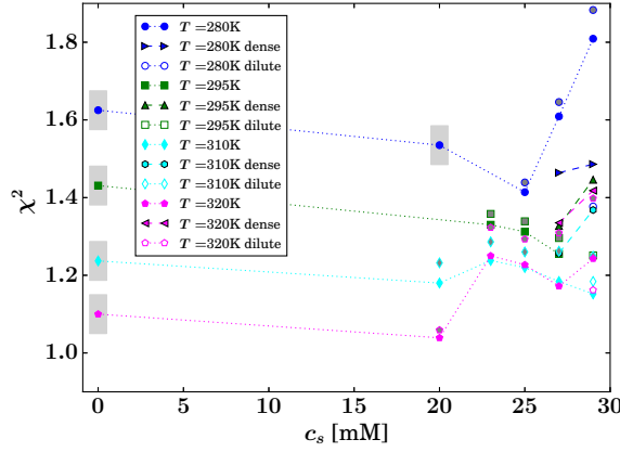
Fig. 7.19. Summary of the goodness-of-fit \chi^2 obtained from the global fits for all samples. For the dense and dilute phases separated by a centrifuge (marked as “dense” and “dilute”, respectively, in the legend) as well as for the samples marked by a grey shaded area under the respective symbol, only one center-of-mass diffusion coefficient was permitted in the fit. For the fits where two center-of-mass diffusion coefficients were employed, \chi^2 for the alternative situation of one center-of-mass diffusion coefficient is in addition displayed by the corresponding grey-filled symbols with identical shape and edge color, that are always located above the associated fit with two center-of-mass diffusion coefficients. All spectra were acquired with the same integral incident neutron flux on the sample. Therefore, the systematic temperature-dependence of this error-weighted \chi^2 can be attributed to the higher total spectral signal at lower T , and, thus, lower statistical error.
